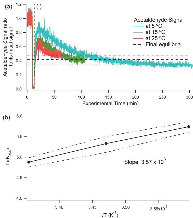
Fig. 7. Typical acetaldehyde time profiles at 5, 15 and 25 °C are shown in (a). The ratios of signal at a given time to the initial signal are shown. H_2O_2 (13.3 mM) was injected to the 10 mM acetaldehyde solutions at time (i). The dashed lines show the signal levels at equilibrium. The van't Hoff diagram for 1-hydroxyethyl hydroperoxide (1-HEHP) formation from acetaldehyde is shown in (b). The dashed lines connects +1\sigma and -1\sigma from the average \ln(K_{app}) determined at the three temperatures.
