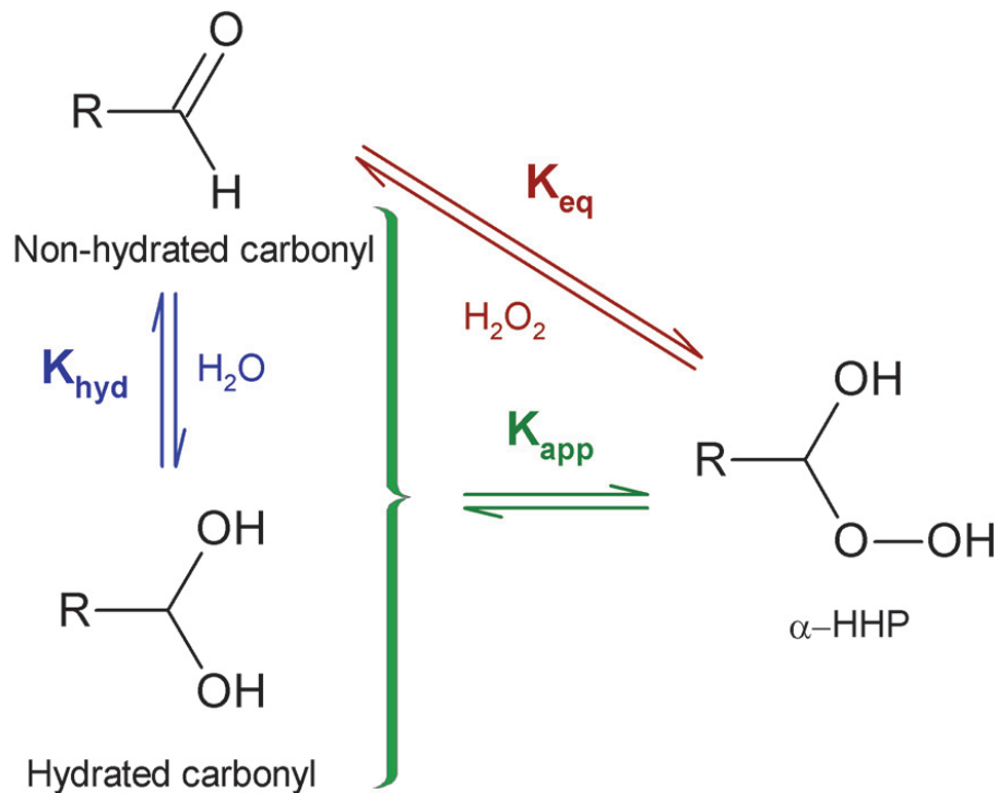
Fig. 4. Hydration equilibrium constant ( K_{\text{hyd}} ), the \alpha -HHP formation equilibrium constant ( K_{\text{eq}} ) and the apparent \alpha -HHP formation equilibrium constant ( K_{\text{app}} ). Please see the text for details.
