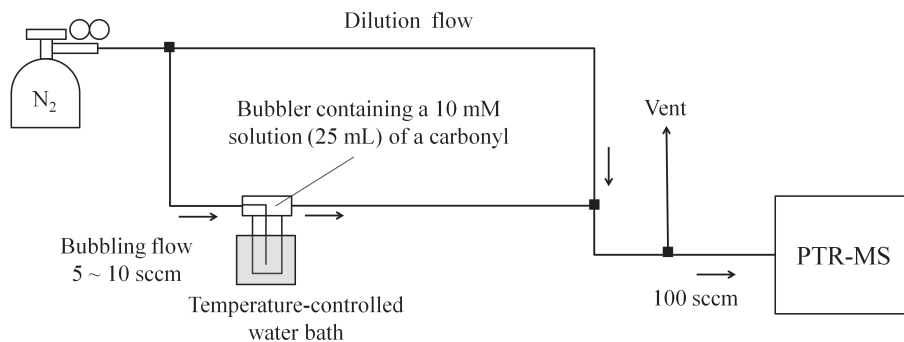
Fig. 2. Experimental setup for the PTR-MS measurements.
