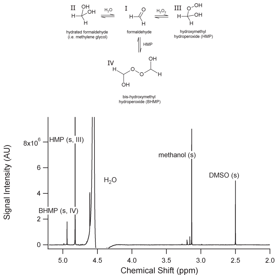
Fig. 6. 1 H NMR spectra of a formaldehyde-H 2 O 2 mixture. The splitting pattern and assignment of the peaks are shown in the bracket.
