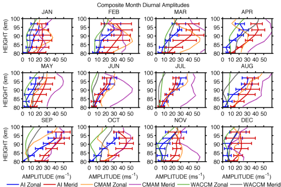
Fig. 7. Amplitudes of the diurnal tide as a function of month and height. The error bars on the radar observations (blue and red lines for zonal and meridional components, respectively) indicate the standard deviation of the individual monthly means over the interval 2002–2011.
