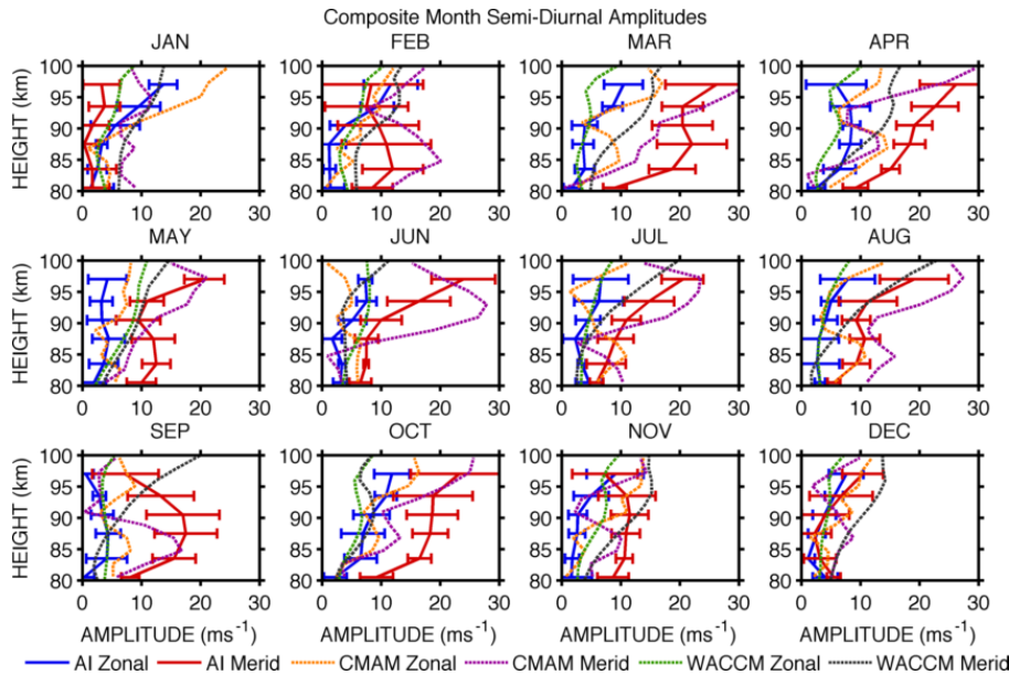
Fig. 10. Amplitudes of the semidiurnal tide as a function of month and height. The error bars on the radar observations (blue and red lines for zonal and meridional components, respectively) indicate the standard deviation of the individual monthly means over the interval 2002–2011.
