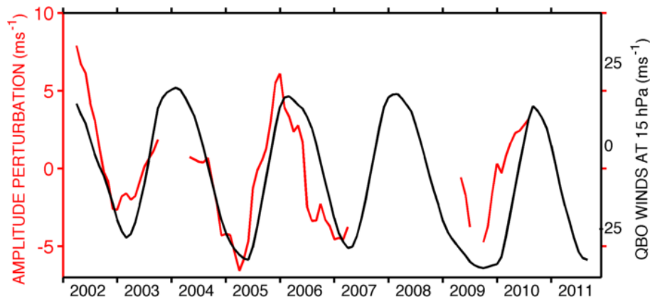
Fig. 13. Perturbations in meridional diurnal tide amplitudes (calculated by subtracting the composite-year monthly mean from each individual month) at heights near 84 km (red line) for 2002–2011. Also plotted are the QBO background winds at 15 hPa (black line). The diurnal-tidal amplitude perturbations and background winds are smoothed with a seven-month running mean. Note the two different axes, with the red axis on the left corresponding to the diurnal amplitude perturbations and the black axis on the right corresponding to the QBO line. Correlation between the amplitude perturbations and the background QBO winds can be clearly seen.
