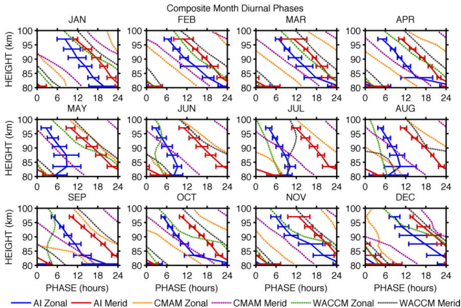
Fig. 8. Phases of the diurnal tide as a function of month and height. The error bars on the radar observations (blue and red lines for zonal and meridional components, respectively) indicate the standard deviation of the individual monthly means over the interval 2002–2011.
