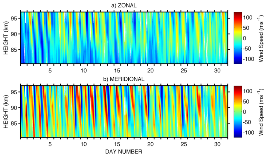
Fig. 3. Zonal (a) and meridional (b) winds as a function of height and time as recorded by the Ascension Island meteor radar in March 2009. The large-amplitude diurnal tide can clearly be seen in both wind components.
