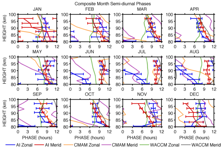
Fig. 11. Phases of the semidiurnal tide as a function of month and height. The error bars on the radar observations (blue and red lines for zonal and meridional components, respectively) indicate the standard deviation of the individual monthly means over the interval 2002–2011.
