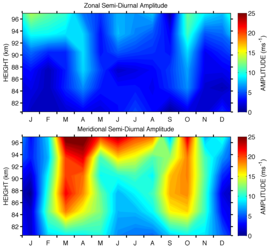
Fig. 9. Composite-year monthly-mean semidiurnal tidal amplitudes as a function of month and height over Ascension Island for all data recorded from January 2002 to June 2011.
