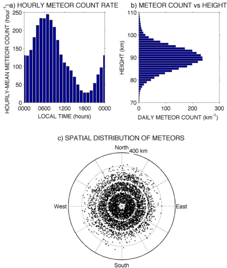
Fig. 1. (a) The diurnal cycle of meteor counts detected by the Ascension Island meteor radar (calculated from the ~200 000 meteors detected in 2005). (b) The vertical profile of these meteor counts as a function of height, presented as meteor counts per km. (c) The distribution of meteors detected on 22 July 2005 projected onto a horizontal plane.
