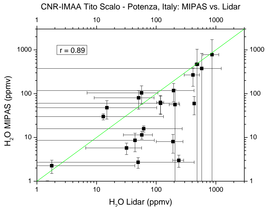
Fig. 19. Correlation between H 2 O mixing ratios measured by MIPAS and 12 lidar soundings performed by the CNR-IMAA in Potenza between July 2002 and February 2004. Green line denotes the 1 : 1 diagonal. A correlation coefficient r is calculated for all data points.
