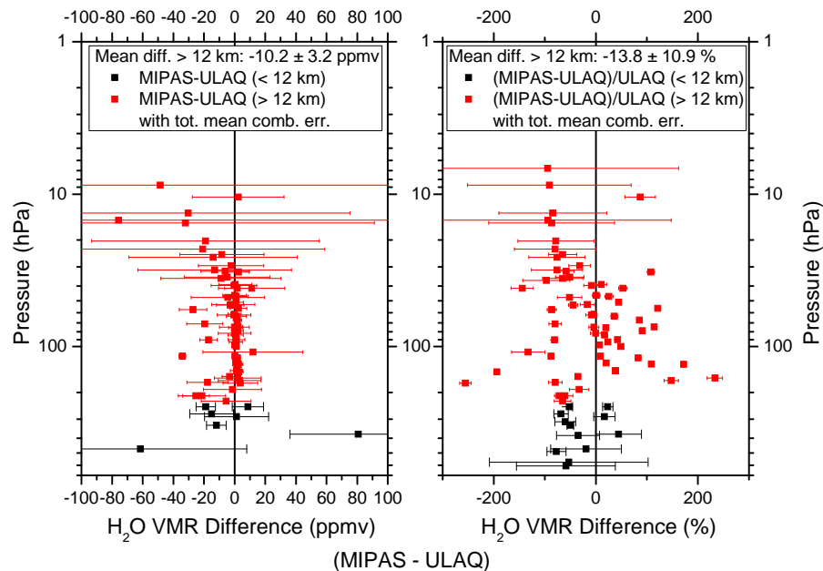
Fig. 18. Differences between H 2 O profiles measured by MIPAS and thirteen radio soundings of the University of L'Aquila, performed in winter/spring 2002 and 2004, together with combined total errors, plotted as error bars. Black squares: differences below 12 km; red squares: differences above 12 km.
