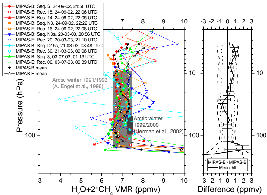
Fig. 3. Hydrogen budget of all comparisons between MIPAS-E and MIPAS-B together with absolute differences and combined precision (dotted lines) and total (dashed lines) errors. For comparison, Arctic winter balloon-borne observations (solid grey bar) performed by Engel et al. (1996) and aircraft measurements (solid dark grey bar) carried out by Herman et al. (2002) are shown, too.
