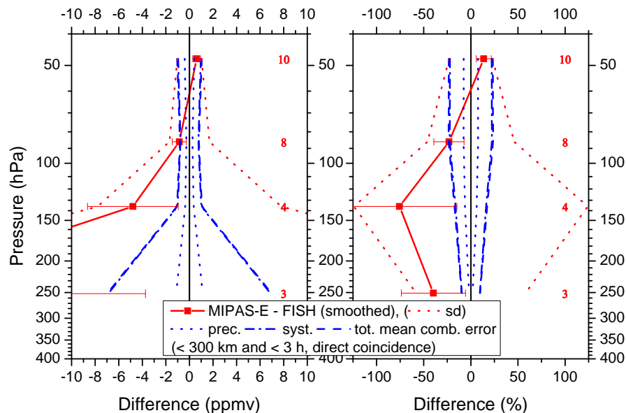
Fig. 8. Absolute (left) and relative (right) differences (red squared lines) between MIPAS-E and the stratospheric hygrometer FISH for all Geophysica flights carried out above Italy and northern Sweden within a direct coincidence limit of 300 km and 3 h together with mean combined precision (blue dotted lines), systematic (blue dash-dotted lines), and total errors (blue dashed lines) as well as standard deviation (red dotted lines) and the standard error of the mean, plotted as error bars. FISH profiles were smoothed with the averaging kernel of MIPAS-E. Red values indicate the number of collocations.
