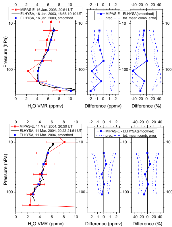
Fig. 4. Comparison between MIPAS-E (red squared line) and ELHYSA (black solid line) measured H 2 O profiles from 16 January 2003 (top) and 11 March 2004 (bottom) at Kiruna (~68° N) along with absolute and relative differences (blue squared lines) and combined errors (blue dotted and dashed lines). The in-situ ELHYSA profile was smoothed with the averaging kernel of MIPAS-E (blue squared line) to make the vertical resolution of both instruments comparable.
