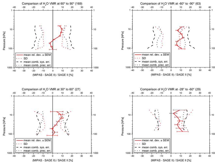
Fig. 15. Mean relative deviation (including the standard error of the mean) of H 2 O profiles as measured by MIPAS and SAGE II in the Northern (left) and Southern (right) Hemisphere for different latitude regions. Annotation as per Fig. 13.
