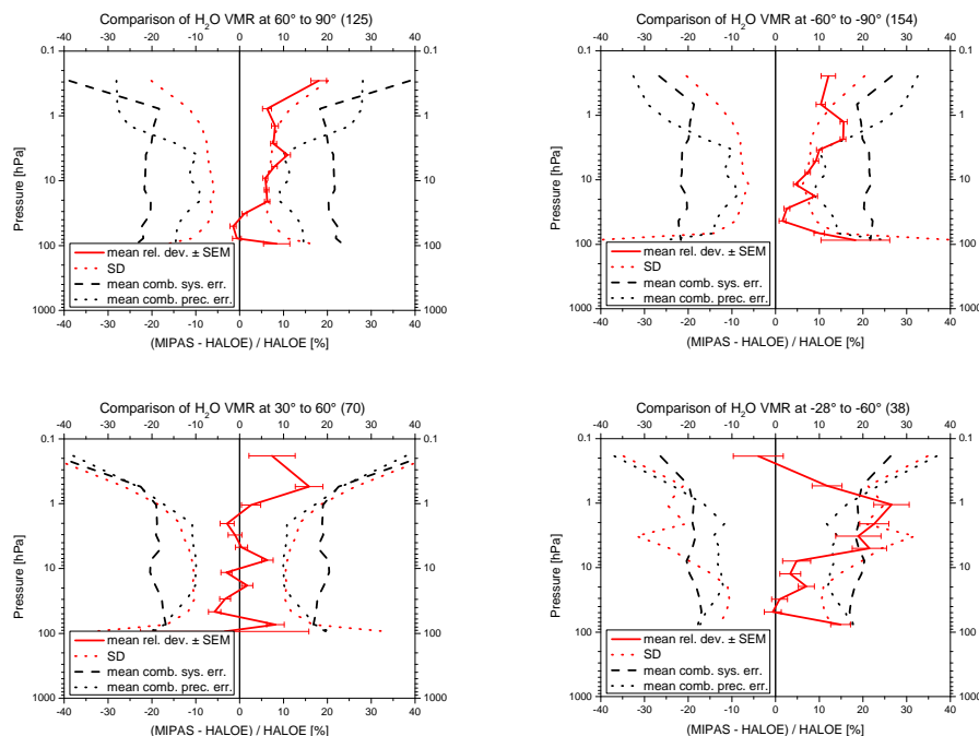
Fig. 13. Mean relative deviation (including the standard error of the mean) of H 2 O profiles as measured by MIPAS and HALOE in the Northern (left) and Southern (right) Hemisphere for different latitude regions (red solid lines). Standard deviation (red dotted lines) and mean combined precision (black dotted lines) and systematic errors (black dashed lines) are plotted, too.
