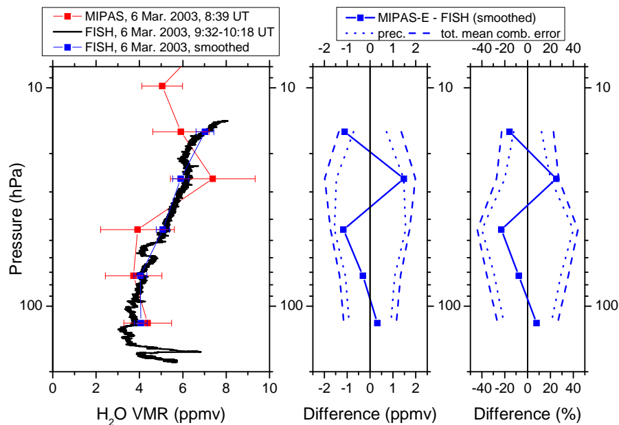
Fig. 5. Direct comparison of H 2 O profiles measured by MIPAS-E and the balloon-borne in-situ instrument FISH on 6 March 2003 at Kiruna (~68°N) along with absolute and relative differences and combined errors. The in-situ FISH profile was smoothed with the averaging kernel of MIPAS-E to make the vertical resolution of both instruments comparable. Annotation as per Fig. 4.
