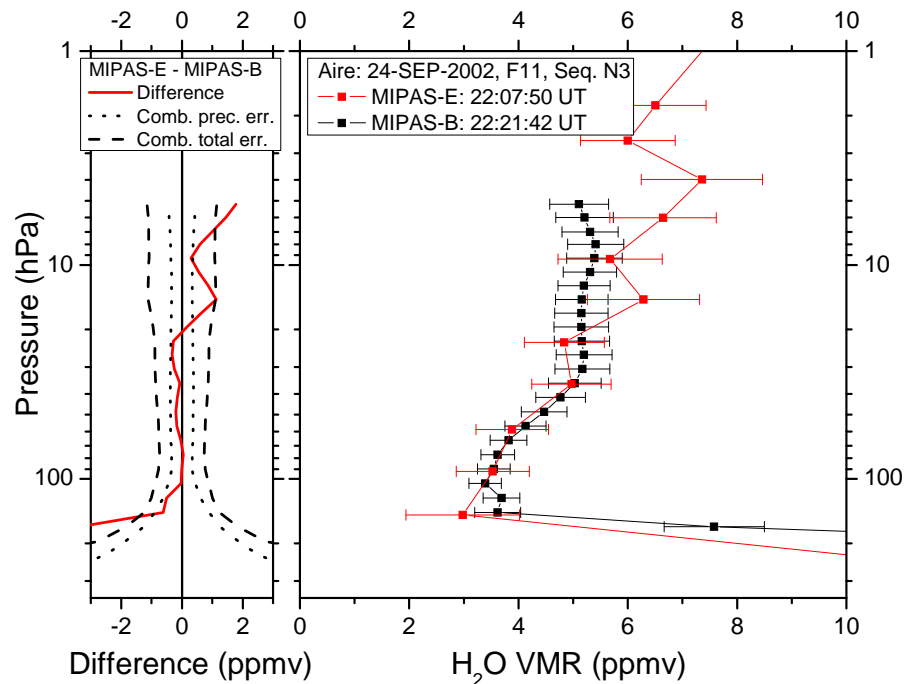
Fig. 1. Comparison of H 2 O profiles measured by MIPAS-B (flight no. 11, sequence N3, black squared line) and MIPAS-E (orbit 2975, red squared line) on 24 September 2002 above southern France along with difference (red solid line) and 1 \sigma combined precision (black dotted lines) and total errors (black dashed lines).
