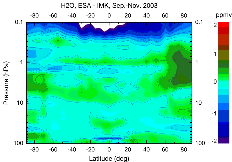
Fig. 20. Difference of global zonally averaged H 2 O VMR distributions in the 100 hPa to 0.1 hPa altitude range as retrieved by the ESA and IMK/IAA processors for the September to November 2003 period. Deviations are mostly within 0.25 ppmv (or about 10%) except of the Arctic upper stratosphere and towards the upper boundary of the MIPAS measurement range. Reddish colours denote positive and bluish colours negative deviations.
