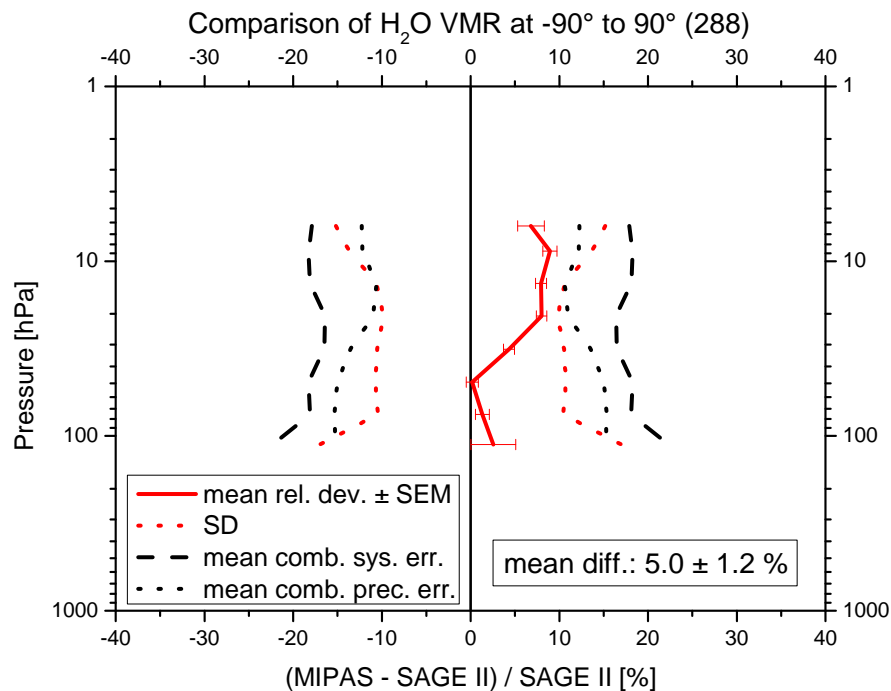
Fig. 16. Mean relative deviation of H 2 O profiles as measured by MIPAS and SAGE II for all collocations (288). Annotation as per Fig. 13.
