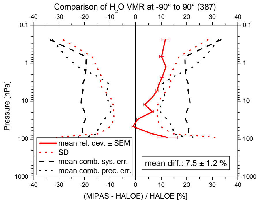
Fig. 14. Mean relative deviation of H 2 O profiles as measured by MIPAS and HALOE for all collocations (387). Annotation as per Fig. 13.
