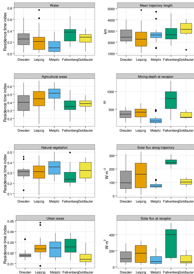
Fig. 2. Box-plots of residence time indices and further parameters of back trajectory analysis at different sampling sites. Bold line represents median, boxes lower and upper quartiles, whiskers 1.5 times the interquartile range, and dots indicate values outside this range.
