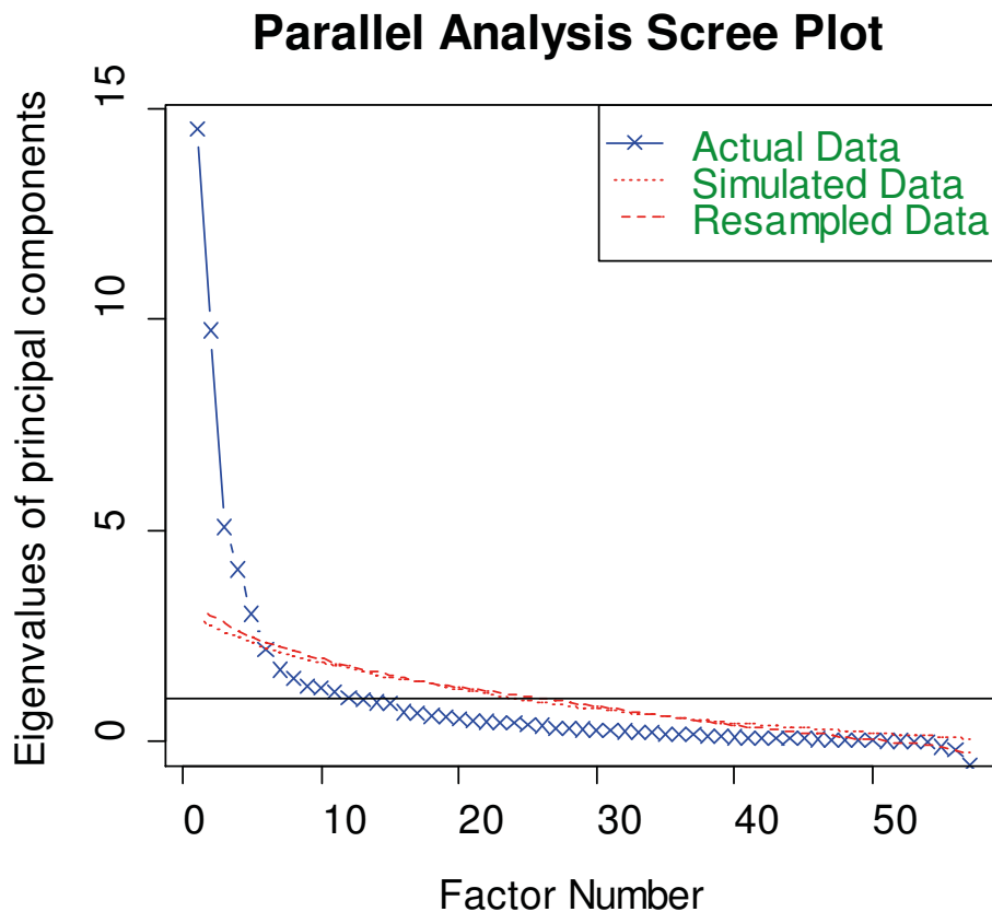
Fig. 3. Screen plot of PCA including results from parallel analysis.
