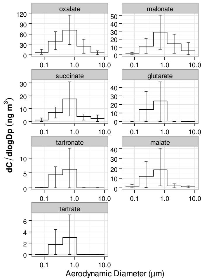
Fig. 1. Mean size distributions of DCAs at all sites. Error bars indicate the 15th and 85th percentiles as a measure of data variability.
