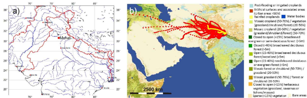
Fig. 2. (a) Location of the city of Mohali in the north west Indo-Gangetic plain ( 30.667^{\circ} N, 76.729^{\circ} E, 310 ma.s.l.) (b) 72 h back trajectories of air masses that arrived at the site (site shown as black marker) everyday from 1 May 2012–31 May 2012 at 14:30 LT (UTC + 05:30) superimposed on a land classification map (courtesy ESA GlobCover 2009 Project).
