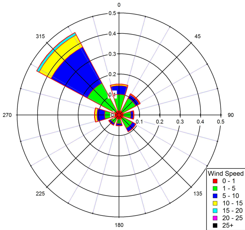
Fig. 4. Wind rose plot derived from in-situ one minute wind direction and wind speed data at the measurement site ( 30.667^\circ N, 76.729^\circ E, 310 ma.s.l.) in May 2012.
