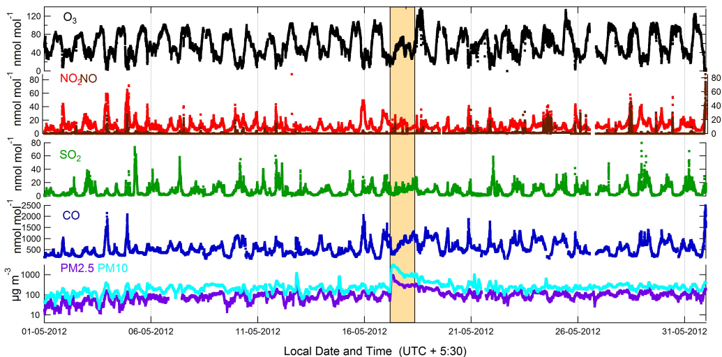
Fig. 7. Time series of the one minute data in May 2012 for the mixing ratios of ozone (top panel), \text{NO}_2 (refer to Section 2.2.3 for details of the \text{NO}_x measurements) and NO (second panel), \text{SO}_2 (third panel), CO (fourth panel) and mass concentrations of \text{PM}_{2.5} and \text{PM}_{10} (bottom panel).
