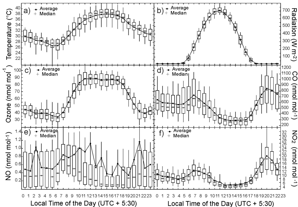
Fig. 9. Diel box and whisker plot of (a) the ambient temperature, (b) radiation, (c) ozone, (d) carbon monoxide, (e) nitrogen monoxide and (f) nitrogen dioxide (refer to Section 2.2.3 for details of the NO x measurements) derived from all measurements ( n > 14300 for each species) in May 2012 at the measurement site.
