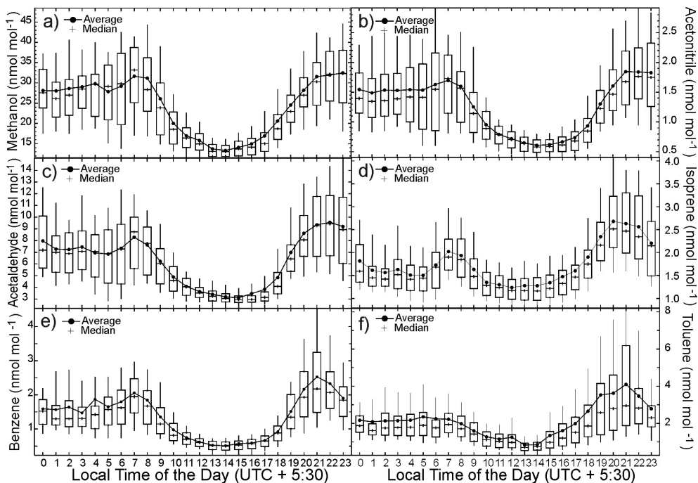
Fig. 10. Diel box and whisker plot of (a) methanol, (b) acetonitrile, (c) acetaldehyde, (d) isoprene, (e) benzene and (f) toluene derived from all measurements ( n > 14300 for each species) in May 2012 at the measurement site.
