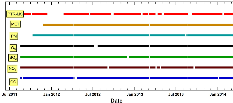
Fig. 1. Status of analyzers and availability of data from IISER Mohali ambient air quality station.
