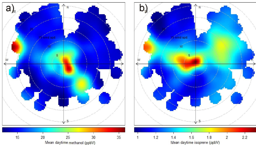
Fig. 8. Bivariate polar plots of the (a) daytime methanol data and (b) daytime isoprene data used for constraining location of major point emission sources.
