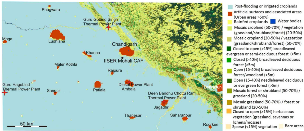
Fig. 3. Map of the land classification (courtesy ESA GlobCover 2009 Project) in a 100\text{km} \times 200\text{km} area surrounding the measurement site (black dot).
