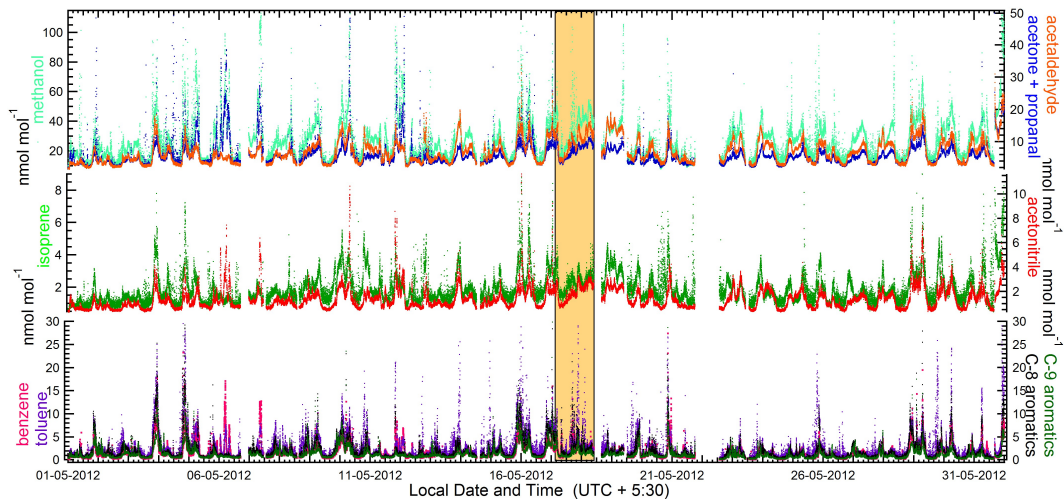
Fig. 6. Time series of the one minute data in May 2012 for the mixing ratios of methanol, acetaldehyde, sum of acetone and propanal (top panel), isoprene and acetonitrile (middle panel) and benzene, toluene, sum of C8-aromatics (xylene isomers and ethyl benzene), sum of C9-aromatics (isomers of trimethyl benzenes and propyl benzenes) (bottom panel).
