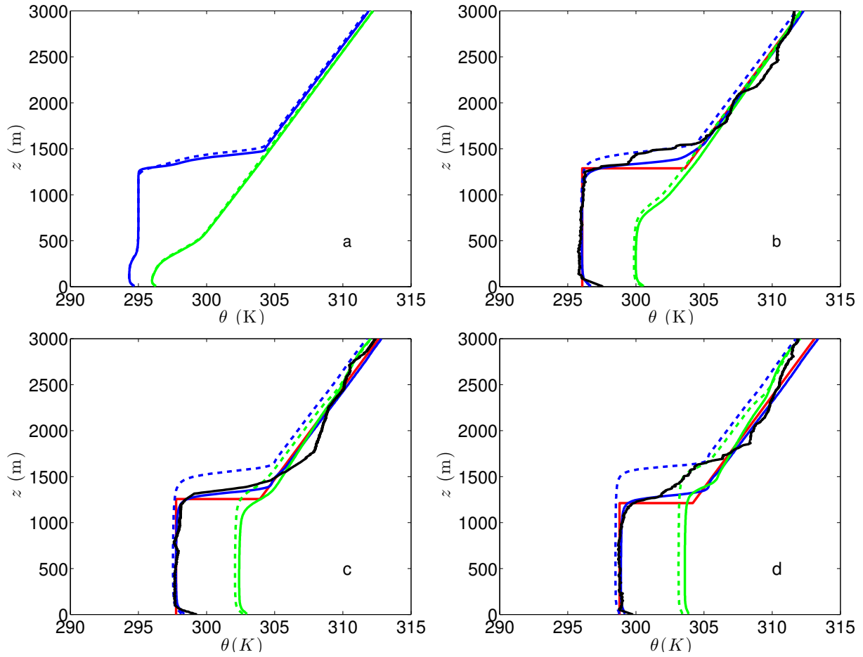
Fig. 3. Vertical profile of the 30-minutes averaged potential temperature at (a) 08:30, (b) 11:00, (c) 14:00 and (d) 17:00 UTC on 1 July 2011 observed by the radio soundings (solid black) and obtained by MLM (solid red) and DALES runs (RLs, solid blue; RLns, dash blue; nRLs, solid green; and nRLns, dash green line).
