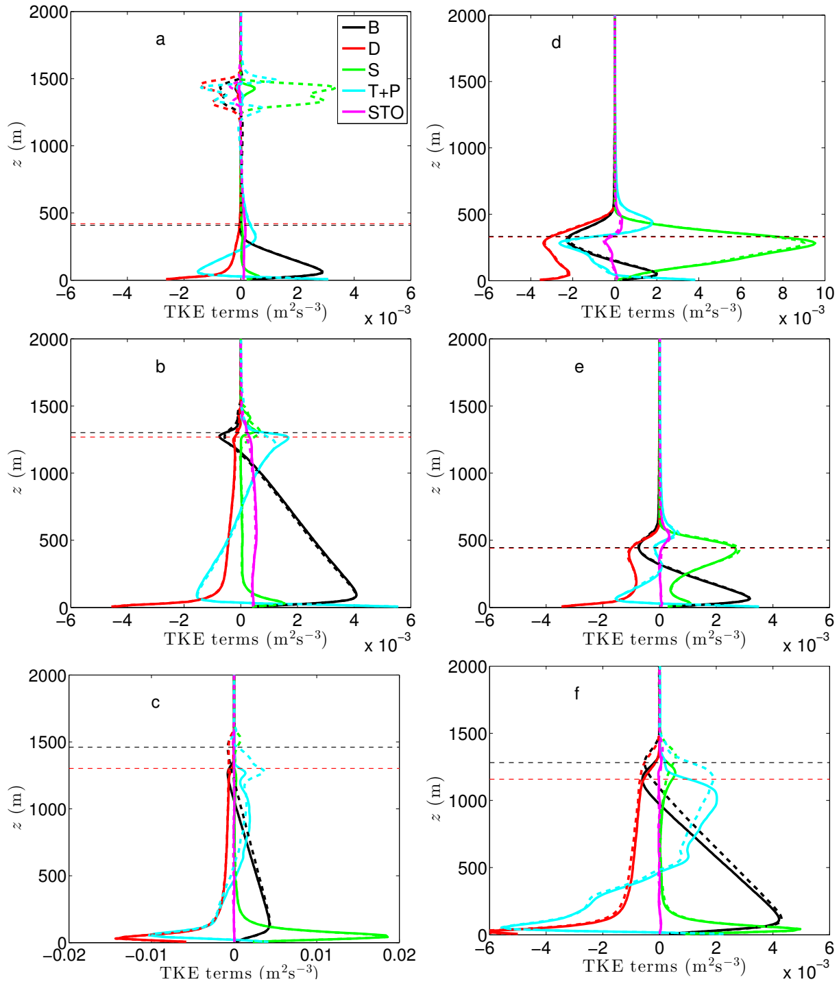
Fig. 7. Vertical profiles of the 30-minutes averaged TKE-terms for the (left) RLns (solid lines) and RLs (dashed lines) and (right) nRLns (solid lines) and nRLns (dashed lines) numerical experiments at (top) 08:30, (middle) 09:00 and (bottom) 14:00 UTC. Buoyancy production (black line), dissipation (red line), shear production (green line), turbulent transport and pressure (cyan line) and storage (magenta line) are shown. Red and black horizontal dashed lines mark for the subsidence and no-subsidence cases z_1 averaged every 30 min.
