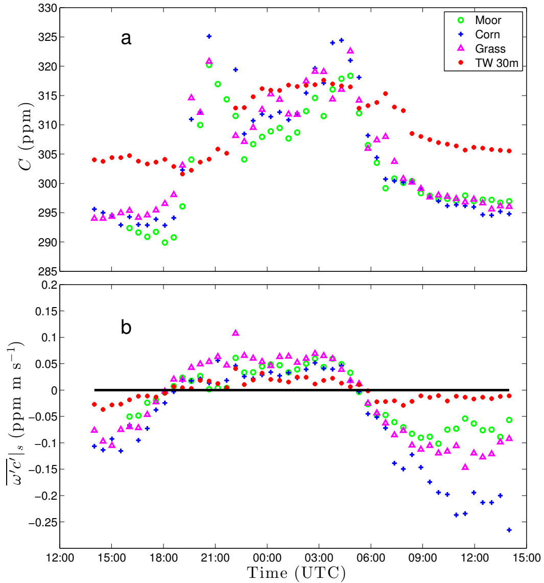
Fig. 9. Temporal evolution from 30 June 2011 at 14:00 UTC to 1 July 2011 at 14:00 UTC of the observed (a) CO 2 mixing ratio and (b) CO 2 surface flux measured at 2-m over moor (green circles), over corn (blue crosses), over long grass (magenta triangles) and at 30-m over grass (red asterisks).
