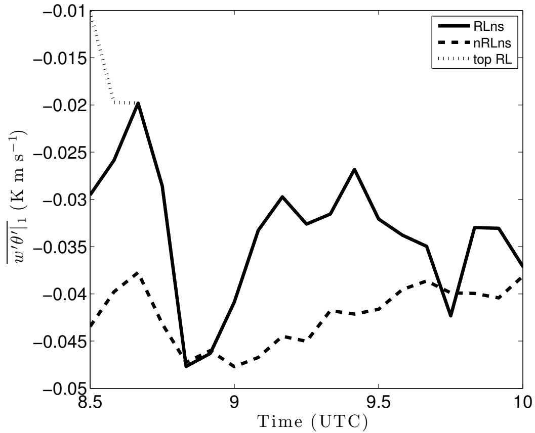
Fig. 6. Temporal evolution during the morning of the entrainment heat flux for the RLns (solid line), the entrainment heat flux at the top of the RL (pointed line), nRLns (dashed line) DALES numerical experiments.
