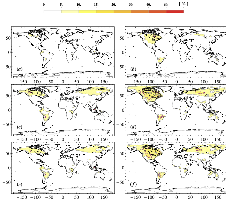
Fig. 6. Estimated percent uncertainty on N_d due to a \pm 50\% uncertainty in the hygroscopicity parameter of SOA for: (a) ARG \alpha -PD, (b) ARG \alpha -Pla, (c) FN-PD, (d) FN-Pla, (e) FN-IL-PD, (f) FN-IL-Pla.
