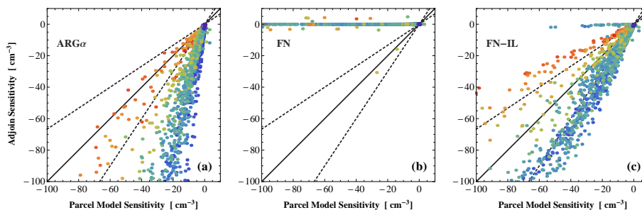
Fig. 7. Comparison between the sensitivity to hygroscopicity for coarse mode aerosol, \partial N_d / \partial \kappa_{a_i} ( \text{cm}^{-3} ), computed with detailed parcel model simulations and: (a) ARG \alpha , (b) FN, (c) FN-IL.
