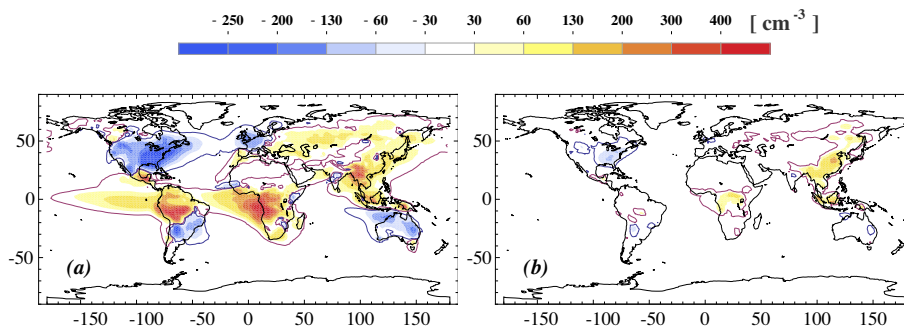
Fig. 5. Estimated contribution to changes in N_d (in \text{cm}^{-3} ) due mass change of POM aerosol. (a) Due to changes associated with the number concentration alone. (b) Changes attributable to mass (volume) associated with POM aerosol. Results shown here are for the ARG \alpha parameterization.
