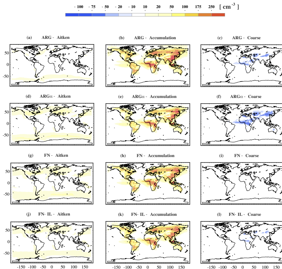
Fig. 3. Same as Fig. 2 but for aerosol hygroscopicity \partial N_d / \partial \kappa_a (in \text{cm}^{-3} ).
