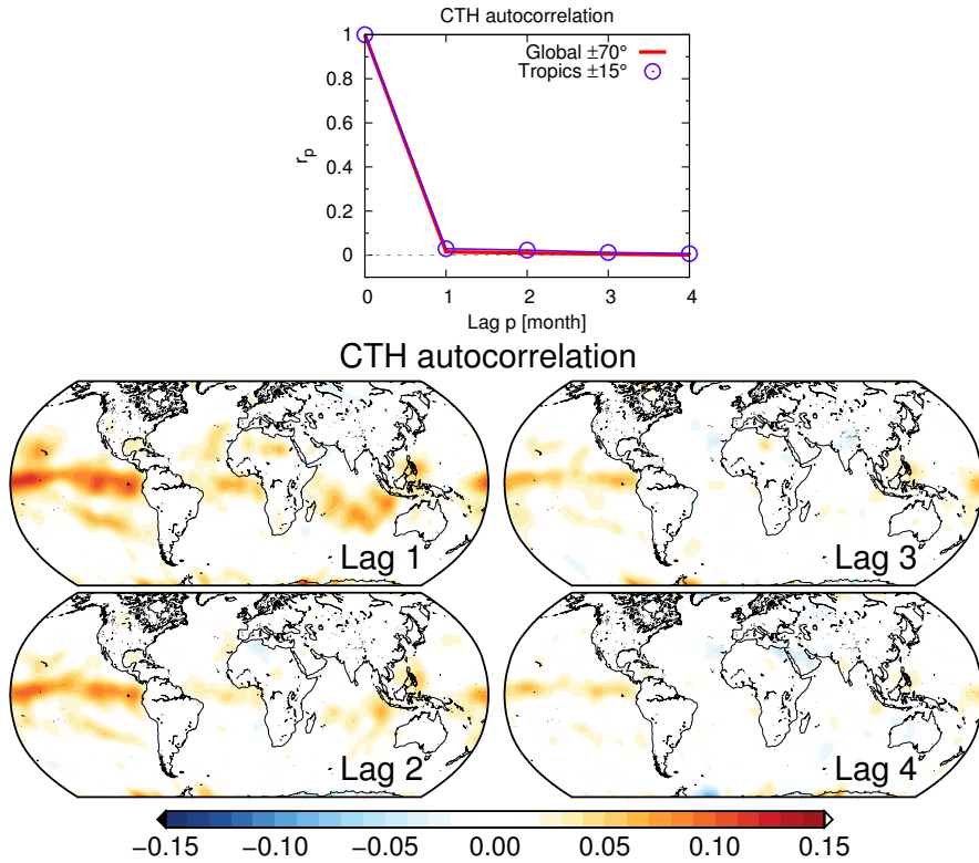
Fig. 4. (Upper plot) Autocorrelation function of cloud top height anomalies. Unlagged data ( p = 0 ) correlate perfectly with themselves ( r_0 = 1 ). r_p decays to almost 0 already at p = 1 . (Lower plot) Maps of CTH autocorrelation for the first 4 months. ENSO-related patterns are seen over Pacific, Indian and Atlantic Oceans.
