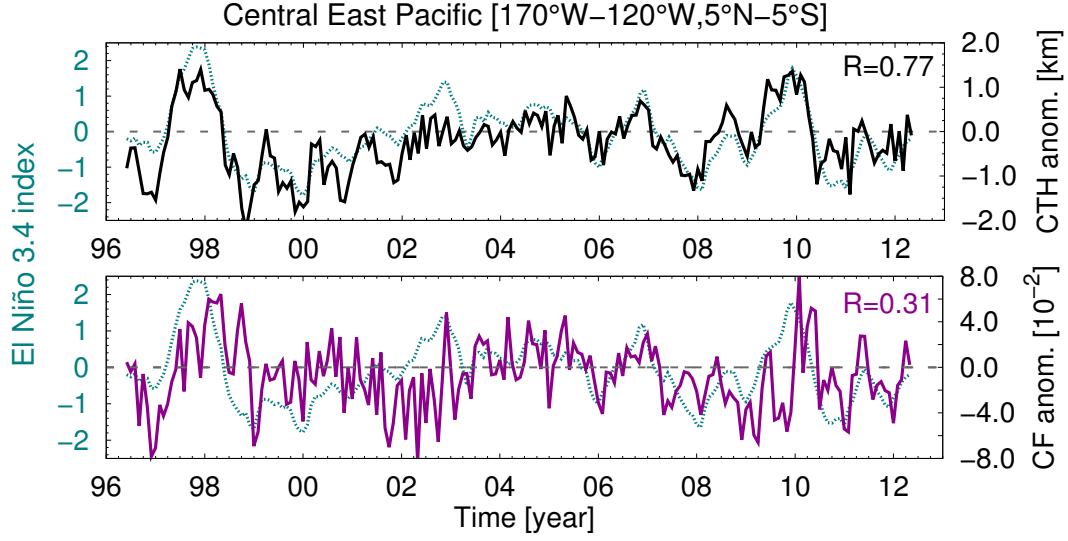
Fig. 7. Time series of cloud top height (top) and cloud fraction (bottom) anomaly over the Central East Pacific with the El Niño 3.4 index.
