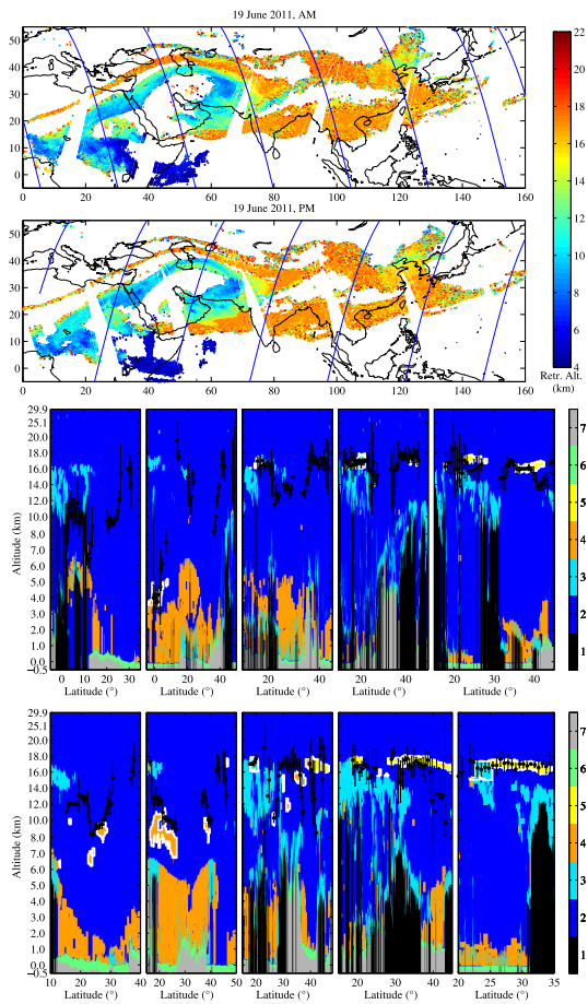
Fig. 9. Same as Fig. 5 for 19 June 2011.
