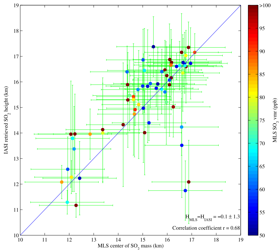
Fig. 10. Comparison of MLS center of SO 2 mass with coincident IASI SO 2 height retrievals in a 200 km radius around the MLS measurements. The MLS errorbar was taken fixed at \pm 1.5 km, the IASI errorbar depicts the standard deviation of the coincident IASI measurements.
