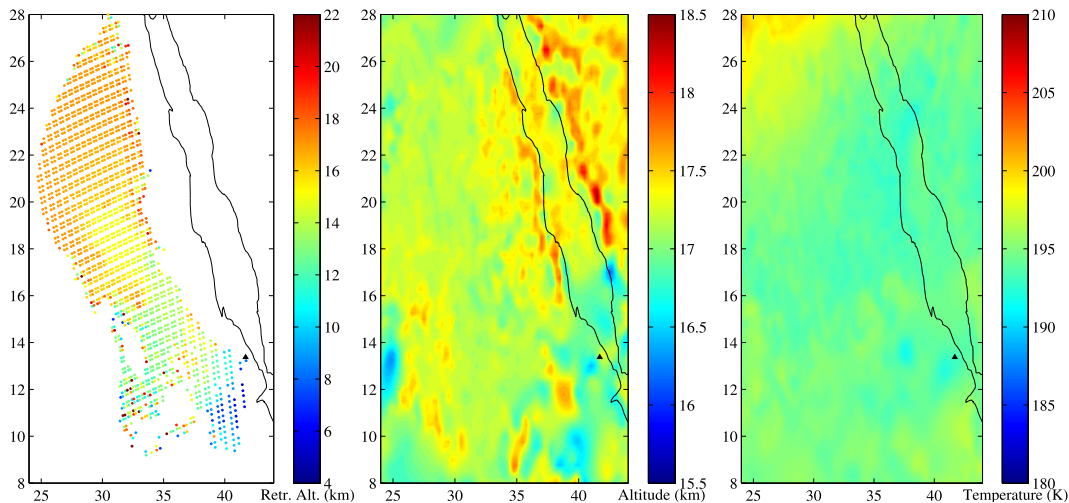
Fig. 2. (Left) IASI retrieved SO 2 altitudes on 13 June (evening overpass). (Middle) Altitude of the tropopause on 14 June (derived from Eumetsat IASI L2 data). (Right) Temperature at the tropopause on 14 June (derived from Eumetsat IASI L2 data).
