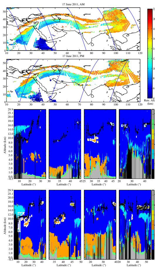
Fig. 7. Same as Fig. 5 for 17 June 2011.
