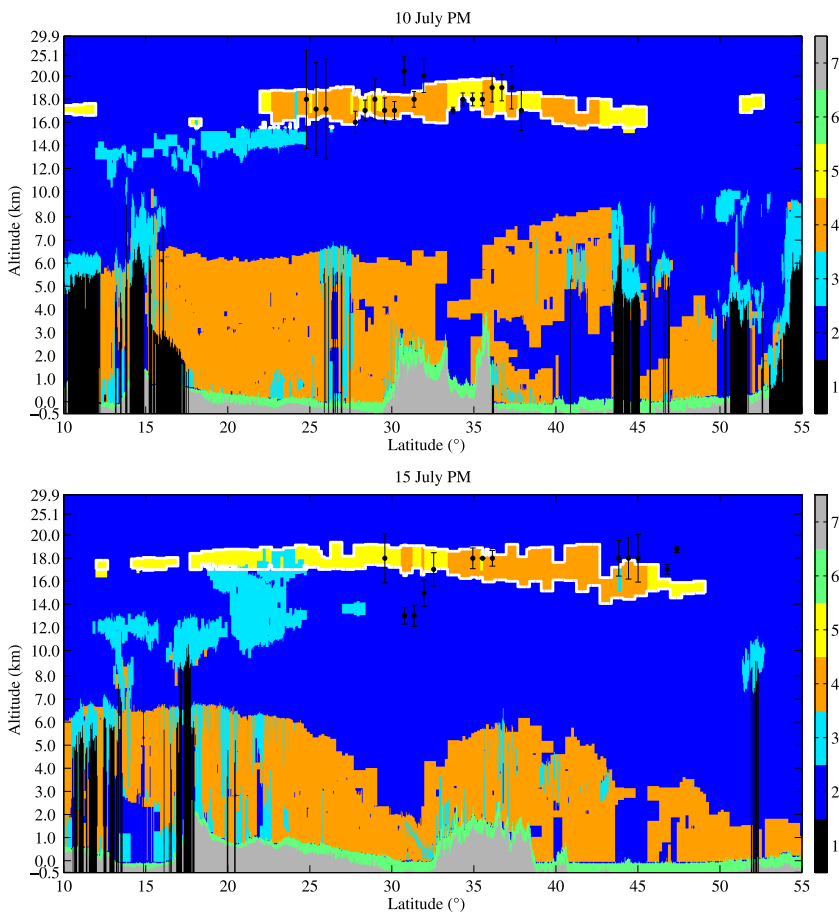
Fig. 13. CALIOP measurements for 10 and 15 July (evening overpass) over the Middle East and coincident IASI retrievals (see text).
