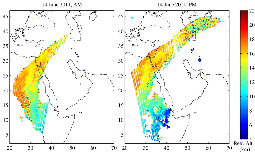
Fig. 3. IASI SO 2 altitude retrievals for 14 June for the morning (left) and evening (right) overpass.
