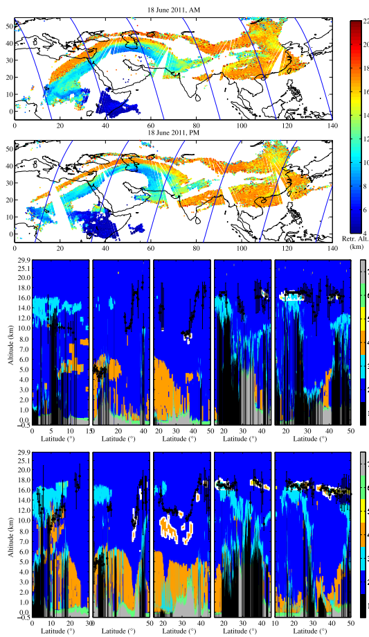
Fig. 8. Same as Fig. 5 for 18 June 2011.
