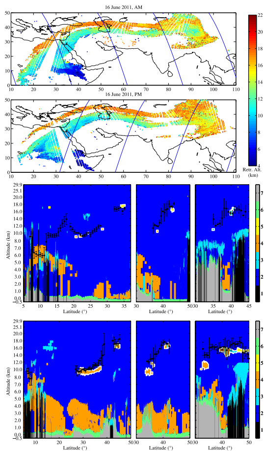
Fig. 6. Same as Fig. 5 for 16 June 2011.
