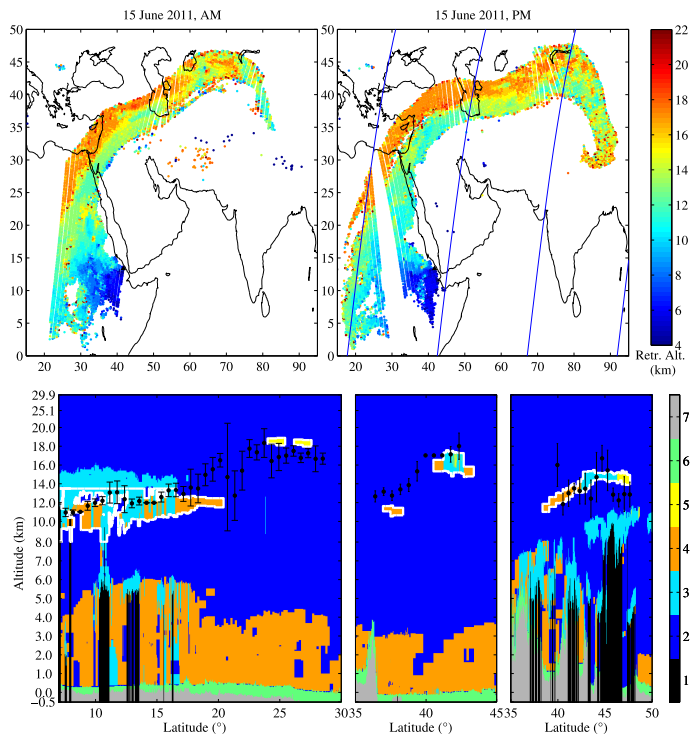
Fig. 5. IASI \text{SO}_2 height retrievals are presented on top from 4 to 22 km; blue lines indicate CALIPSO ground tracks within 5 h of the plume. In the bottom panels, the CALIOP the Level 2 product, “Vertical Feature Mask” is shown for the CALIPSO curtains corresponding to the ground tracks shown above, from left to right. Colors are numbered 1 to 7 indicated in the color bar and stand for: no signal (1), clean air (2), cloud (3), aerosol (4), stratospheric feature (5), surface (6) and subsurface (7). Features which are likely to correspond to sulfate aerosols originating from Nabro are contoured in white on the CALIOP maps. Coincident IASI altitude retrievals are superimposed on these CALIOP maps as black dots, with a standard deviation representing the spread in retrieved altitudes around the overpass.
