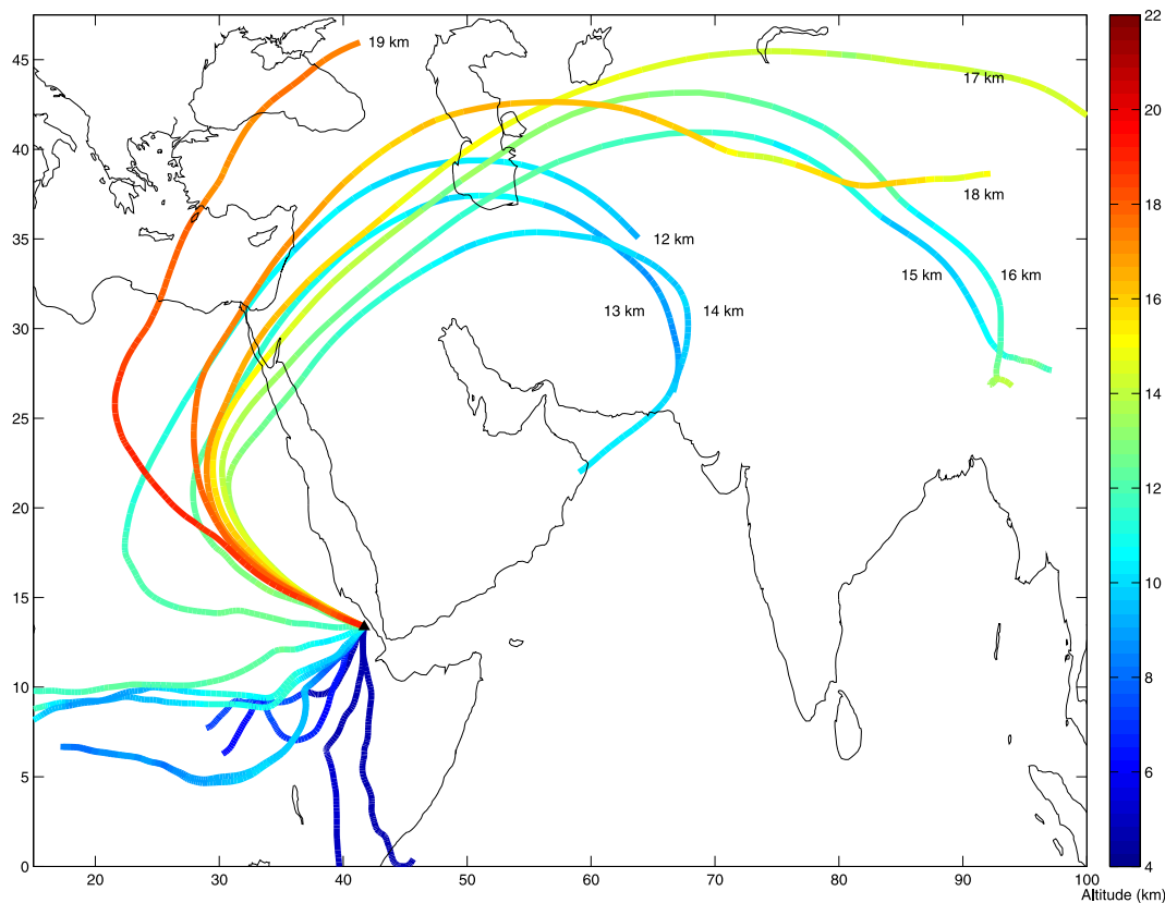
Fig. 4. HYSPLIT trajectories of an instantaneous injection from Nabro at 22:00 UTC on 12 June 2011 with injection heights ranging from 3–19 km for a period of 5 days. The colors of the trajectories indicate the forecasted altitude, rather than the injected altitude.
