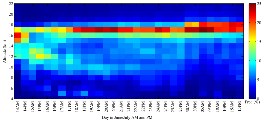
Fig. 12. Frequency of the IASI retrieved SO 2 plume height altitude as a function of time for 14 June to 15 July 2011.
