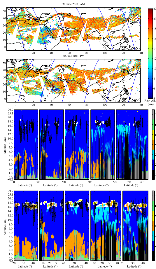
Fig. 11. Same as Fig. 5 for 30 June 2011.
