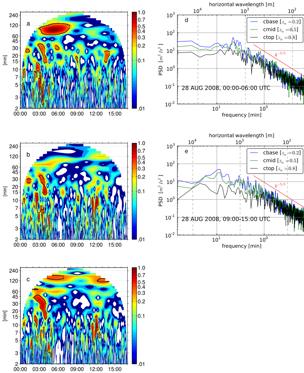
Figure 7. Normalized w wavelet evolution (contours, 1 = maximum observed w -variance; note logarithmic color scale) as a function of frequency scale (ordinate [min]) for 00:00-17:00 UTC on 28 August (hours, abscissa) for a) cloud top ( z_n = 0.8 ), b) cloud mid ( z_n = 0.5 ) and c) cloud base ( z_n = 0.2 ). Wavelet spectral peaks that are statistically significantly (98% confidence level) different than the theoretical red-noise background spectrum, calculated using the lag1 autocorrelation coefficients, have black contour lines. The right panels show the absolute (non-frequency scaled) power spectral density (PSD) of cloud-level (colors) w [ m^2 s^{-2} ] as a function of
