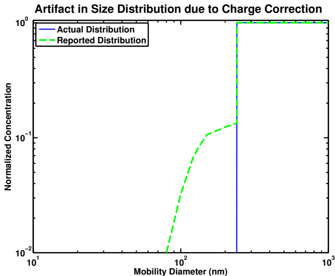
Fig. 4. Artifact introduced into a idealized step function size distribution due to SMPS charge corrections. The “actual” idealized size distribution is shown in blue, and the size distribution reported by a DMA (after charge correction) is shown in dashed green. The difference between the two distribution arises from miss-assigning correctly-sized particles to smaller size bins, as would be done for multiply charged particles. The two sloped regions in the green curve correspond to the singly charged particles mis-assigned as doubly or triply charged.
