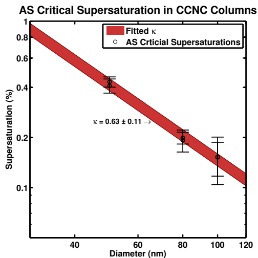
Fig. 2. Left: AS Activation Curves for 50, 80, and 100 nm particles in the A and B columns of the CCNC. Right: Critical supersaturation as a function of mobility diameter from the interpolated 50% activation points from the curves on the left. A \kappa value of 0.63 \pm 0.11 corresponds well with the literature value of \kappa_{AS} = 0.61 (Petters and Kreidenweis, 2007a) and provides validation of the CCNC setup.
