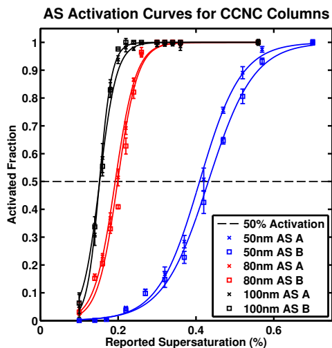
Fig. 2. Left: AS Activation Curves for 50, 80, and 100 nm particles in the A and B columns of the CCNC. Right: Critical supersaturation as a function of mobility diameter from the interpolated 50% activation points from the curves on the left. A \kappa value of 0.63 \pm 0.11 corresponds well with the literature value of \kappa_{AS} = 0.61 (Petters and Kreidenweis, 2007a) and provides validation of the CCNC setup.
