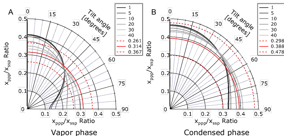
Fig. 4. Radial plots indicating methyl C_{3v} tilt angle as a function of A_{ppp}/A_{ssp} amplitude ratio of the methyl symmetric stretching mode for vapor (left) and spin-coated (right) trans - \beta -IEPOX (1) calculated as described in the text. Solid red curves indicate the experimentally determined ratio point estimates, and dashed red curves indicate the standard errors of these ratios. Gray curves indicate theoretically calculated monomodal Gaussian orientation distributions of widths ranging from 1 to 40°.
