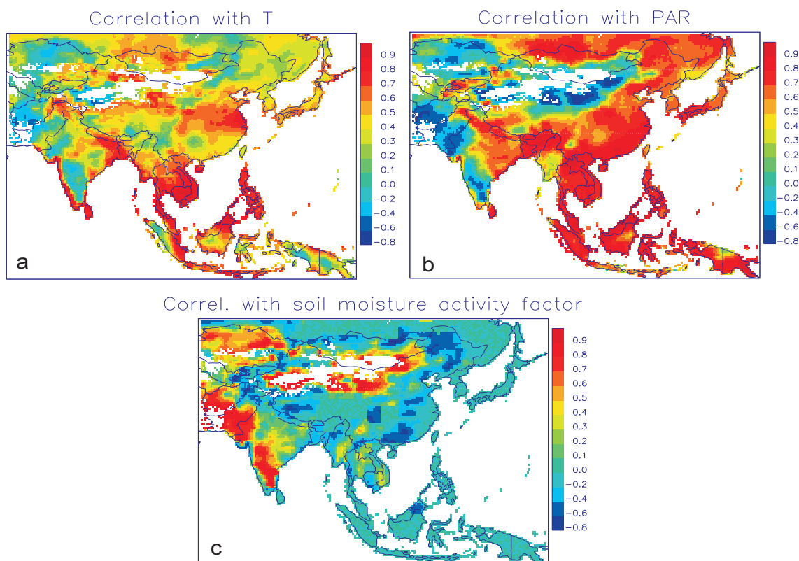
Fig. 4. Correlation coefficient between the annual isoprene emission and air temperature (a), above-canopy solar radiation (b), and the soil moisture stress activity factor (c) over 1979-2012.
