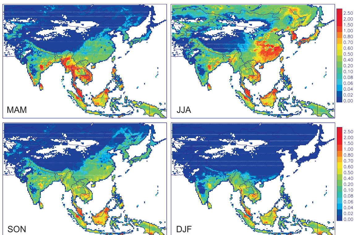
Fig. 9. Seasonal isoprene emission rates calculated by the S4 simulation in 2005 expressed in \text{mg isoprene m}^{-2} \text{h}^{-1} in March-April-May (MAM), June-July-August (JJA), September-October-November (SON), and December-January-February (DJF).
