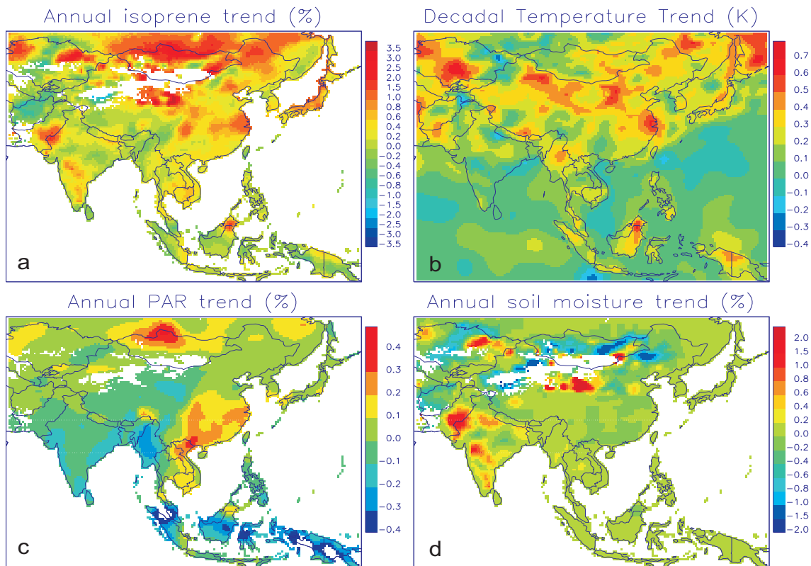
Fig. 5. Annual percentage trend in isoprene emissions derived from the S0 simulation (a), decadal temperature trend (b), annual percentage PAR trend (c) and annual percentage trend in the soil moisture activity factor (d) over 1979-2012 based on ERA-Interim data.
