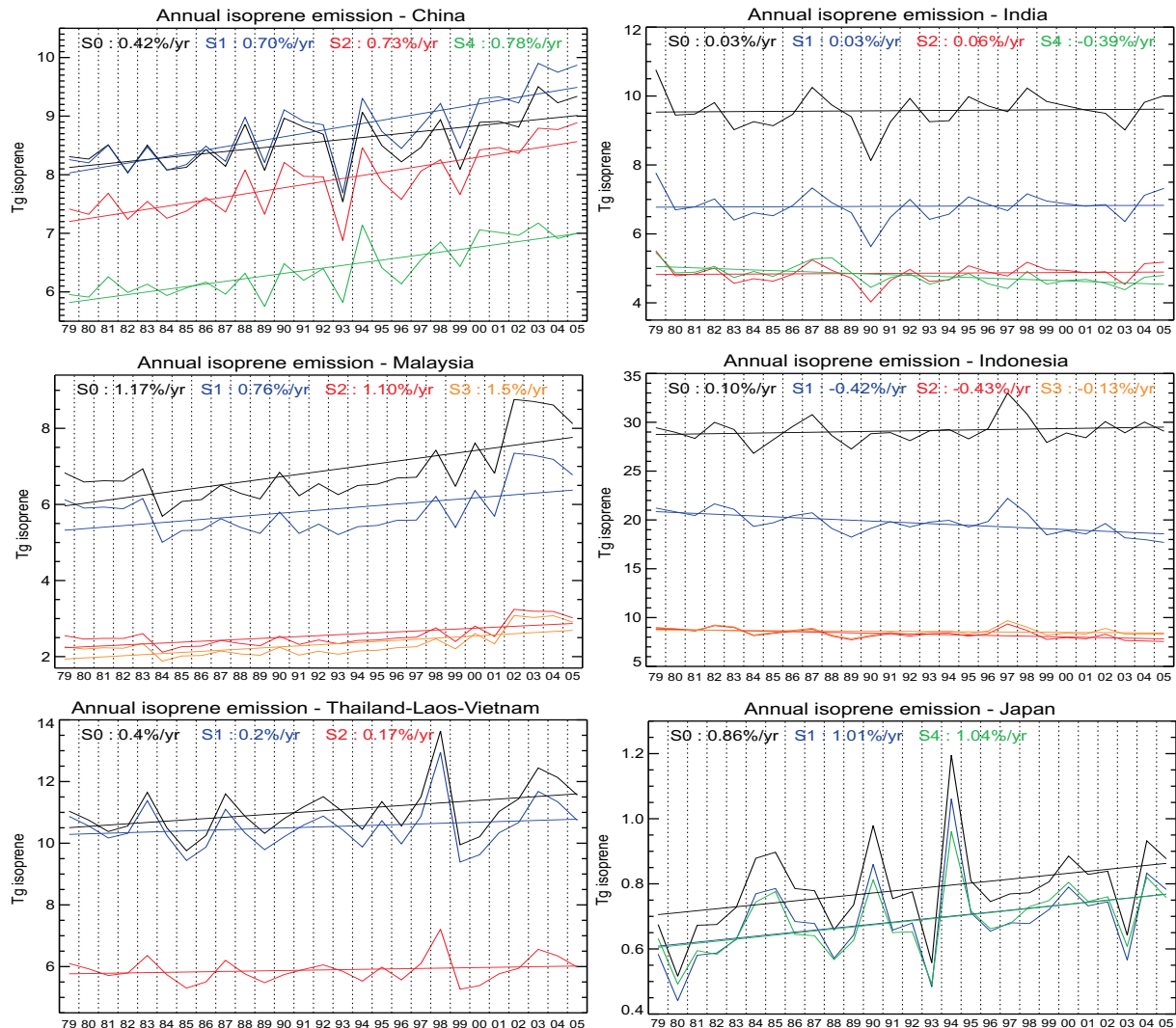
Fig. 10. Annual isoprene emission per country between 1979 and 2005. The colours denote the different simulations : S0 in black, S1 in blue, S2 in red, S3 in orange, and S4 in green (Table 1). Relative trends obtained by linear regression are given inset following the same colour code. Scenarios yielding identical results are not shown, e.g. S2 and S3 over Japan.
