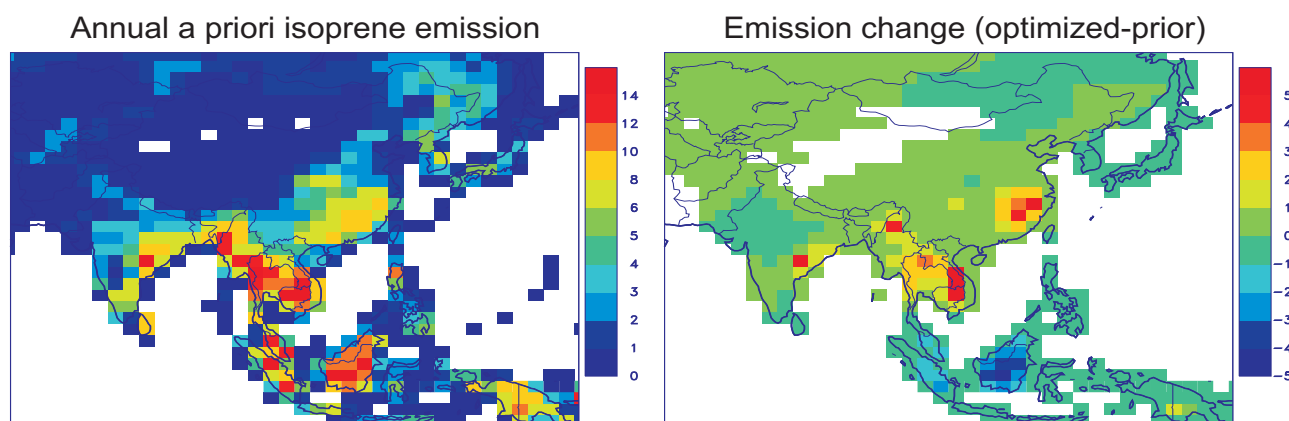
Fig. 12. Annual a priori isoprene emission in 2008 and deviation from the a priori inferred by an inversion constrained by GOME-2 HCHO columns. Units are 10^{10} \text{ molec. cm}^{-2} \text{ s}^{-1} . The a priori inventory is obtained from the S4 simulation (cf. Sect. 7.1).
