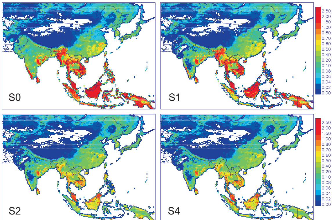
Fig. 8. Annually averaged isoprene emission rates computed in S0, S1, S2 and S4 simulation for 2005. S1 accounts for land use change effects, S2 also incorporates reduced emission rates from tropical forests, and S4 includes both updates in solar radiation and in the representation of oil palm in Indonesia and Malaysia (Table 1). S4 simulation is identical to S3 over Indonesia and Malaysia.
