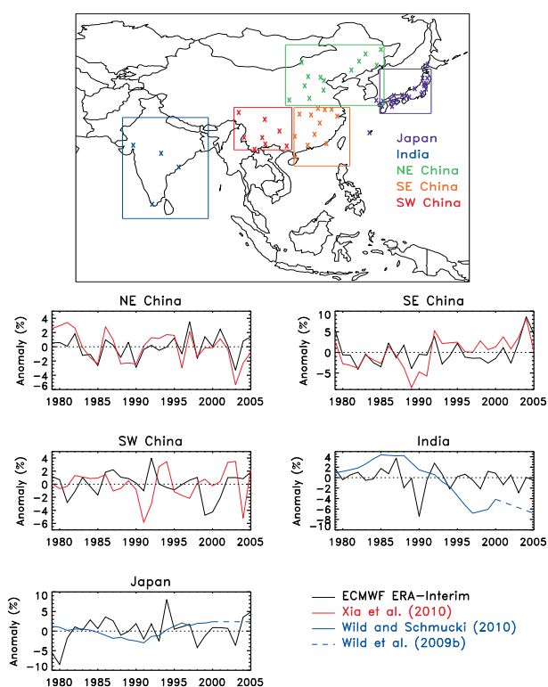
Fig. 3. Upper panel : The crosses represent the locations of surface radiation measurement stations in China, Japan and India, as reported in Xia (2010); Wild and Schmucki (2010). Lower panel: Annual downward surface solar radiation (SSR) anomaly (in %) derived from ERA-Interim fields (black) and corrected based on ground-based SSR observations in China (Xia, 2010), India and Japan (Wild and Schmucki, 2010; Wild et al., 2009b).
