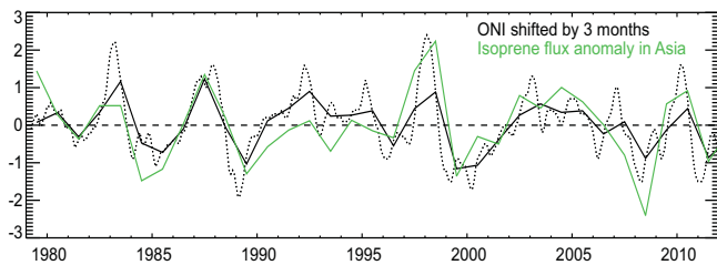
Fig. 7. Isoprene flux anomaly in Asia (green) and comparison with 650 the Oceanic Niño Index (black) shifted by 3 months over the target period. Dotted and solid black lines correspond to monthly and annual ONI data, respectively.
