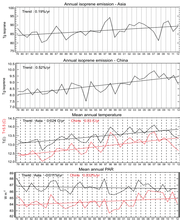
Fig. 6. Annual isoprene emissions (Tg) in the whole domain, and 635 China (two upper panels) over 1979-2012 using the S0 simulation. Annual temperature and PAR (bottom) in Asia (black) and China (red) are shown in the two lower panels over the same period. Lin- ear regression trends are given inset and applied over the whole simu- lation period.
