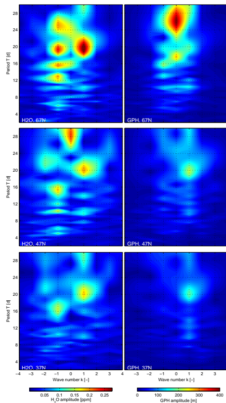
Fig. 4. Periodogram for travelling and stationary planetary waves in water vapor (left panels) and geopotential height (right panels) on 0.05 hPa (approximately 70 km) as observed by Aura MLS at the latitudes of the ground based microwave radiometers (67° N, 47° N and 37° N, from top to bottom) during boreal winter 2011/2012.
