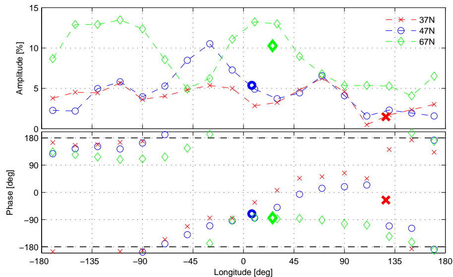
Fig. 5. Amplitudes (top panel) and phase (bottom panel) of the 20 day wave in water vapor on 0.05 hPa as observed by Aura MLS and the three ground based microwave radiometers during boreal winter 2011/2012. The bold symbols are from the ground based radiometers (Bern at 7.5° E, Sodankylä at 26.6° E and Seoul at 127° E) and the thin symbols connected with dashed lines are from Aura MLS at the latitudes of the ground based microwave radiometers (37° N for Seoul, 47° N for Bern and 67° N for Sodankylä).
