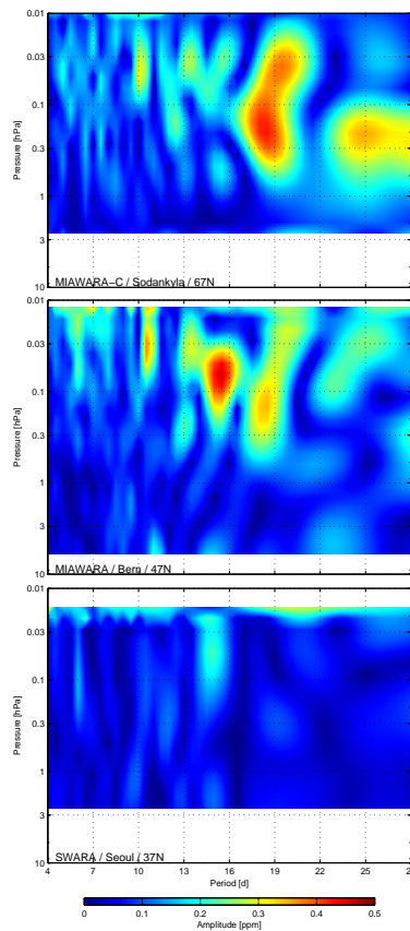
Fig. 1. Average wave amplitudes from the spectral analysis of the water vapor measurements from the three ground-based microwave radiometers in Sodankylä, Bern and Seoul (from top to bottom) for the period from 1 December 2011 to 31 March 2012. See description within the text for details about the calculation method.
