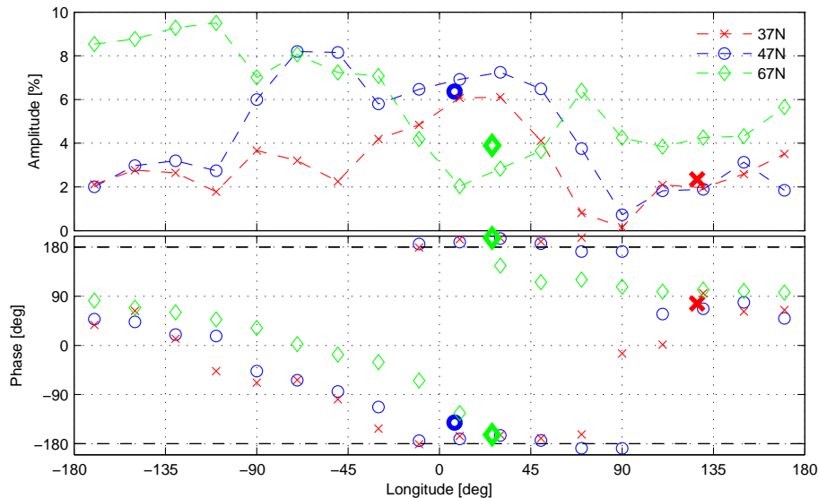
Fig. 6. Analogous to Fig. 5 but for the 16-day wave.
