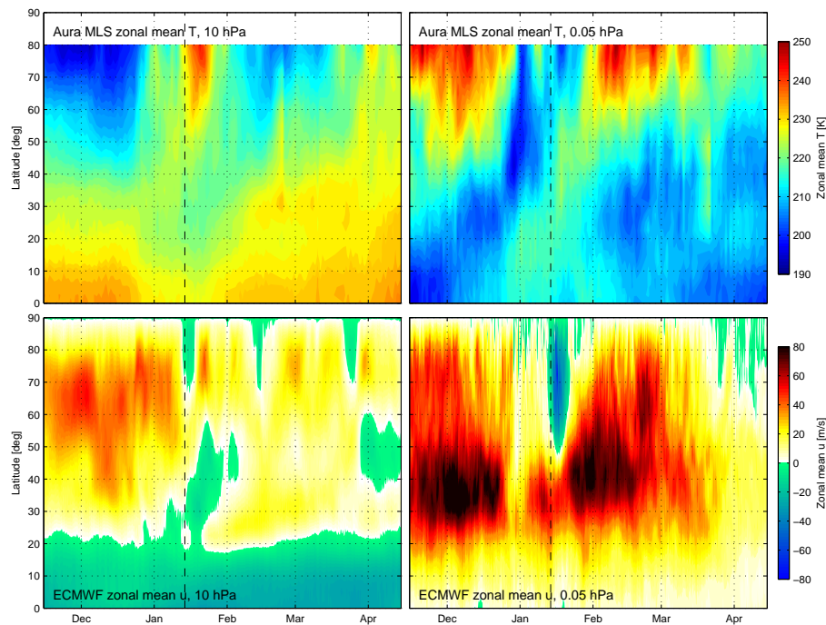
Fig. 3. Zonal mean Aura MLS temperature (top panels) and ECMWF zonal wind (bottom panels) on 10 hPa (left panels) and 0.05 hPa (right panels) during boreal winter 2011/2012. The black dashed lines indicates the beginning of the SSW on 14 January 2012.
