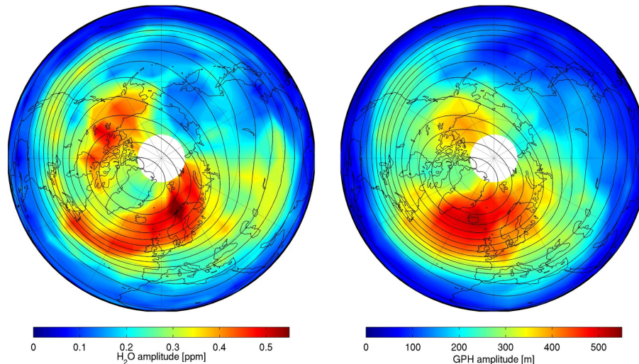
Fig. 7. Hemispheric map of the amplitude of the quasi 16-day wave in water vapor (left panel) and geopotential height (right panel) on 0.05 hPa as observed by Aura MLS during boreal winter 2011/2012. The amplitude is obtained by averaging the wave amplitude of the bandpass filtered water vapor and geopotential height time series with a bandpass range from 14 to 20 days. The contour lines represent the average geopotential height on 0.05 hPa between 1 December 2011 and 31 March 2012. The contour lines are equally spaced.
