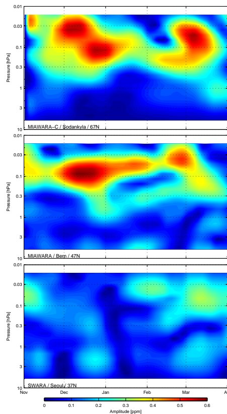
Fig. 2. Amplitude of the bandpass filtered water vapor time series as observed by the three ground-based microwave radiometers in Sodankylä, Bern and Seoul (from top to bottom). The lower and upper bandpass limits are 14 and 20 days, respectively. See description within the text for details about the calculation method.
