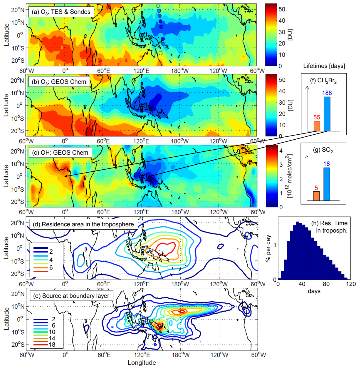
Fig. 4. Tropospheric ozone columns from (a) TES for October 2009 (results for 2005–2009 are similar, see Fig. 5), the sondes (dots, dates see Fig. 1), and (b) GEOS Chem (mean 1–15 October 2009). (c) OH columns from GEOS-Chem (mean 1–15 October 2009). (d, e, h) show ATLAS 4-months backtrajectory runs for air entering the stratosphere (1 October–31 January). Average conditions for 2002–2011, individual results for 2009 in Fig. 7 and Fig. 8. (d) Density distribution function of the horizontal positions of the trajectories between the boundary layer and the LCPs. (e) Density distribution function of the horizontal positions of the last contact with the boundary layer. The values in (d) and (e) are normalized such that a horizontally uniform distribution corresponds to a value of 1 at every grid point. (f–g) Examples of gas-phase lifetimes of relevant species in the mid-troposphere (500 hPa) at the equator for typical conditions over the Atlantic (0° E, orange) and for conditions in the OH minimum (130° E, blue). (h) Distribution of residence times between last contact with the boundary layer and the LCP for trajectories ascending into the stratosphere.
