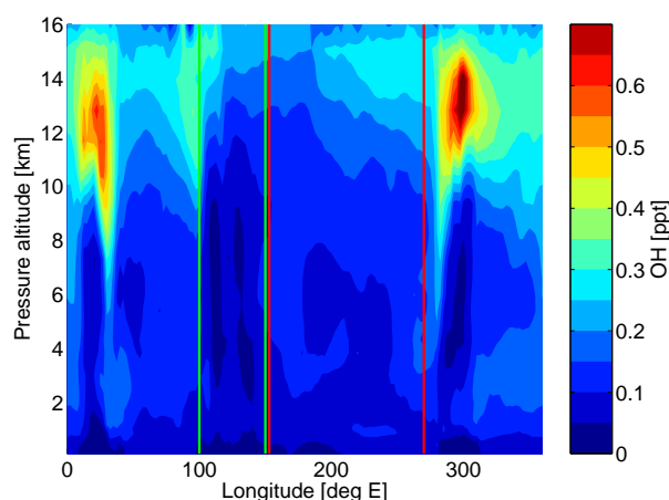
Fig. 6. Cross section of equatorial OH mixing ratio profiles modeled with GEOS-Chem, averaged over the first half of October 2009. The area between the green lines denotes the region of the OH minimum in Fig. 4c. The area between the red lines shows the longitudinal extent of the NASA DC-8 flights of the PEM-Tropics B campaign (which were not always directly at the equator).
