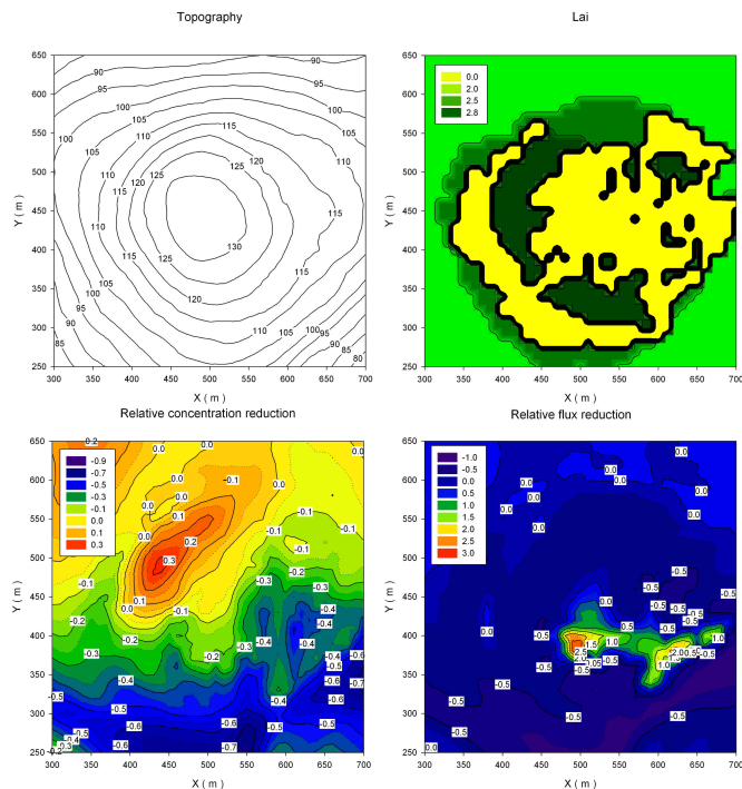
Fig. 3. Exemplary relative dilution simulation of a passive scalar at the height of 4 m for a southward wind direction ( 0^\circ ). The figures display: (top, left) the topography, (top right) the leaf area index distribution, (bottom left) concentration difference scaled to the concentration at the forest edge and (bottom right) relative trace gas flux reduction (Eq. (4), see Fig. 2). The measurement container for gases and some aerosol parameters at the hill top is located at (480 m, 430 m). Further plots can be found in supporting online information.
