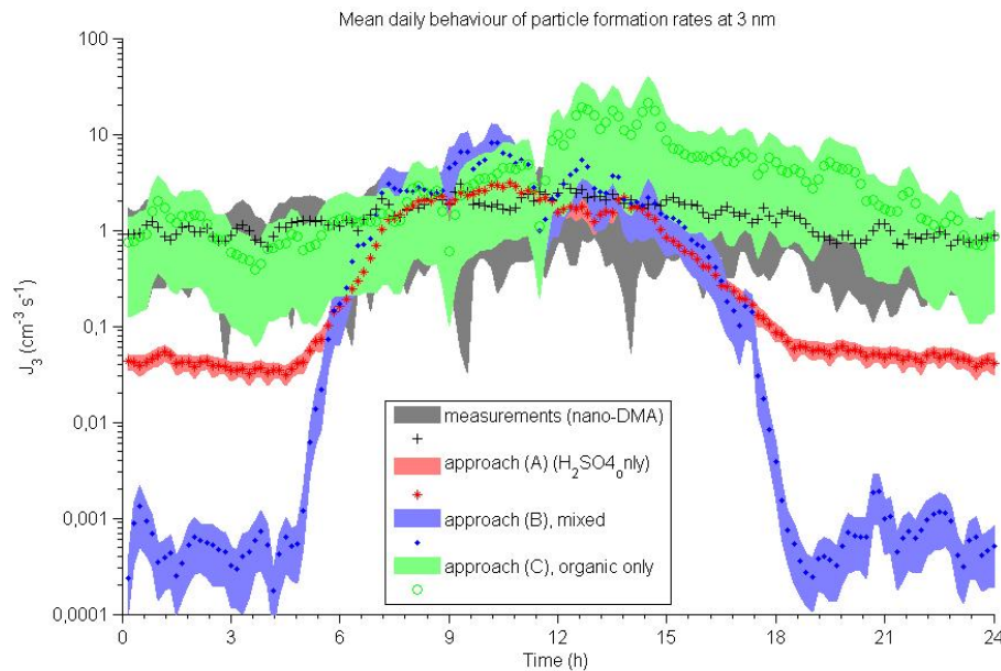
Fig. 11. Mean daily pattern of measured and calculated particle formation rates at 3 nm diameter.
