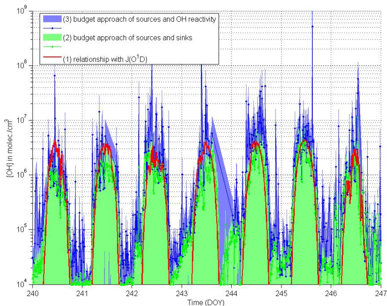
Fig. 4. Concentrations of ambient OH calculated through different approaches for a period during PARADE (DOY 240–247): (1) J(O^1D) based formulation, (2) budget approach of measured individual sources and sinks as well as (3) budget approach of measured individual sources and OH reactivity. The extended version can be found in supporting online information.
