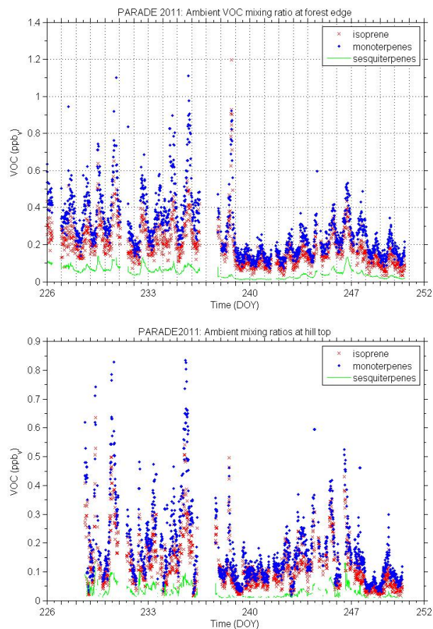
Fig. 6. Measured volume mixing ratios at the forest edge (top) and calculated mixing ratios at the hill top (bottom) of isoprene, mono- and sesquiterpenes.
