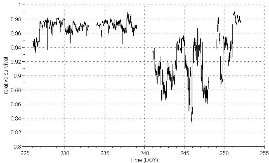
Fig. 14. Calculated relative survival of particles during growth from 3 to 5 nm.
