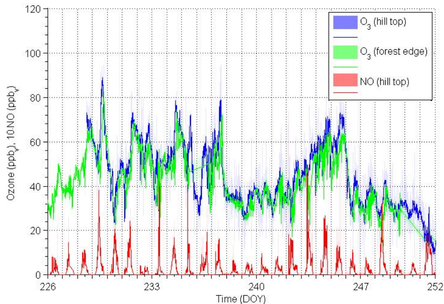
Fig. 7. Detailed behavior of detected ambient ozone and NO mixing ratios. Note, detection limit of NO was 21 ppt v .
