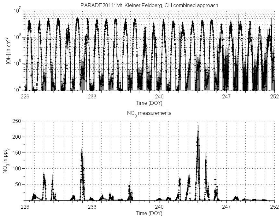
Fig. 8. (top) Calculated OH concentrations at the hill top. (bottom) Detected NO 3 radical mixing ratios at the same location.
