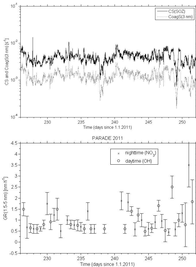
Fig. 12. (top) Calculated condensation (CS) and coagulation sinks (CoagS(3 nm)) and (bottom) mean growth rates (GR) of clusters or particles between 1.5 and 5 nm in diameter.
