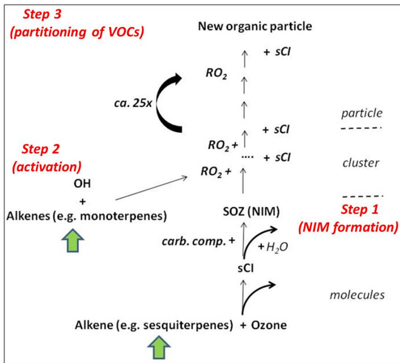
Fig. 1. Particle formation scheme of hypothesis (C) by organic compounds only. Three essential steps, of which the first two can both limit nucleation, are marked.
