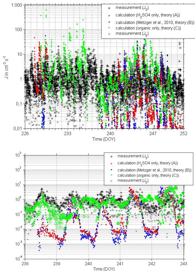
Fig. 10. (top) Measured and derived particle formation rates at 3 nm in particle diameter and measured one at 5 nm. (bottom) Zoom to five days only in order to show the behavior at different times of the day.
