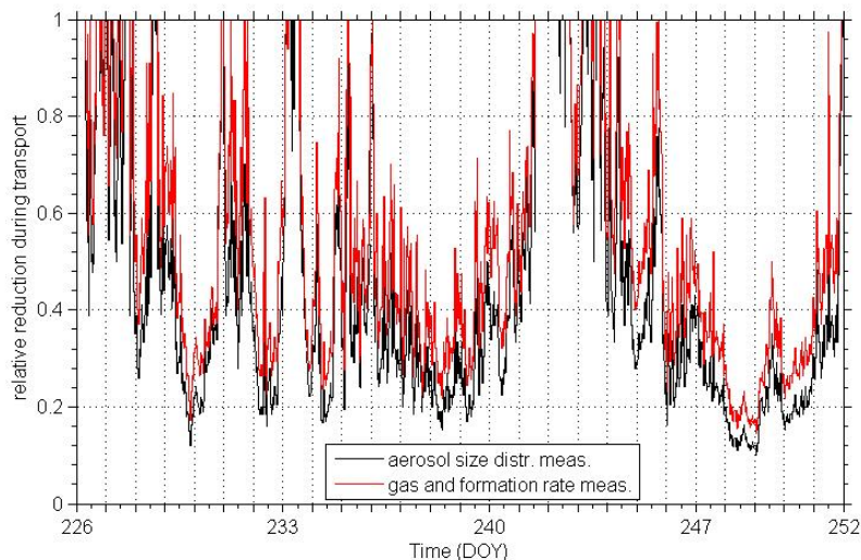
Fig. 5. Relative reduction of concentrations during transport from the forest edge to the hill top depending on the present wind direction and speed. This factor is used for scaling the measured VOC concentrations to obtain values after transport.
