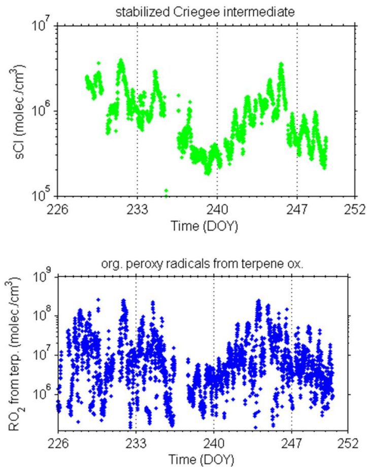
Fig. 9. (top) Estimated ambient stabilized Criegee Intermediates (sCI) and (bottom) \text{RO}_2(\text{terp.}) radicals.
