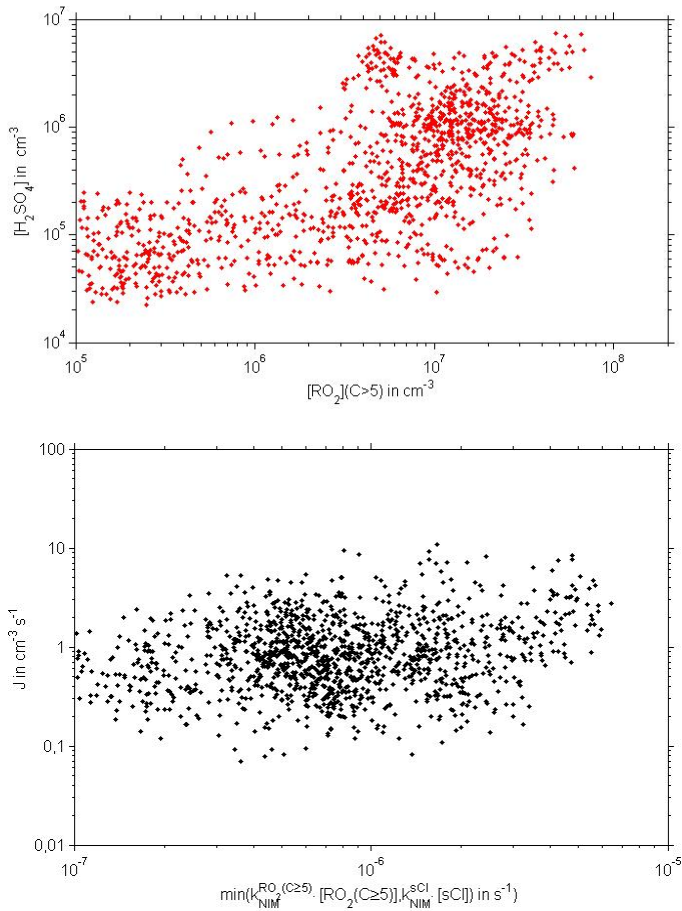
Fig. 16. Scatter plot of the activation term in Eq. (5) vs. the formation rate.
