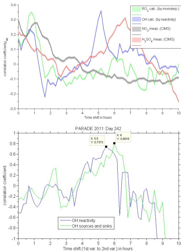
Fig. 13. (top) Cross-correlation of particle formation at 5 nm with RO 2 (terp.), OH, NO 3 and H 2 SO 4 . (bottom) Cross-correlation between the particle formation rate at 5 nm and the estimated OH-concentration using two different approaches. The maximum is found at \tau of 5.5 h (6 h for the budget approach), resulting in a GR of 3.5 nm/5.5 h = 0.6 nm/h.
