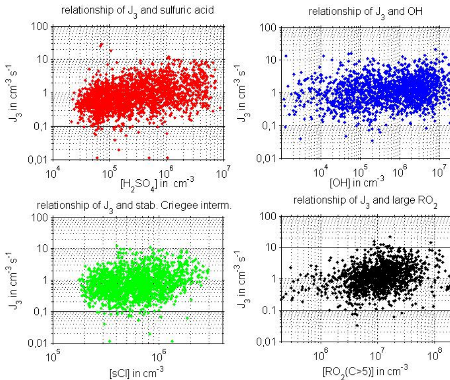
Fig. 15. Scatter plots of sulphuric acid, OH, stabilised Criegee intermediates and large organic peroxy radicals by monoterpene oxidation ( RO_2(\text{terp}) ) with the particle formation rate at 3 nm.
