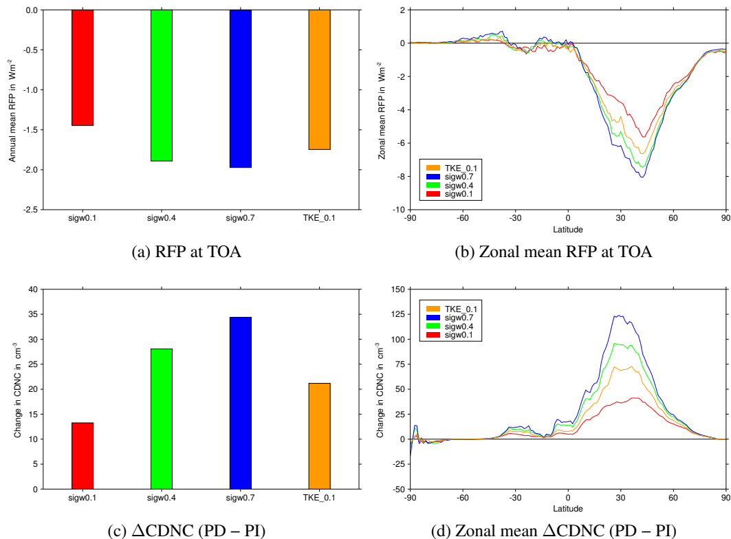
Fig. 8. RFP due to total anthropogenic aerosol effects and change in annual mean CDNC (at 720m) for model configurations sigw0.1 (red), sigw0.4 (green), sigw0.7 (blue) and TKE_0.1 (orange). (a) and (c) show differences in global mean (PD – PI); (b) and (d) show differences in zonal mean (PD – PI).
