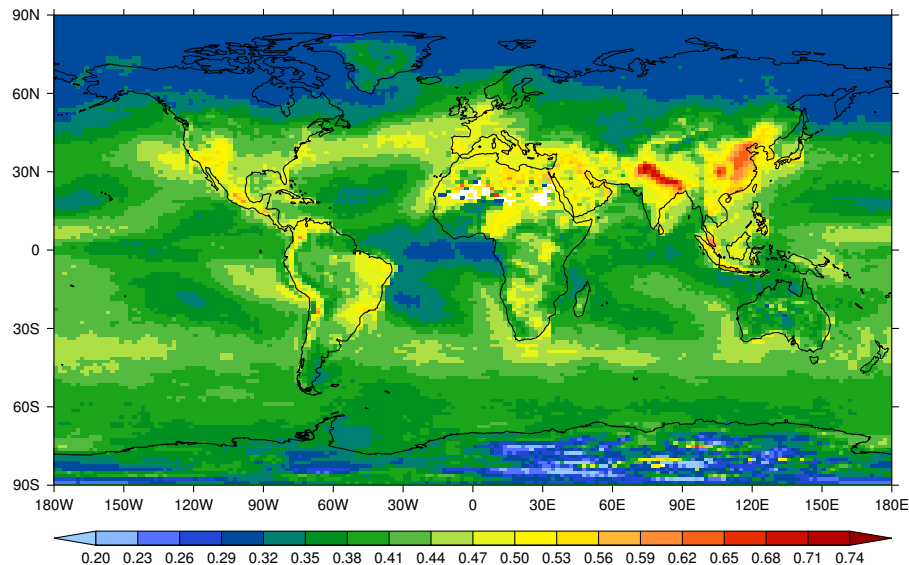
Fig. 5. Annual mean in-cloud \lambda calculated from w^* = \lambda \sigma_w from model configuration sigw0.4 at hybrid height of 720 m (AWM = 0.40).
