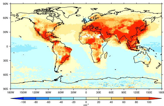
(a) \Delta CDNC in sigw0.4 (PD – PI)
