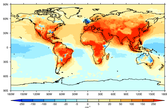
(b) \Delta CCN sigw0.4 (PD – PI)
