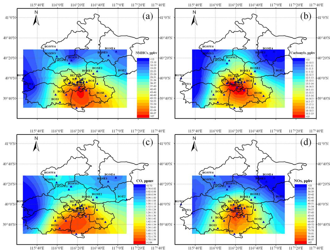
Fig. 1. Contour maps of annual average mixing ratios of (a) total NMHCs, (b) total carbonyls, (c) CO, and (d) NO x in Beijing. Blue triangles indicate sampling locations and the names of these sites were listed in Table S1.
