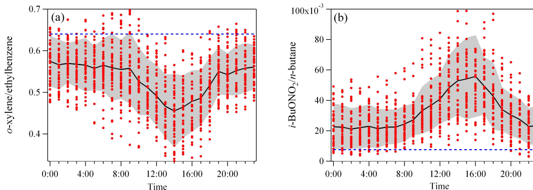
Fig. 5. Diurnal variation in hourly average ratios of (a) o -xylene/ethylbenzene (X/E), and (b) i -BuONO 2 / n -butane. The red dots correspond to the measured ratios. The grey areas represent one standard deviation from the hourly average ratios. The blue dashed line corresponds to the average ratio at the time of emission.
