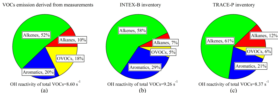
Fig. 10. Comparison of the relative contributions of VOC groups to the total OH reactivity of measured VOC species from (a) measurements, (b) the INTEX-B emission inventory (Zhang et al., 2009), and (c) the TRACE-P emission inventory (Streets et al., 2003). The OH reactivity for each VOC species was calculated as the product of its emission ratio, rate constant with OH ( k_{OH} ), and an assumed CO mixing ratio (1.0 ppmv).
