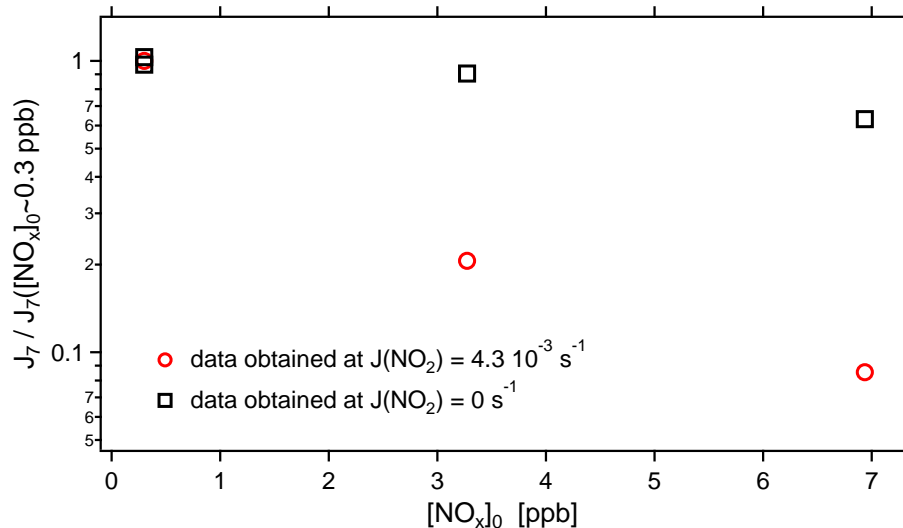
Fig. 8. J_7 normalized to J_7 measured at [\text{NO}_x]_0 \sim 0 as a function of [\text{NO}_x]_0 . Red circles: data points measured at J(\text{NO}_2) = 4.3 \times 10^{-3} \text{ s}^{-1} , black squares: data measured at J(\text{NO}_2) \sim 0 \text{ s}^{-1} . In the presence of UVA light suppression of J_7 by \text{NO}_x addition was more pronounced than in the absence of UVA light. Note the logarithmic scale for J_7 .
