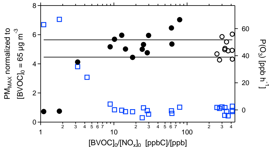
Fig. 7. PM_{MAX} normalized to [BVOC]_0 = 65 \mu\text{g m}^{-3} in dependence of BNR. Solid circles show data from experiments with \text{NO}_x addition; open circles are from experiments without \text{NO}_x addition. The black lines show the average \pm 1\sigma standard deviation (upper/lower line) of the data without \text{NO}_x addition. For comparison P(\text{O}_3) is shown (blue squares) as in Fig. 5. For one of the experiments (BNR = 4.3, [\text{NO}_x]_0 = 23 \text{ ppb} ) PM_{MAX} was not available. Therefore the number of data in Fig. 7 is by one less than that in Fig. 5.
