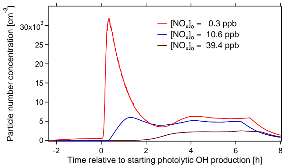
Fig. 3. Temporal shape of particle number concentrations for different [\text{NO}_x]_0 .
