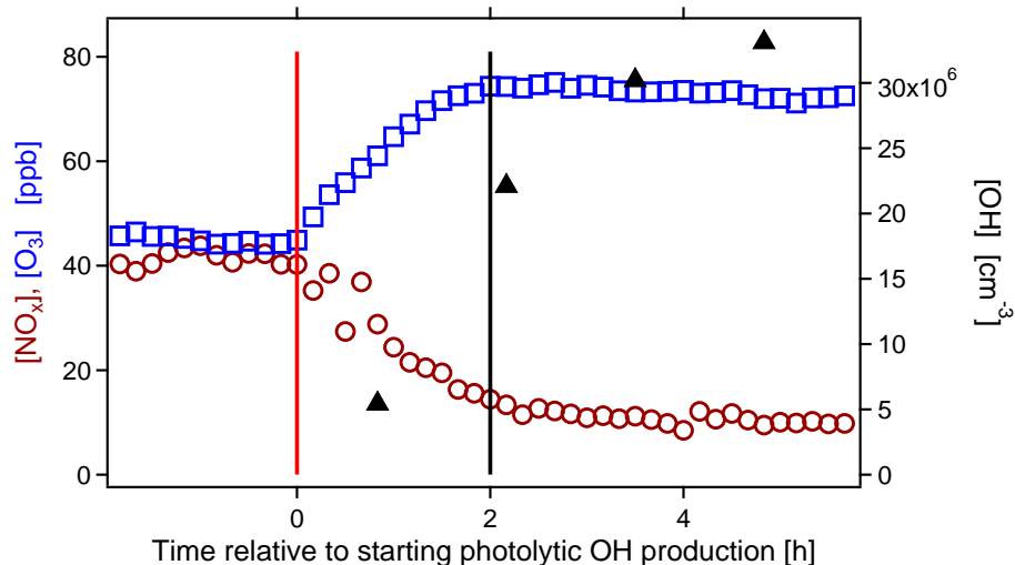
Fig. 4. Temporal behavior of [\text{NO}_x] (brown circles, left scale), [\text{O}_3] (blue squares, left scale) and [\text{OH}] (black triangles, right scale) in an experiment with [\text{NO}_x]_0 \sim 40 ppb, [\text{BVOC}]_0 \sim 124.5 ppbC. OH concentrations were measured indirectly by GC-MS with a time resolution of \sim 70 min. The red bar shows the time when the TUV lamp was switched on and the black bar shows the time when the particle number concentrations increased significantly above the background.
