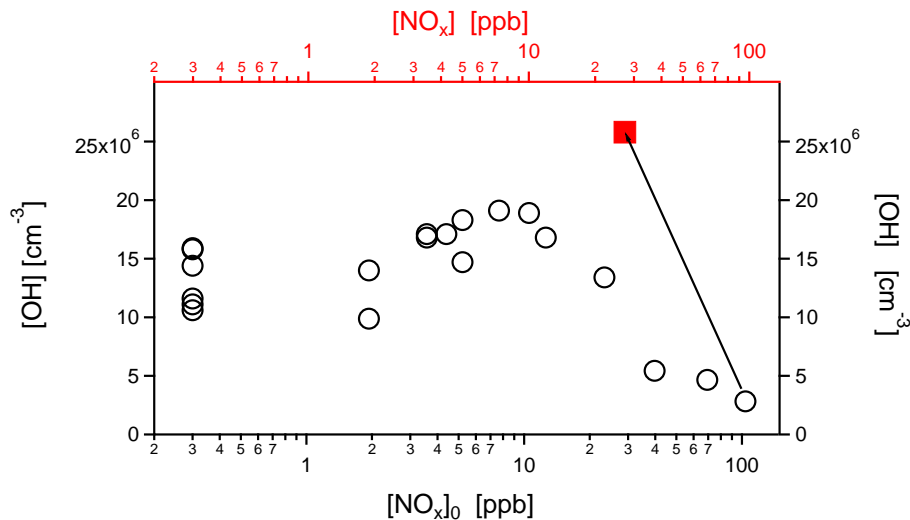
Fig. 6. OH concentrations measured during the first hour after switching on the TUV lamp in dependence of [\text{NO}_x]_0 (black circles, note the logarithmic scale of x-axis). The red square shows the OH concentration measured for the experiment with the highest \text{NO}_x addition ( [\text{NO}_x]_0 = 103.5 ppb), 5 h after ignition of the TUV lamp. After that time new particle formation was observed, [\text{O}_3] had increased to 85 ppb and [\text{NO}_x] had decreased to 26 ppb.
