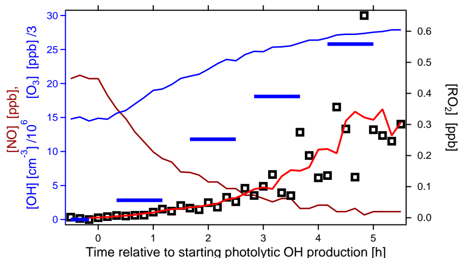
Fig. 9. Estimated [RO_2] ( = \sum_i [RO_2^i] ) using deviation from PSS and an average rate constant k_2 = 9 \times 10^{-12} \text{ cm}^3 \text{ s}^{-1} for Reaction (R2). The open squares show the original data, the red line shows the five point moving average of the [RO_2] data (both right hand y-scale). The brown line shows the NO concentrations measured during the experiment, the blue bars show OH concentrations divided by 10^6 for clarity, and the blue line shows the ozone concentrations divided by 3 for clarity (left hand y scale). New particle formation started 5 h after the TUV lamp was switched on. Then [NO] had decreased to \sim 1 ppb and [RO_2] had increased to \sim 300 ppt.
