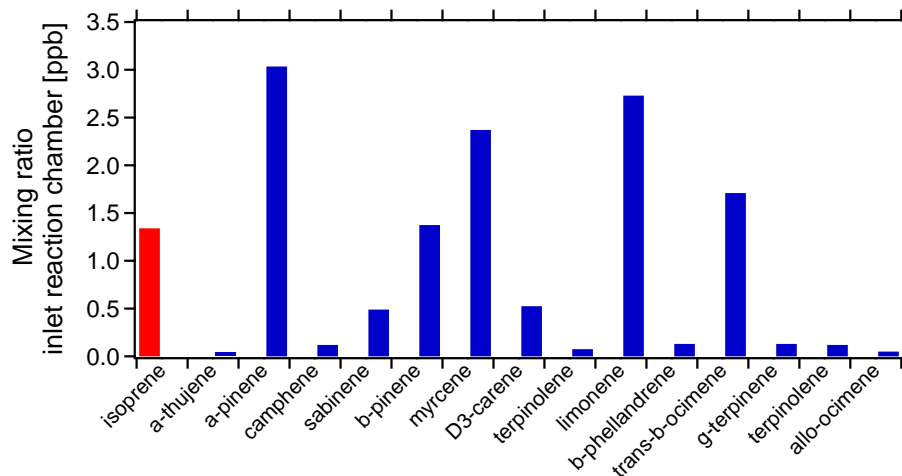
Fig. 2. BVOC mixing ratios at the inlet of the reaction chamber. Dilution by the second air stream is already considered, the sum of mixing ratios represents [\text{BVOC}]_0 . The plants in the plant chamber (two Aleppo pines, one Holm oak, one Palestine oak, and one Pistachio) constitutively emitted isoprene (red bar) and monoterpenes (blue bars).
