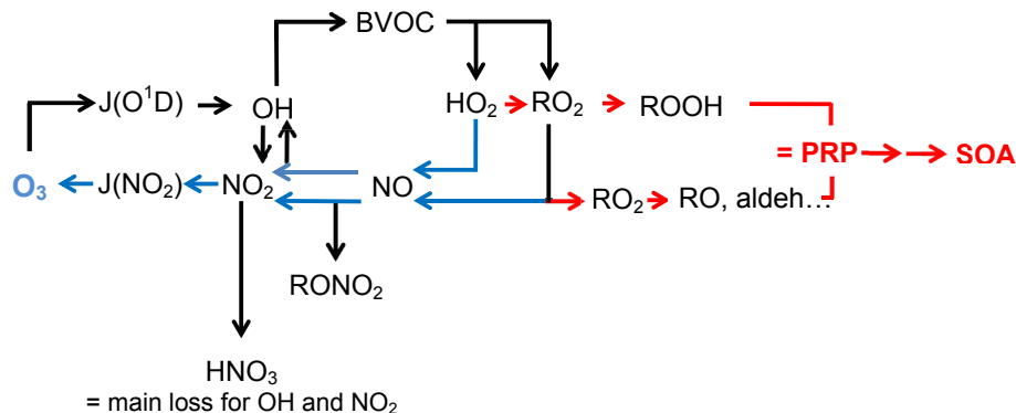
Fig. 1. Schematics of the basic reactions considered here. BVOC oxidation forms peroxy radicals that, dependent on NO concentrations, have different fates. At low NO x conditions, permutation reactions among RO 2 (including HO 2 ) are predominant (red arrows). Products of permutation reactions are termed as PRP. At high NO x conditions, peroxy radicals react predominantly with NO. Products of RO 2 + NO reactions are NO 2 and organic nitrates. NO 2 is photolysed and subsequently O 3 is formed. On photolysis in the ultraviolet, O 3 is precursor of OH. Main sink of OH, the oxidant driving this chemistry, is the OH + NO 2 reaction. This reaction is also the main sink of NO 2 in the system.
