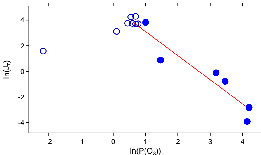
Fig. 10. Double logarithmic plot of J_7 ( J_7 in units of \text{cm}^{-3}\text{s}^{-1} ) vs. P(O_3) ( P(O_3) in units of \text{ppbh}^{-1} ). Open circles are data obtained at P(O_3) < 2.5 \text{ ppbh}^{-1} , closed circles are data obtained at P(O_3) > 2.5 \text{ ppbh}^{-1} . Data pairs with P(O_3) < 2.5 \text{ ppbh}^{-1} were regarded as error prone because P(O_3) was calculated to -0.15 \pm 2.5 \text{ ppbh}^{-1} when no \text{NO}_x was added and P(O_3) was essentially zero. Therefore linear regression analysis was restricted to data points with P(O_3) > 2.5 \text{ ppbh}^{-1} . The line shows the result from linear regression analysis resulting in a slope of -1.9 \pm 0.37 , R^2 = 0.87 . Data points with formally negative P(O_3) are not included in the plot.
