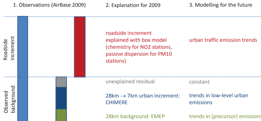
Fig. 1. Schematic overview of the traffic station scheme. Observed roadside concentrations (left) are first disaggregated into background and traffic increment (step 1), then the different components are explained to the extent possible for 2009 (step 2). For the roadside increment, this involves estimating the station-specific parameters (residence time of air in the street canyon, background representativeness correction if needed). For the modelling of scenario years other than the base year (step 3), we consider changes in European wide NO x emissions for the background, and changes in urban driving emissions (including changes in primary NO 2 emissions) for the traffic increment.
