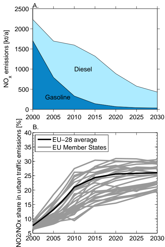
Fig. 10. (A) Trends in \text{NO}_x emissions from passenger cars in the EU-28 under the current legislation scenario. (B) Share of primary \text{NO}_2 in \text{NO}_x emissions from road traffic, in the individual EU Member States (grey) and the EU-28 mean (black).
