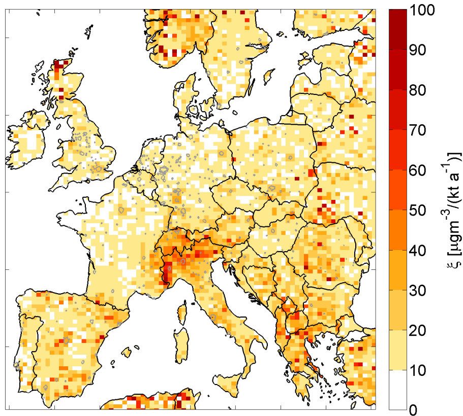
Fig. 2. Regression coefficient \xi relating \text{NO}_x emissions to concentration increments in CHIMERE.
