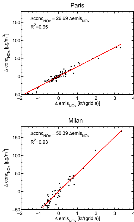
Fig. 3. \text{NO}_x emission vs. concentration increments in two major European cities: Paris (top panel) and Milan (bottom panel) in the CHIMERE model run. Each dot represents a grid cell. All EMEP grid cells which contain parts of the urban area are combined here. The linear fit is shown as red line. Note the different slopes of the fit, corresponding to the different meteorological characteristics of these cities.
