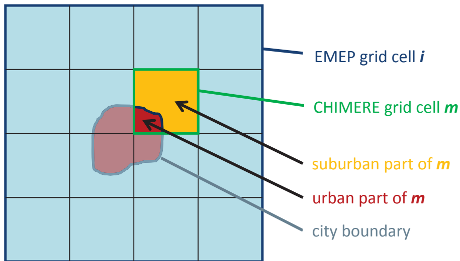
Fig. 4. Disaggregation of CHIMERE grid cell m into urban (red) and suburban (yellow) part.
