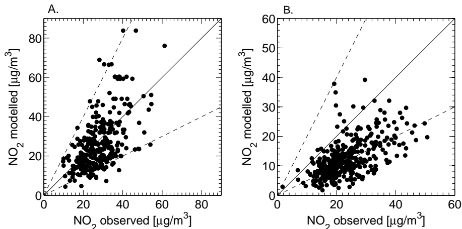
Fig. 6. Comparison of modelled (explained) vs. observed \text{NO}_2 urban background concentrations: (A) urban background stations in cities for which an urban polygon is defined, (B) urban background stations in cities for which no urban polygon is defined ( 7 \times 7 km grid value is taken here).
