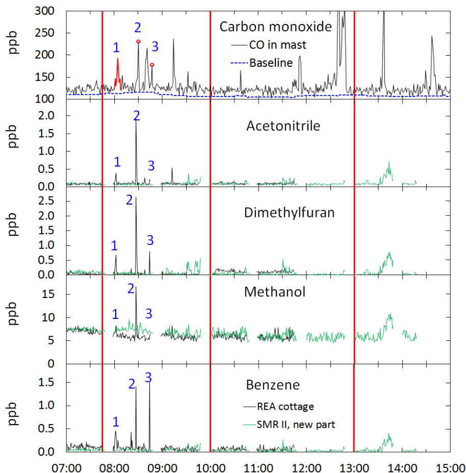
Fig. 10. Data of selected VOCs measured with PTR-MS and carbon monoxide measured in the mast at all altitudes. The numbers on the peaks and the red line for CO in peak 1 denote the data that that were used for the regressions in Fig. 10 and Table 3.
