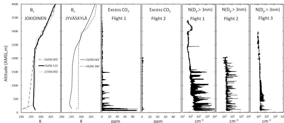
Fig. 12. Vertical profiles of virtual potential temperature ( \theta_v ), excess \text{CO}_2 and particle number concentrations during the experiment day. For flight 3 no excess \text{CO}_2 data are shown because they did not deviate from zero. The \theta_v data are from meteorological soundings from two sites, the Jokioinen observatory and the Tikkakoski airport in Jyväskylä.
