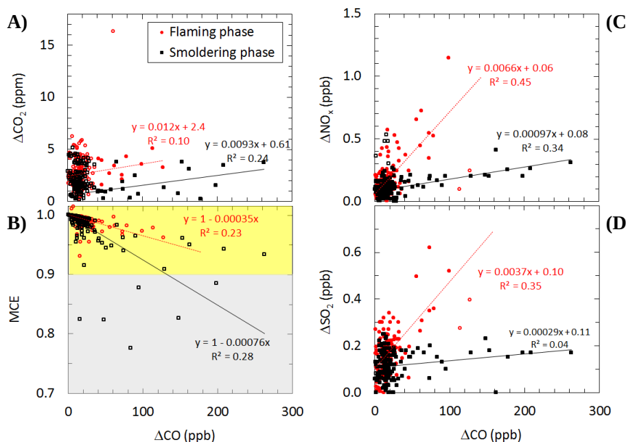
Fig. 5. Relationships of trace gases measured from the SMEAR II mast during the flaming and smoldering phases. Left: (A) excess \text{CO}_2 and (B) modified combustion efficiency as a function of excess CO concentration, right: (C) excess \text{NO}_x and (D) excess \text{SO}_2 concentrations as a function of excess CO concentration. The yellow shading in the low left panel denotes the range of MCE values where more than 50 % of combustion can be assumed to be flaming and the grey shading the range of MCE values where more than 50 % of combustion can be assumed to be smoldering.
