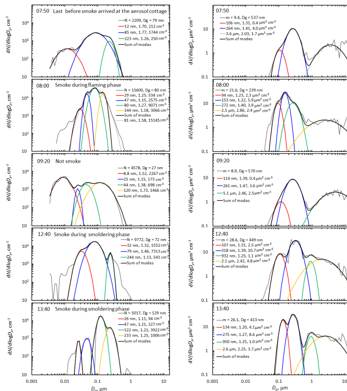
Fig. 7. Selected particle size distributions measured with DMPS and APS in the aerosol cottage. The left column: number size distributions, right column: volume size distributions. In each plot the grey line represents the measured size distribution and the associated numbers the number concentration in \text{cm}^{-3} (left column), the mass concentration integrated to 10\text{ }\mu\text{m} in \mu\text{g m}^{-3} calculated assuming a density of 1.5\text{ g cm}^{-3} , (right column), and the geometric mean diameter ( D_g ) of the whole size distribution. The modal parameters are the geometric mean diameter, the geometric standard deviation, and the number or volume concentration of the mode.
