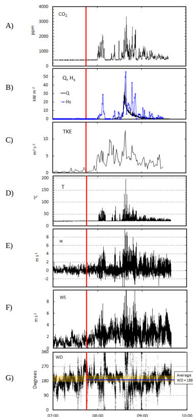
Fig. 3. Observations within the burning area during the flaming phase. (A) \text{CO}_2 concentrations, (B) heat flux ( Q ), turbulent sensible heat flux ( H_s ), (C) turbulent kinetic energy (TKE), (D) temperature ( T ), and (E) vertical flow velocity ( w ), (F) horizontal wind speed (WS), and (G) wind direction (WD) at 12 m altitude. The 3-D wind data are at 10 Hz, the others at 1 Hz time resolution. The red line shows the ignition time at 07:45. The yellow shading indicates the wind direction sector that would bring smoke from the fire to SMEAR II.
