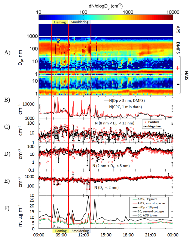
Fig. 6. Data of selected ground-based aerosol measurements at SMEAR II on 26 June 2009. (A) Particle number size distributions measured with the APS and the DMPS, and the positive and negative air ion size distributions measured with the NAIS, (B) total particle number concentrations measured with a CPC and integrated from the DMPS, (C–E) air ion number concentrations from the NAIS data in three different size ranges and (E) concentrations of organics and the sum of all compounds measured with an AMS, mass concentration of particles smaller than 10 \mu\text{m} using the density of 1.5 \text{ g cm}^{-3} , and black carbon concentration at two locations.
