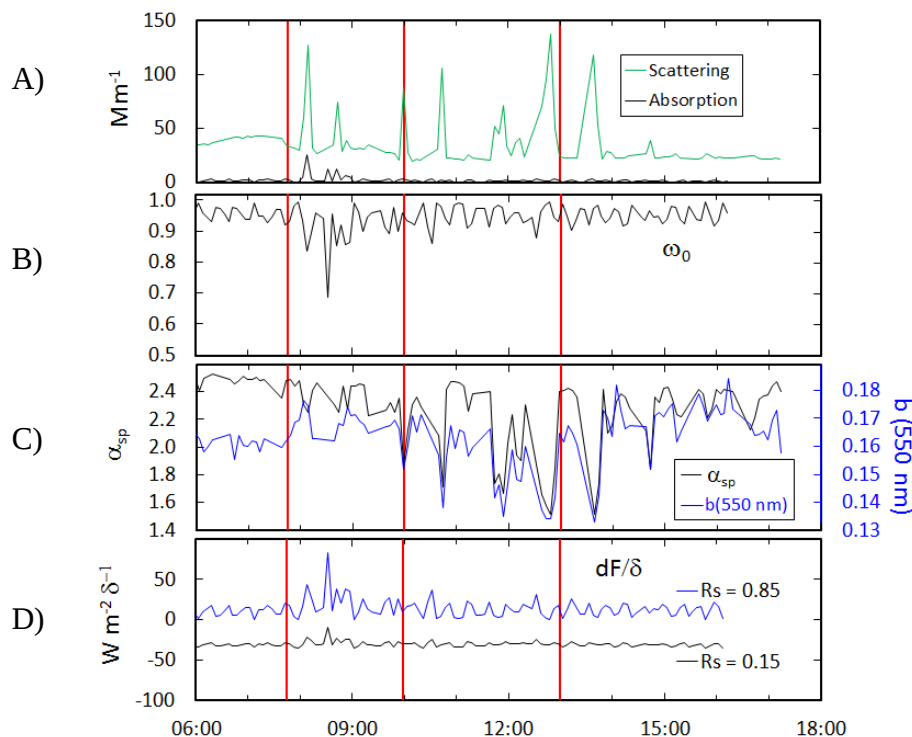
Fig. 8. Optical properties of aerosol observed in the aerosol cottage. (A) scattering and absorption coefficients at \lambda = 550 nm, (B) single-scattering albedo at \lambda = 550 nm, (C) Ångström exponent of scattering over 450–700 nm ( \alpha_{sp} ) and backscatter fraction ( b ) at \lambda = 550 nm; (D) intrinsic aerosol forcing efficiency for two surface reflectances ( R_s ).
