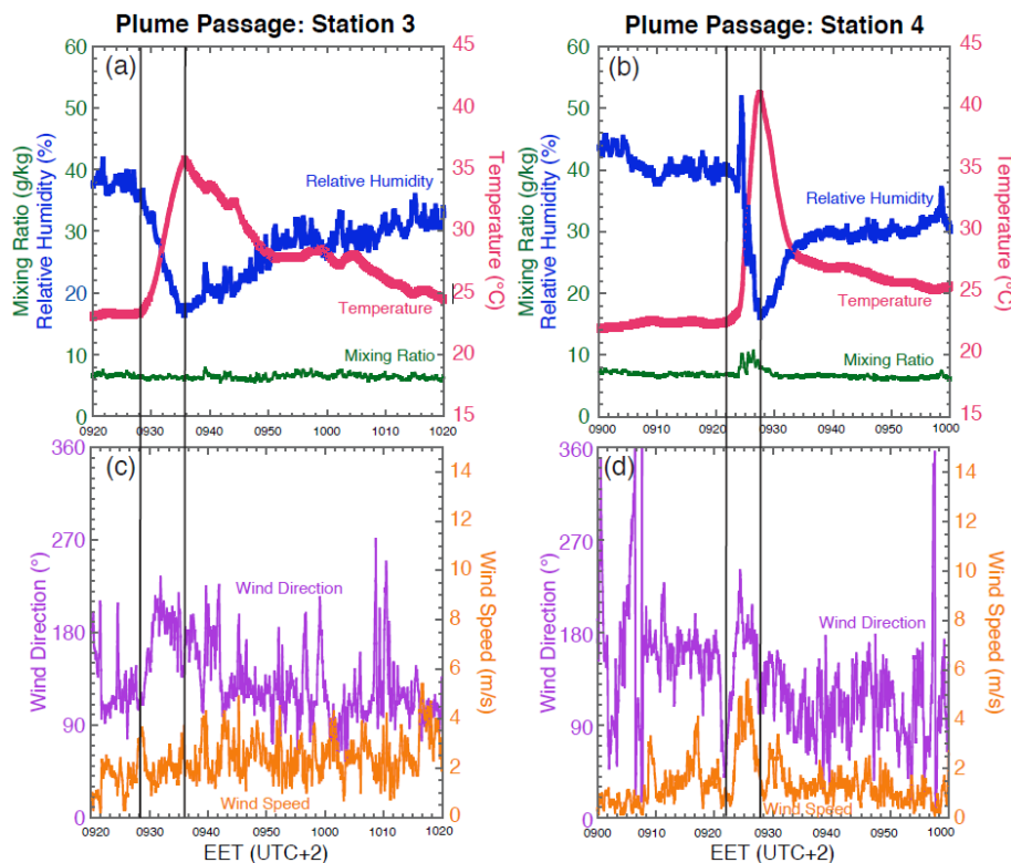
Fig. 4. Observations on top of two meteorological stations outside of the perimeter of the burning area.
