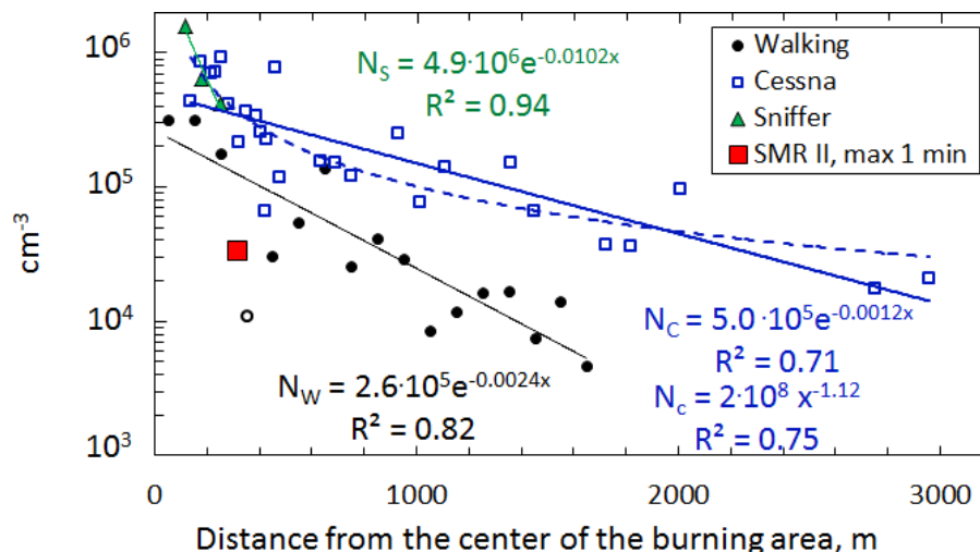
Fig. 14. Particle number concentration as a function of 3-dimensional distance from the center of the burning area measured in the Cessna, with the portable CPCs on ground (walking, N_W ), in the aeroplane (Cessna, N_C ), and on ground in the van ( Sniffer , N_S ). The walking data points are the maximum concentrations of each 100 m distance bin, the aircraft data points are the maxima in each plume passage and the Sniffer data points the 3–5 min average concentrations measured at three standing locations of the van. The SMR II data point denotes the maximum 1 min particle number concentration in the aerosol cottage during the experiment. The solid lines denote fittings of the exponential function N_0 e^{-kx} and the dashed line the fitting of a power law N_0 x^{-b} and where x is the distance from the center of the burn area.
