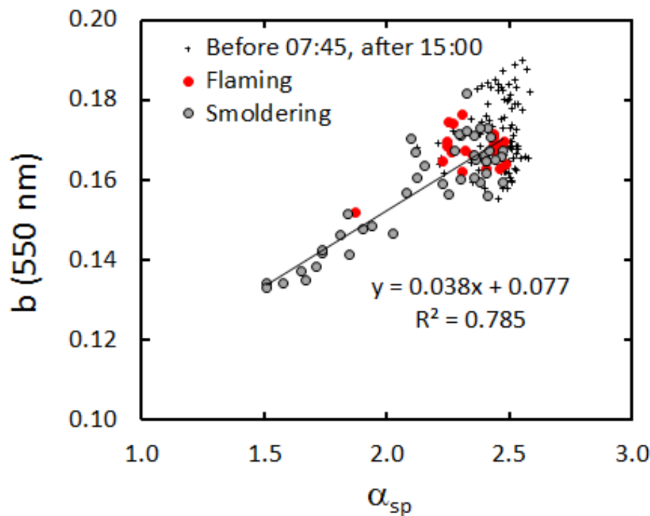
Fig. 9. Backscatter fraction ( b ) at \lambda = 550 \text{ nm} vs. Ångström exponent of scattering ( \alpha_{sp} ) in the aerosol cottage before the flaming phase and after the last plume was observed (crosses), during the flaming phase (red circles), and during the smoldering phase (grey circles). The regression line was fitted with the smoldering-phase data.
