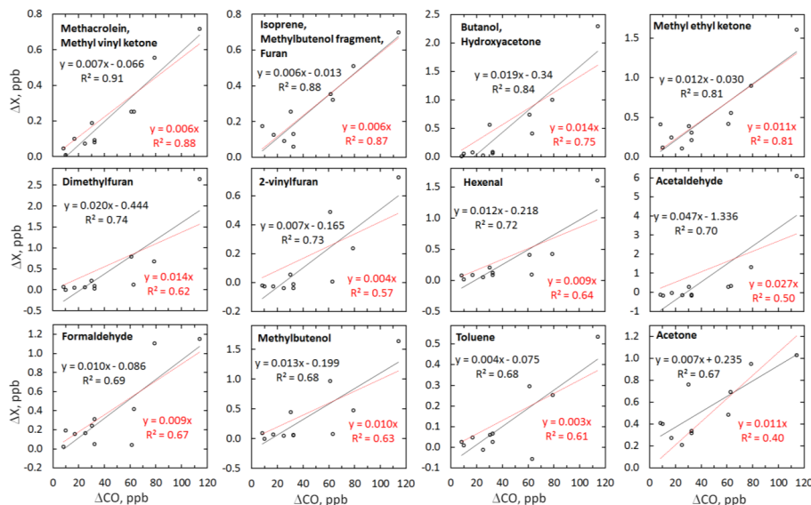
Fig. 11. Relationships of excess concentrations ( \Delta X ) of organic trace gases to excess carbon monoxide ( \Delta CO ) concentrations in the smoke plume peaks presented in Fig. 9. The black lines and formulas denote linear regressions without forcing the offset to zero and the red lines and formulas linear regressions with forcing the offset to zero.
