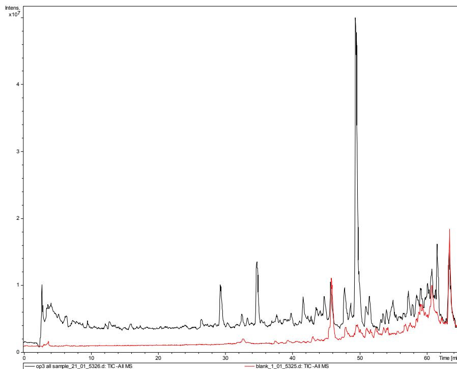
Fig. 1. Total ion chromatograms for LC-MS analysis in negative ionisation mode. Black: OP3_all extract from filters collected at the Bukit Atur site, Borneo. Red: blank control sample. Many of the peaks after 45 min are contaminants from the methanol used in the LC analysis.
