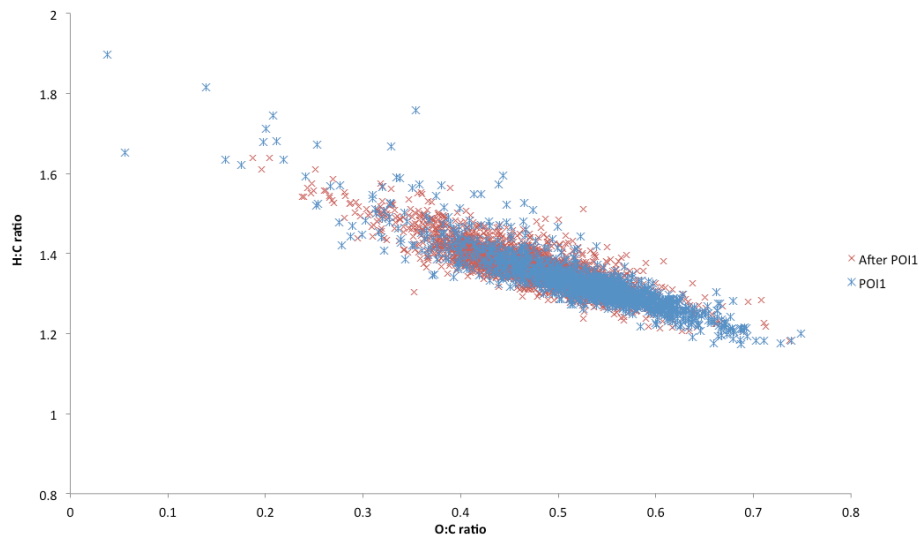
Fig. 3. Van Krevelen plot of 10 min average O : C and H : C ratios determined using HR-AMS. Blue crosses indicate ratios measured during a period of increased biomass burning influence (POI1). Red crosses indicate the measurements taken after POI1 when lower pollution levels were seen.
