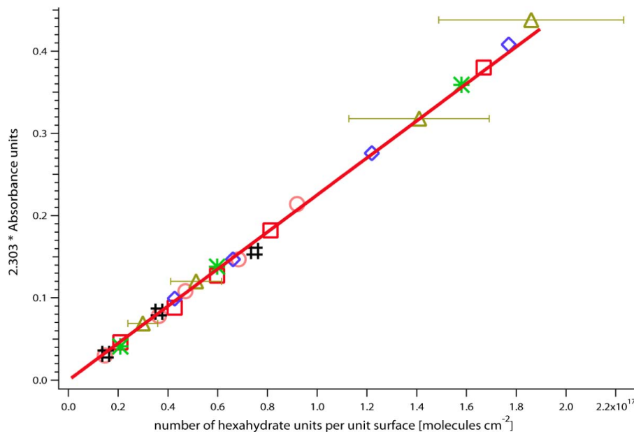
Fig. 3. Plot of the IR absorbance at 3426\text{ cm}^{-1} as a function of the number of formula units per unit surface for pure HCl hexahydrate ( \text{HCl}\cdot 6\text{H}_2\text{O} ). The different symbols represent the six different samples listed in Table 4. From the fit one obtains a cross section of \sigma = (2.3 \pm 0.7)10^{-18}\text{ cm}^2\text{ molec}^{-1} per HCl hexahydrate formula unit.
