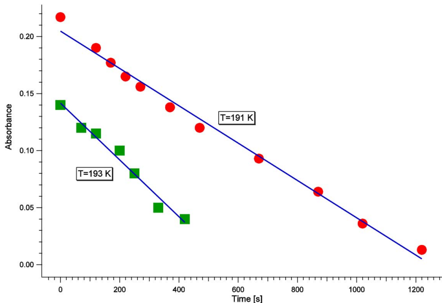
Fig. 4. Rate of decrease of IR absorbance at 3426\text{ cm}^{-1} of a pure HCl·6H 2 O sample during evaporation under SFR conditions at T = 191 and 193 \pm 1\text{ K} , displayed as a function of time. See also Fig. 2.
