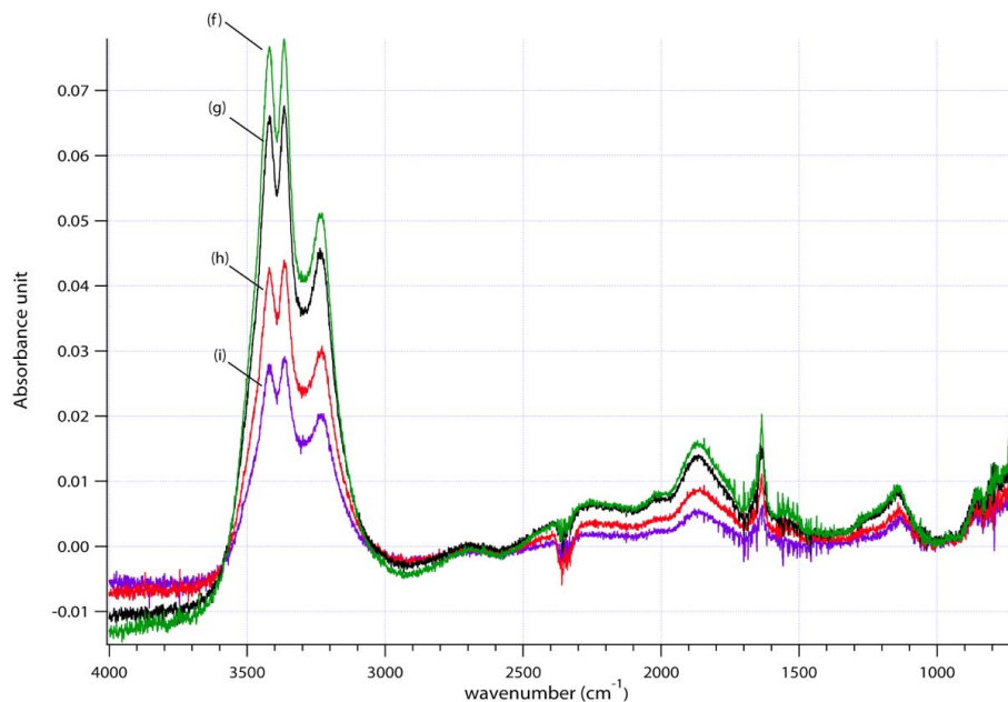
Fig. 2. IR spectra of the same ice/HCl film shown in Fig. 1 at successive stages during evaporation for 20 min. evaporation, at T = 187 \pm 0.5\text{K} under SFR conditions. No offset has been introduced.
