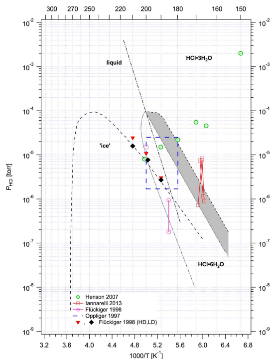
Fig. 12. Phase diagram for the binary system HCl/H 2 O. The gray area for the HCl·6H 2 O existence is an extension of the existence area proposed by Iannarelli et al. (2013), the green points from Henson et al. (2007), the red squares from Iannarelli et al. (2013), the purple points from Flückiger et al. (1998) and the blue broken rectangle from Oppliger et al. (1997). See text for discussion.
