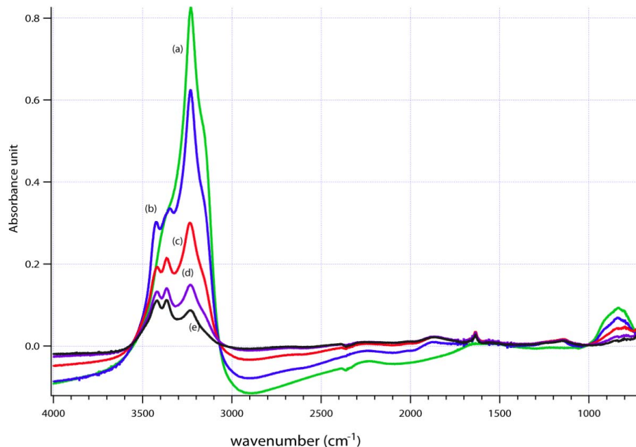
Fig. 1. IR transmission spectra of a pure ice film before (a) and after (b) doping with gaseous HCl at 170 K at a typical dose of 1 - 2 \times 10^{17} molecules. Spectra (c) , (d) and (e) have been collected in 4 scans each at 1 \text{ cm}^{-1} resolution during film evaporation at increasing temperature under SFR (stirred flow) conditions. No offset has been introduced in order to facilitate the quantitative comparison between spectra.
