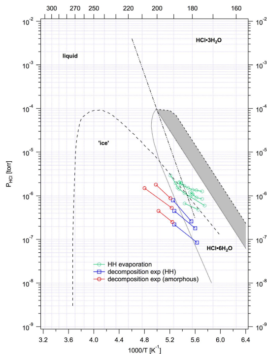
Fig. 11. Phase diagram for the binary system HCl/H 2 O. The gray area for the HCl·6H 2 O existence is an extension of the existence area proposed by Iannarelli et al. (2013). The green circles represent HH evaporation whereas the red circles (amorphous HCl/H 2 O) and blue squares (crystalline HCl·6H 2 O) represent phase transition experiments. The colored lines represent individual experiments at stirred-flow conditions. The squares indicate the presence of a crystalline HCl·6H 2 O phase, while the circles represent amorphous HCl/ice as indicated by the corresponding FTIR spectra. The juxtaposition of red circles/blue squares in the “ice” existence area corresponds to simultaneous observations of HH and amHCl/H 2 O.
