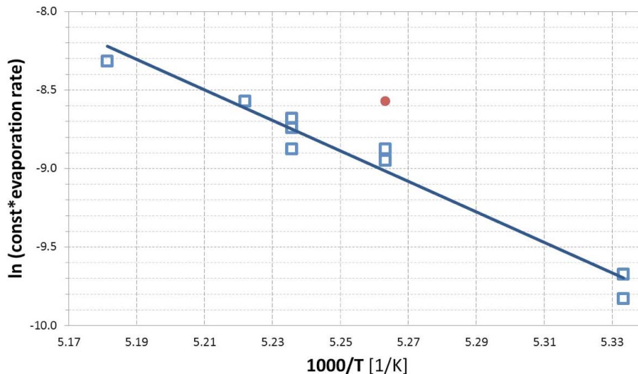
Fig. 5. Arrhenius plot of the rate of change of the IR absorption of pure HCl·6H 2 O. From the slope ( m = -9722 ), one obtains the activation energy E_a for HCl sublimation in HCl·6H 2 O of 80.8 \pm 5.8 \text{ kJ mol}^{-1} leading to \log J_{\text{ev}} \text{ molec cm}^{-2} \text{ s}^{-1} = (36.3 \pm 3.2) - (80.8 \pm 5.8)/2.303RT ; R = 8.312 \text{ J K}^{-1} \text{ mol}^{-1} without taking into account the outlier (red circle). The evaporation rate of HCl has been multiplied by \log(e) \sigma(3426 \text{ cm}^{-1}) = 1.0 \times 10^{20} \text{ cm}^2 \text{ molec}^{-1} (ordinate).
