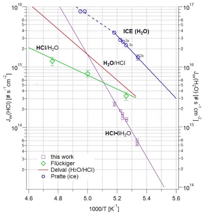
Fig. 7. HCl (left ordinate, bold HCl in plot) and H 2 O (right ordinate, bold H 2 O in plot) evaporation rates as a function of 1/T of: HCl·6H 2 O (this work, decay monitored using FTIR absorption of HCl·6H 2 O, purple line), HCl/H 2 O (Flückiger et al., 1998, green line), H 2 O/HCl (Delval et al., 2003, red line) and pure H 2 O ice (Pratte et al., 2006, blue line). The green and purple lines correspond to \log J_{\text{ev}}(\text{HCl}) \text{ molec}^{-1} \text{ cm}^{-2} \text{ s}^{-1} = (20.6 \pm 2.1) - (21\,967 \pm 4800)/2.303RT , and \log J_{\text{ev}}(\text{H}_2\text{O}) \text{ molec}^{-1} \text{ cm}^{-2} \text{ s}^{-1} = (36.34 \pm 3.20) - (80\,810 \pm 5800)/2.303RT , R = 8.312 \text{ J K}^{-1} \text{ mol}^{-1} , respectively.
