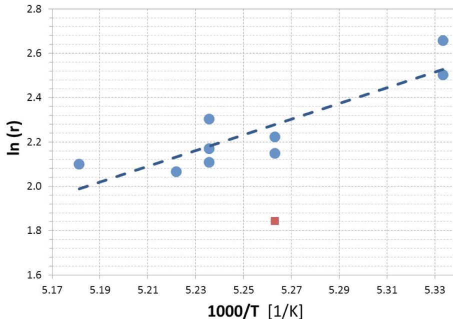
Fig. 6. Arrhenius plot of r corresponding to r = J_{\text{ev}}^{\text{net}}(\text{H}_2\text{O})/J_{\text{ev}}(\text{HCl}\cdot 6\text{H}_2\text{O}) leading to a slope of 3544.7 corresponding to E_{\text{a}}^{\text{sub}}(\text{H}_2\text{O}) - E_{\text{a}}^{\text{sub}}(\text{HCl}\cdot 6\text{H}_2\text{O}) = -29.5 \pm 9.6 \text{ kJ mol}^{-1} . The slope has been evaluated without taking into account the outlier (red square).
