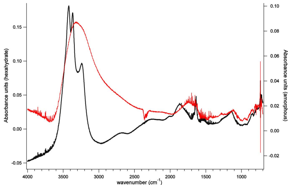
Fig. 10. IR spectrum of an initial \text{HCl} \cdot 6\text{H}_2\text{O} film generated at 170 K using a dose leading to 8 \times 10^{16} molecules of adsorbed HCl. The HH film was heated to 192 K (black trace) and subsequently to 200 K (red trace). This experiment was performed under static conditions.
