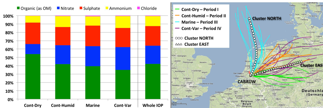
Fig. 1. Average PM 1 -filters chemical composition and back-trajectory analysis for the four periods of the campaign. Organics are reported as total organic matter (OM) calculated by relationship OM = OC_{PM_1\text{filters}} \cdot 1.6 .
