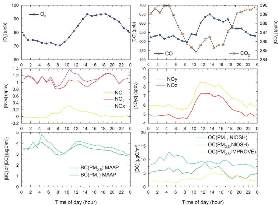
Fig. 6. Average diurnal variations in O 3 , CO, CO 2 , NO, NO 2 , NO x , NO y , NO z , BC, and OC concentrations during the MTX2006 campaign.
