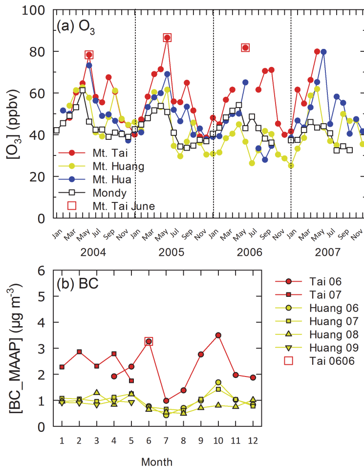
Fig. 5. Year-round observations of (a) O 3 and (b) BC at Mt. Tai and other mountain sites. Data for Mt. Tai in June are surrounded by squares.
