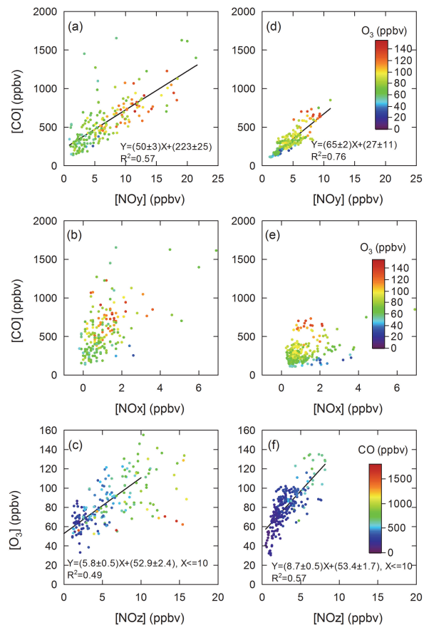
Fig. 4. Observed correlations between (a) NO y and CO concentrations, (b) NO x and CO concentrations, and (c) NO z and O 3 concentrations. Symbols are colored by O 3 concentrations for (a) and (b) , and by CO concentrations for (d)–(f) same as (a)–(c) but using modeled concentrations.
