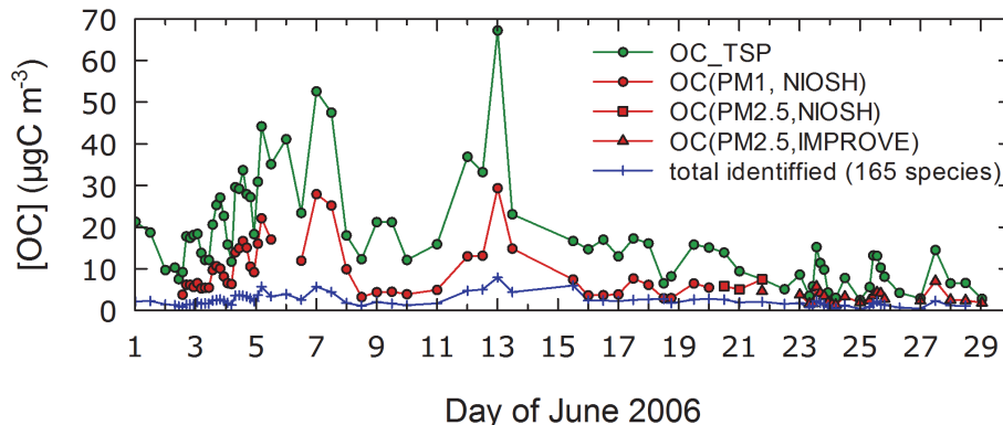
Fig. 11. Time series of OC concentrations measured for TSP filter samples (green) and size-segregated OC concentrations (PM 1 and PM 2.5 ) measured using a semi-continuous ECOC analyzer (red). The sum of molecularly identified OCs (165 species) for TSP samples is shown in blue. The time intervals of the TSP samplings are used in all cases
