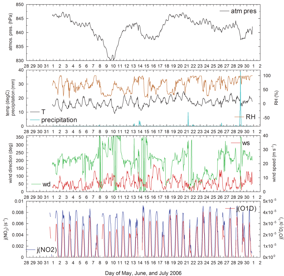
Fig. 2. Time series of atmospheric pressure, temperature, RH, precipitation, wind direction and speed, J(\text{NO}_2) and J(\text{O}^1\text{D}) values.
