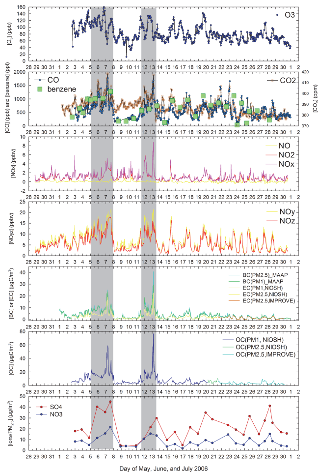
Fig. 3. Overall time series of O_3 , CO, benzene, CO_2 , NO, NO_2 , NO_x , NO_y , NO_z , BC, OC, sulfate and nitrate. Hatched areas indicate two episodes with strong influences from OCRB.
