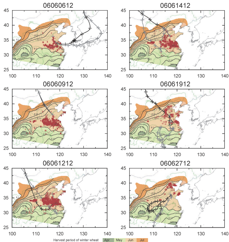
Fig. 8. Backward trajectories with starting altitudes of 1500 m (black) and 750 m (gray) at six different times (YYMMDDHH in LT, shown above individual panels). Plus marks indicate the locations of air mass every 12 h. Hotspots detected by satellite sensors during the 5 preceding days are shown in red (numbers indicate the detection day in June). Harvest areas of winter wheat in different months are shown by colored areas.
