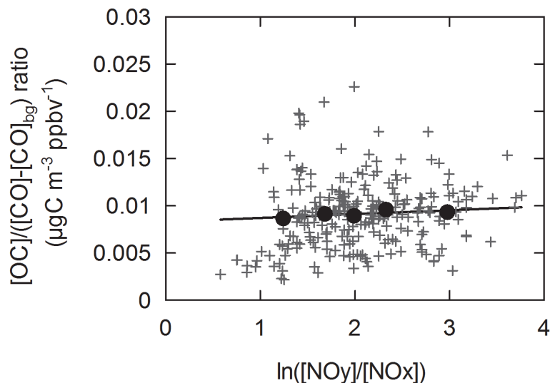
Fig. 10. \Delta[\text{OC}]/\Delta[\text{CO}] ratio during the latter period of the campaign (from 16 June 2006) without influence from biomass burning and increasing air mass age, indicated by \ln([\text{NO}_y]/[\text{NO}_x]) . The CO background concentration, [\text{CO}]_{\text{bg}} was assumed to be 90 ppbv.
