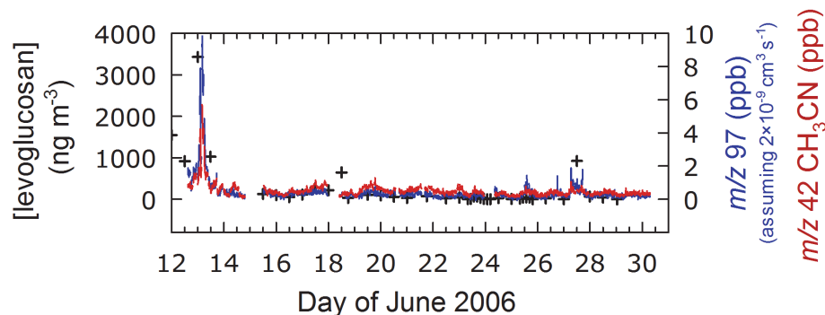
Fig. 9. Correlations between levoglucosan concentrations from TSP filter samples (plus marks) and m/z 97 and m/z 42 ( \text{CH}_3\text{CN} ) signals (colored solid lines) derived from continuous PTR-MS measurements.
