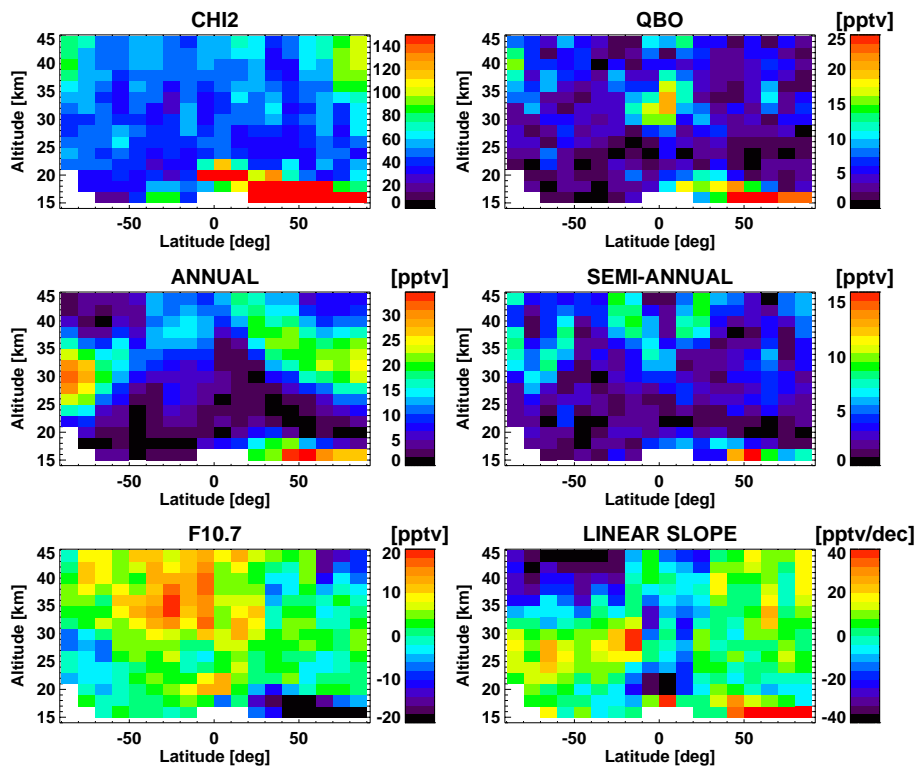
Fig. 14. Global overview of the fit RMS (top left), the amplitudes of various fit parameters and the linear trends (bottom right). For “QBO” and “ F_{10.7} ”, the amplitude is defined as the semi-difference between maximum and minimum of the fitted time series of Singapore winds and solar F_{10.7} flux, respectively. For “ F_{10.7} ” the sign indicates a positive or negative correlation with the solar cycle.
