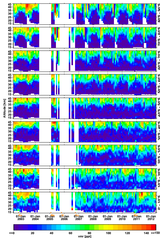
Fig. 4. Time series of color-coded \text{SO}_2 monthly mean volume mixing ratio profiles for 10^\circ latitude bins in the Southern Hemisphere. The color scale is restricted to 0–150 pptv: negative and values larger than 150 pptv are given the color belonging to 0 and 150 pptv, respectively. Major volcanic eruptions are indicated within the latitude bin of their location (see Table 2).
