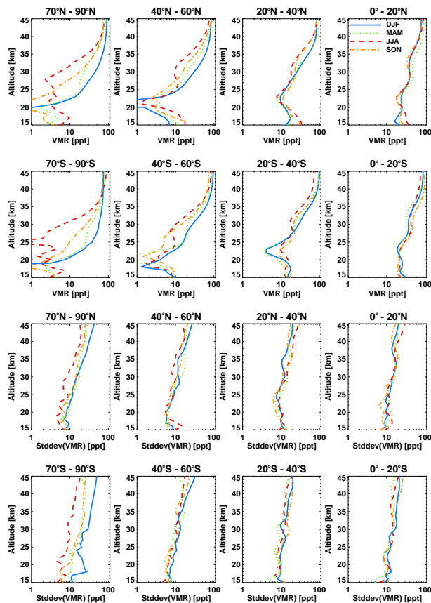
Fig. 7. Mean background seasonal profiles of \text{SO}_2 (top two rows) and standard deviation of the distribution (bottom two rows). Periods of major volcanic influence which have been excluded here are: October–December 2002, July 2003, January–June 2005, May–November 2006, October 2007, July–December 2008, June–December 2009, November–December 2010, July–September 2011.
