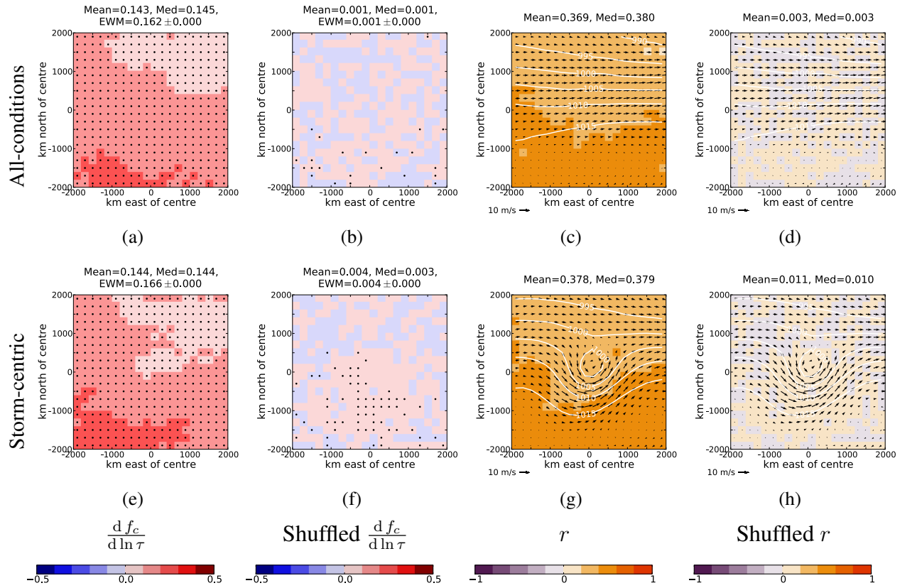
Figure S2. Similar to Figure 3 but for lin-log fits of cloud fraction ( f_c ) versus aerosol optical depth ( \tau ) over the South Atlantic ocean.
