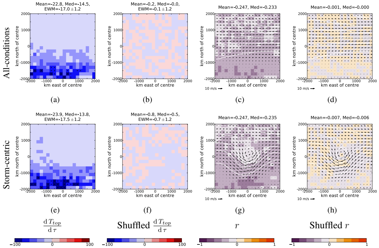
Figure S3. Similar to Figure 5, but for lin-lin fits of cloud top temperature ( T_{top} ) versus aerosol optical depth ( \tau ) over the South Atlantic ocean.
