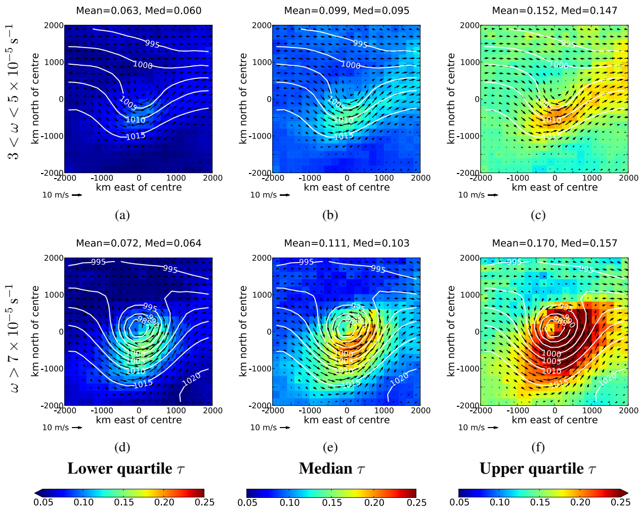
Figure S1. Similar to Figure 1, but for Aqua-MODIS aerosol optical depth ( \tau ) over the South Atlantic ocean.
