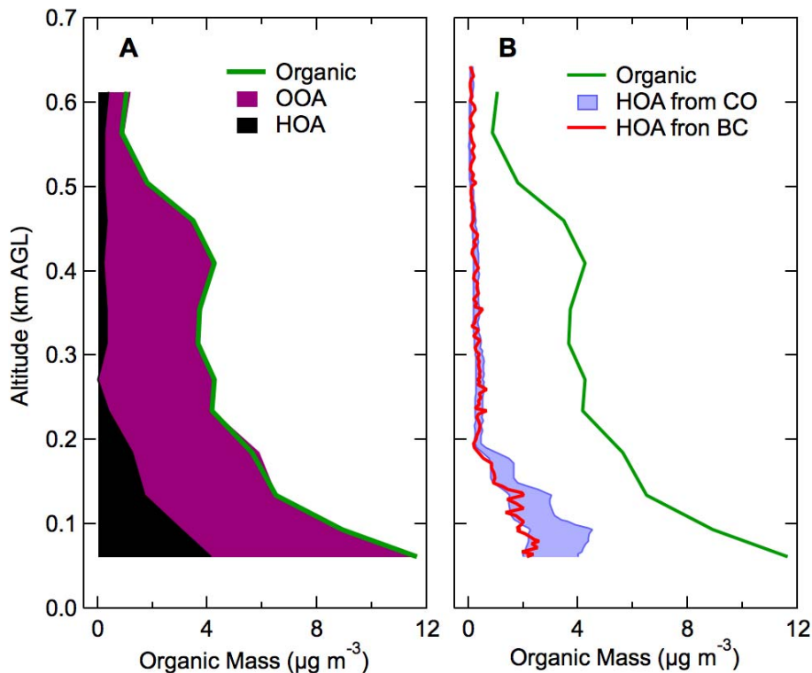
Fig. 14. Vertical profile from descent to Lone Star airfield on 12 October showing: (A) organic mass loading in comparison to OOA and HOA derived from the AMS; (B) organic mass loading compared to HOA derived from a parameterization against CO and black carbon (BC) (see text).
