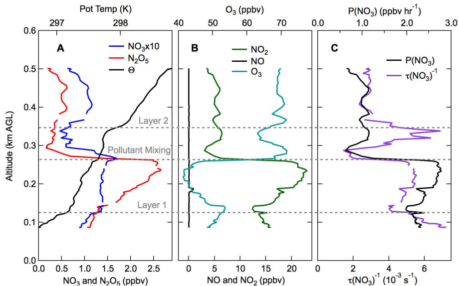
Fig. 3. Vertical profiles of: (A) mixing ratios of \text{NO}_3 ( \times 10 to make it visible) and \text{N}_2\text{O}_5 (bottom axis) and potential temperature (top axis); (B) mixing ratios of \text{NO} and \text{NO}_2 (bottom axis) and \text{O}_3 (top axis); (C) \text{NO}_3 reactivity, measured as \tau(\text{NO}_3)^{-1} (bottom axis), and production rate, P(\text{NO}_3) (top axis). Data are for descent to Hooks on 8 October, 9:33 p.m. local time. Grey dashed lines and labels indicate altitudes of layers in the potential temperature profile and in the observed mixing of pollutants (see text).
