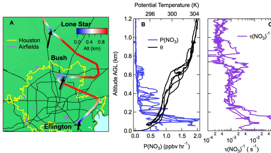
Fig. 10. Same as Fig. 2 except for the latter portion of the P-3 flight track on 11–12 October. Note that \tau(\text{NO}_3)^{-1} in panel (C) is on a logarithmic scale to show the contrast between its large increase in the lowest layer and its small values at high altitude.
