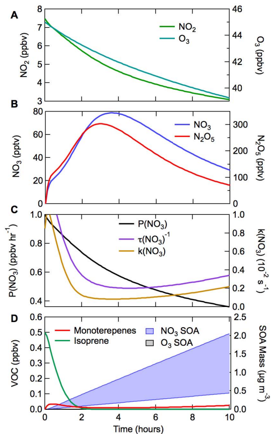
Fig. 18. Same as Fig. 17, except for smaller nitrate radical and BVOC emission rates intended to represent biogenic VOC oxidation over the urban area (see text).
