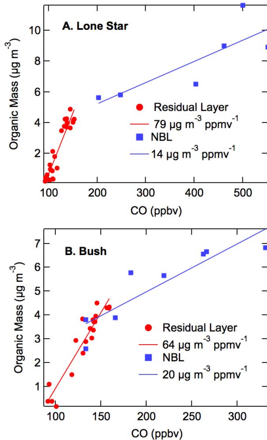
Fig. 15. Plot of organic aerosol mass ( \mu\text{g m}^{-3} ) from the AMS against carbon monoxide (CO) in ppbv for the profiles at (A) Lone Star and (B) Bush airfields on 12 October. Red and blue data points are for the residual and nocturnal boundary layers, respectively. Slopes of linear fits to each data set are shown in the caption.
