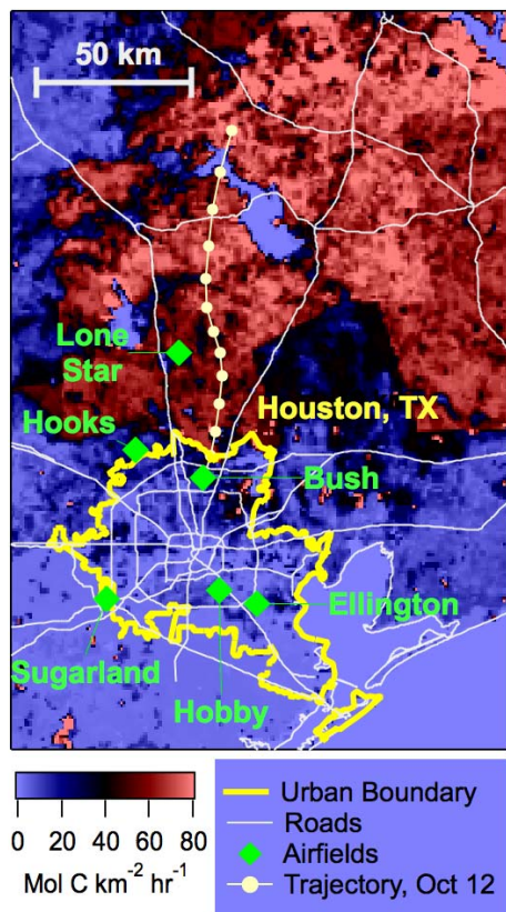
Fig. 1. Map of the Houston, TX area showing the location of airfields, major roadways (white lines) and monoterpane emission potential (blue-red color scale, legend below) from the BEIS3 inventory. The line with circles is a twelve-hour forward trajectory from Bush airfield on the north side of Houston beginning at sunset on 12 October (see text).
