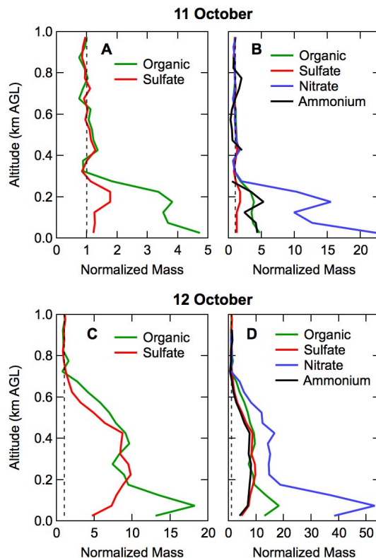
Fig. 16. Normalized mass loading of aerosol organic, sulfate, nitrate and ammonium from the average of 5 vertical profiles between midnight and 1 a.m. on 11 October ( A, B ) and 12 October ( C, D ). Mass loadings are averaged into 50 m bins and normalized to the value above the boundary layer (400–1000 m on 11 October, 700–1000 m on 12 October) to show relative enhancements as a function of decreasing height for each flight.
