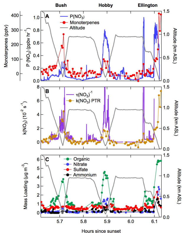
Fig. 6. Time series (plotted as hours since sunset) from five vertical profiles between midnight and 1 a.m. local time on 11 October showing (A) . Nitrate radical production rate, P(\text{NO}_3) (left axis), monoterpene mixing ratio (far left axis) and aircraft altitude (right axis); (B) inverse \text{NO}_3 lifetime, \tau(\text{NO}_3)^{-1} , and first-order \text{NO}_3 loss rate coefficient, k(\text{NO}_3) from PTRMS measurements of biogenic VOCs (see text), plotted together against the left axis; (C) mass loading of aerosol organic, nitrate, sulfate and ammonium from the AMS. Aircraft altitude is plotted against the right axis for reference in (B) and (C) .
