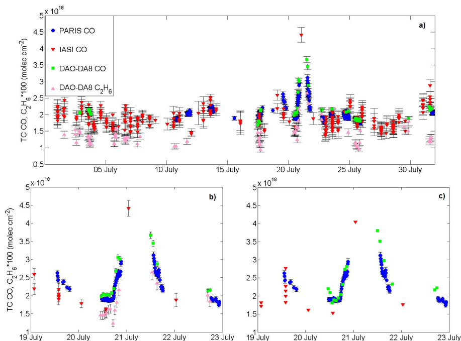
Fig. 2. The total column measurements (TC) in Halifax are shown for CO and C 2 H 6 for (a) July 2011, (b) between 19 and 23 July 2011 and (c) CO total columns of DAO-DA8 and IASI smoothed with the PARIS-IR averaging kernel. PARIS-IR (blue dots), IASI (red inverted triangles), DAO-DA8 (green squares) total columns for CO, and DAO-DA8 total columns for C 2 H 6 (pink triangles) are shown. The labels on the x-axes indicate the start of each day at 00:00 UTC. Note that the C 2 H 6 columns are scaled by a factor of 100 in panels (a) and (b) . The black bars indicate the estimated uncertainties for each gas and instrument, as described in Table 1 and Sect. 2.4.
