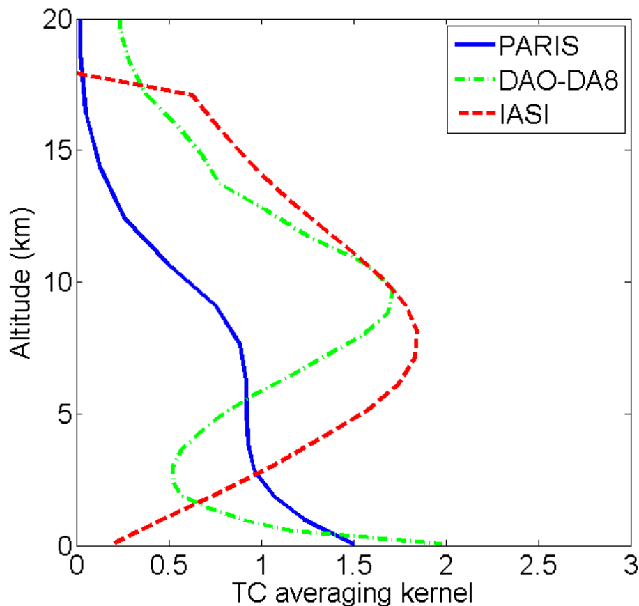
Fig. 1. Typical total column (TC) averaging kernels for CO for PARIS-IR (solid blue line), DA8 (dot-dashed green line) and IASI during a morning overpass (dashed red line).
