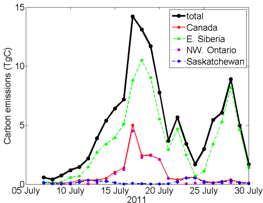
Fig. 4. Daily distribution of carbon emissions from the FLAMBE inventory, based on fire information from MODIS and GOES, is shown. The traces show the daily total carbon emitted from all boreal fire regions ( \geq 50^\circ N; thick black line), for all of Canada ( 50^\circ – 75^\circ N, 170^\circ – 50^\circ W; thin red line), Northwestern Ontario ( 50^\circ – 55^\circ N, 95^\circ – 80^\circ W; dotted purple line), Saskatchewan ( 55^\circ – 65^\circ N, 120^\circ – 105^\circ W; dot-dashed blue line), and Eastern Siberia ( 50^\circ – 75^\circ N, 110^\circ – 179^\circ E; dashed green line).
