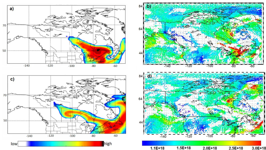
Fig. 6. FLEXPART forward-trajectories at 15:00 UTC on (a) 20 July and (c) 21 July 2011, for a constant particle release starting on 17 July 2011 at 12:00 UTC. The colour contours are on a relative scale from high (red) to low (blue) low concentrations. IASI CO total columns in \text{molec cm}^{-2} on (b) 20 July and (d) 21 July 2011 for the morning overpass (approximately 14:00 UTC).
