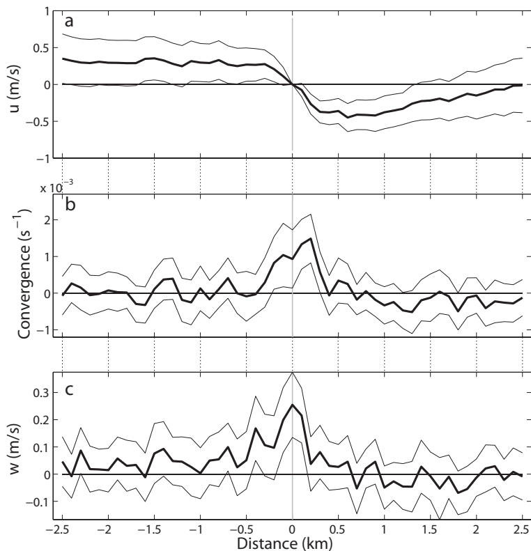
Fig. 12. Composites of dynamic measurements of (a) along-track wind speed ( u ), (b) convergence calculated from u , and (c) vertical wind speed ( w ) across 90 cold pool edges. Bold lines indicate mean values, while thinner lines indicate the 95 % confidence intervals of the mean, calculated using a standard Student t -test. For u in (a) , anomalies from the value at the cold pool edge are composited and plotted, while for convergence and w in (b) and (c) they are not.
