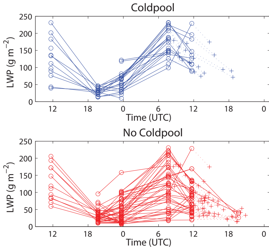
Fig. 10. 2°-box-averaged LWP of cloud field along the ECMWF-derived back trajectories flight legs with (blue) and without (red) cold pools. Averaged LWP (circles) are plotted against UTC to rid of any diurnal cycle in the data. The times of the flight legs are indicated by crosses. LWP values of the crosses are estimated by linearly interpolating satellite LWP retrievals taken before and after the flight legs.
