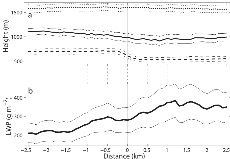
Fig. 13. Composites of cloud properties: (a) cloud top height (dotted), cloud base height (solid), and lifting condensation level (LCL; dashed); (b) cloud LWP retrieved by the GVR. The variables in (a and b) are composited without taking the anomalies in relation to the cold pool edge.
