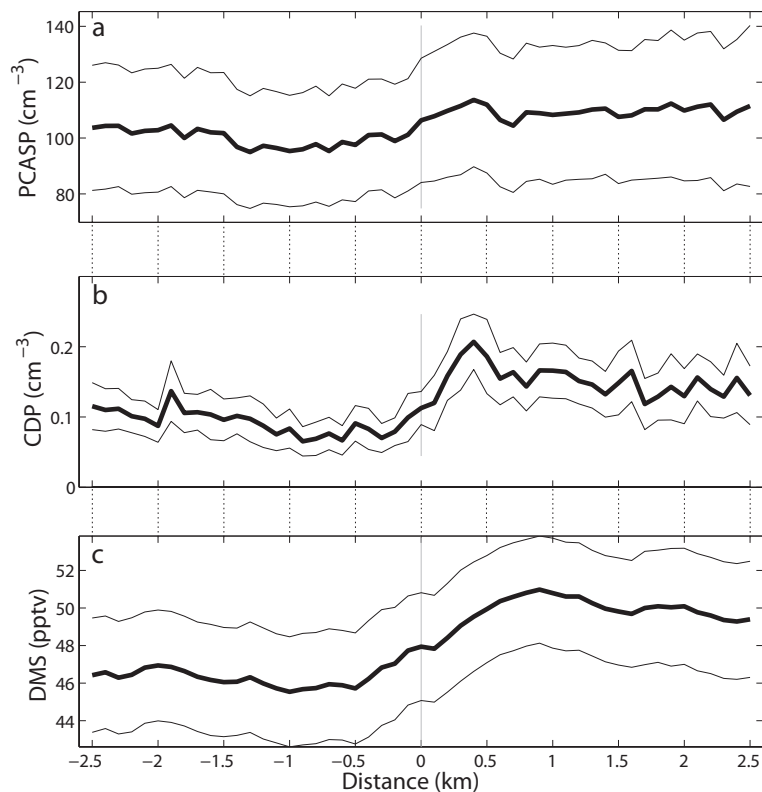
Fig. 15. Composites of (a) PCASP-measured aerosol concentration ( 0.1 \mu\text{m} < D < 3 \mu\text{m} ), (b) CDP-measured aerosol concentration ( D > 1 \mu\text{m} ), and (c) dimethyl sulfide (DMS) concentration. All variables are composited without taking the anomalies in relation to the cold pool edge.
