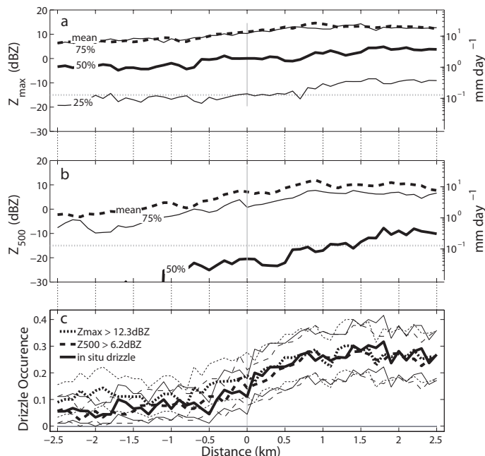
Fig. 14. Composites of (a) column maximum reflectivity ( Z_{\max} ), (b) reflectivity at 500 m ( Z_{500} ), (c) the occurrence of subcloud 98th percentile precipitation rates across the cold pool edge at each of the three different levels: at altitude of Z_{\max} (dotted), at 500 m (dashed), and at flight level (solid). For (a and b) , dotted lines indicate mean values, bold solid lines indicate median values, and thin solid lines indicate 25th and 75th percentile values. The 25th, 50th, and 75th percentile values are shown instead of the mean and the 95 % confidence intervals, since the radar reflectivity does not follow (a) Gaussian distribution. This can be easily noted from the mean reflectivity (dashed) lying far above the median value (solid bold). Previously used -15 dBZ threshold for drizzle occurrence is noted by a dotted gray line. In (c) , the mean values and the 95 % confidence interval are calculated using bootstrap resampling (Efron and Gong, 1983) of the mean occurrence over 1000 iterations.
