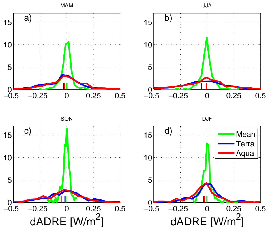
Fig. 4. Histograms of all AERONET sites on a seasonal basis: (a) MAM, (b) JJA, (c) SON, (d) DJF. Green line is ADRE difference between two AOD assumptions: with observed diurnal variability and assuming daily mean AOD. In the blue line case, AOD is taken from the observed diurnal cycle at Terra overpass time and in the red line case at Aqua overpass time. The histograms are scaled so that the area below each curve equals unity.
