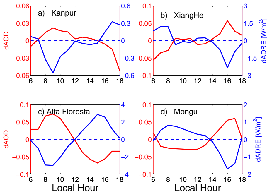
Fig. 3. As in Fig. 2, but for the following sites and seasons: (a) Kanpur, India, MAM; (b) XiangHe, China, MAM; (c) Alta Floresta, Brazil, SON; (d) Mongu, Zambia, SON.
