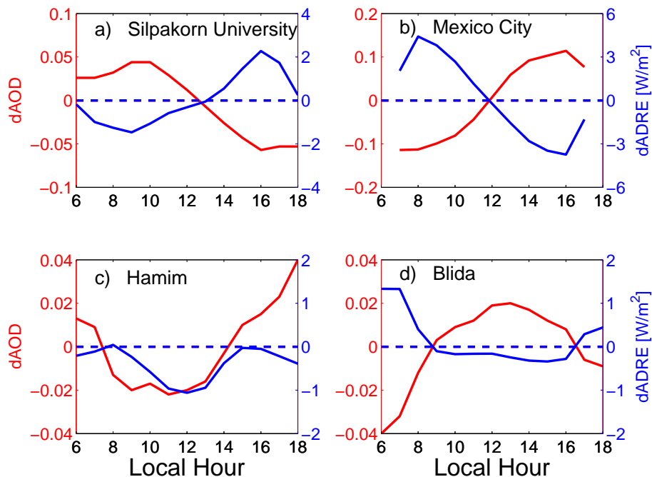
Fig. 2. Hourly AOD departures from the daily mean in red (dAOD, left side y-axis) and the instantaneous difference between two ADRE runs (assuming the observed daily AOD variability and with mean daily AOD) in blue (dADRE, right side y-axis). Same sites and seasons (and in the same order) as in the Fig. 1.
