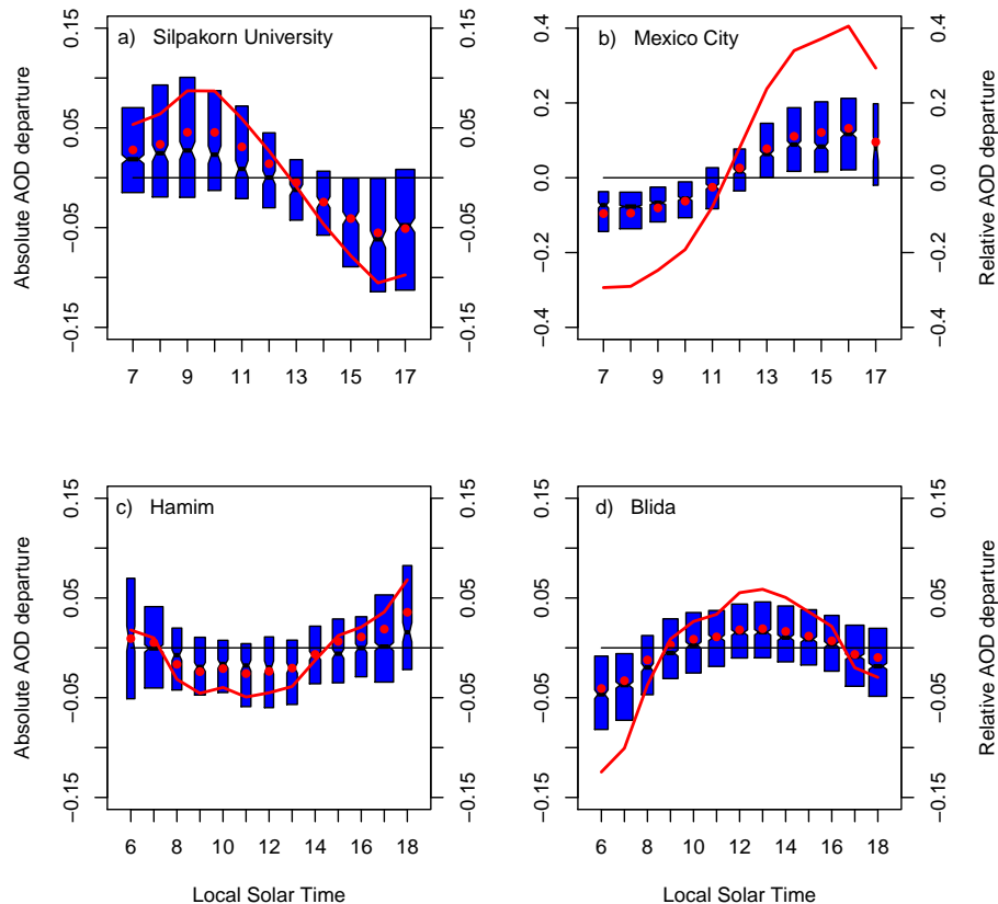
Fig. 1. AOD departures from the daily mean. Boxplots give the medians (with 5th/95th percentiles) of absolute AOD departure and the red solid points provide the mean, in addition. The red line is the relative departure in right axis; the absolute departure in each hour divided by the overall mean AOD of each season and site. The following sites and seasons are shown: (a) Silpakorn University, Thailand, MAM; (b) Mexico City, Mexico, DJF; (c) Hamim, United Arab Emirates, JJA; (d) Blida, Algeria, JJA.
