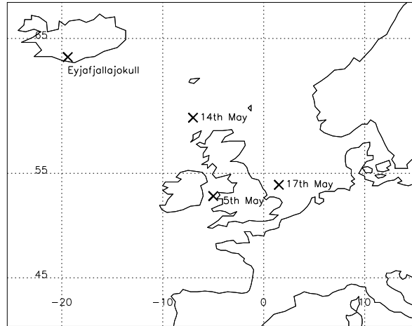
Figure 1: Location of FAAM aircraft profiles in relation to Eyjafjallajökull volcano vent.
