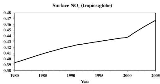
Fig S4 Ratio of tropics (30S:30N) to global surface \text{NO}_x emissions from 1980-2005 in HIST.
