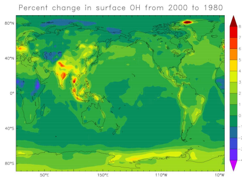
Fig S3 Global distribution of percent change in surface OH from 1980 to 2000 relative to 1980.
