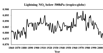
Fig. S1 Ratio of tropics (30S:30N) to global lightning NO x emissions below 500hPa in HIST.
