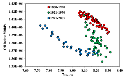
Fig. S2 Scatter plot of \tau_{\text{CH}_4, \text{OH}} versus OH below 500hPa for WMGGO3. Colored circles denote different time periods within the simulation: 1860-1920 (red), 1921-1970 (green), 1971-2005 (blue).
