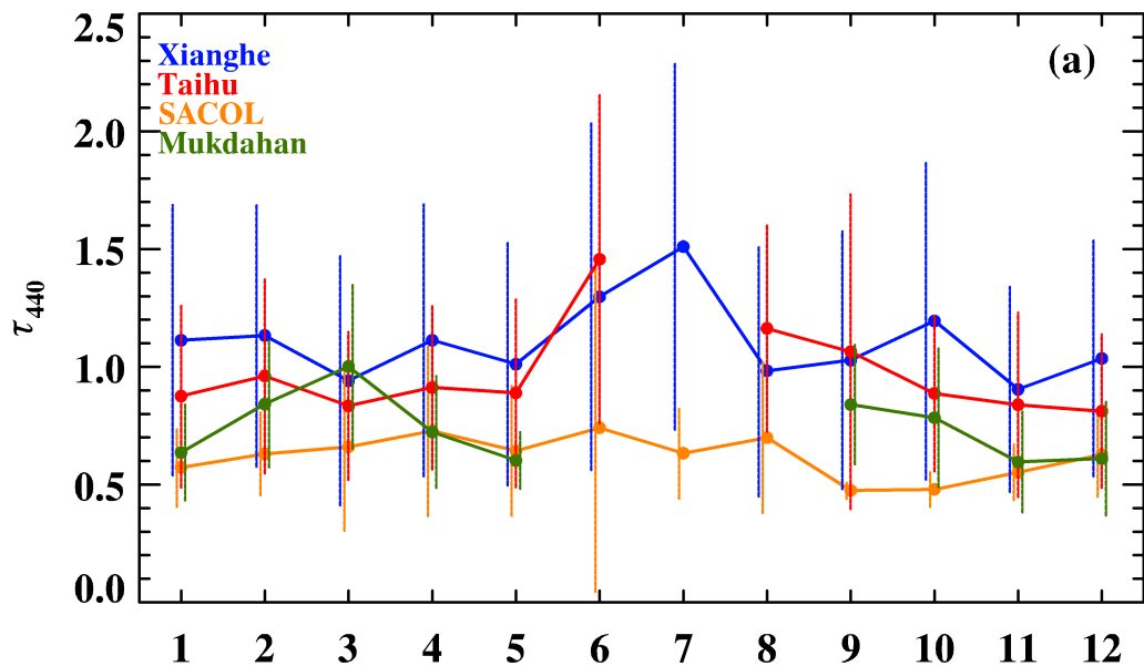
Fig. 1. Figure 4a. Aerosol optical depth at 440 nm plot with error bars denoting one standard deviation.
