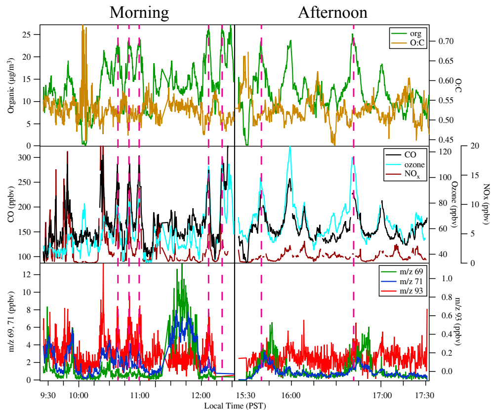
Fig. 4. Organic particle mass, organic particle O:C, CO, ozone, NO x , m/z 69 (isoprene), m/z 71 (MVK + MACR), and m/z 93 (toluene) concentrations for the morning and afternoon June 28th flights. Note there is a break in the time axis. The plume transects analyzed for Figure 5 are indicated by the dashed pink line
