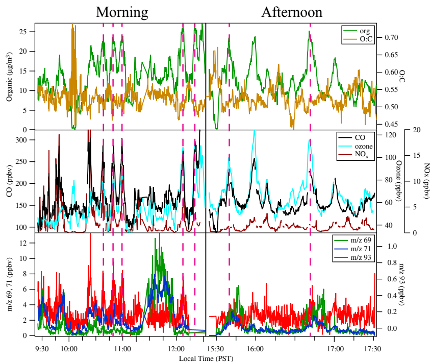
Fig. 4. Organic particle mass, organic particle O:C, CO, ozone, NO x , m/z 69 (isoprene), m/z 71 (MVK + MACR), and m/z 93 (toluene) concentrations for the morning and afternoon June 28th flights. Note there is a break in the time axis. The plume transects analyzed for Figure 5 are indicated by the dashed pink line
