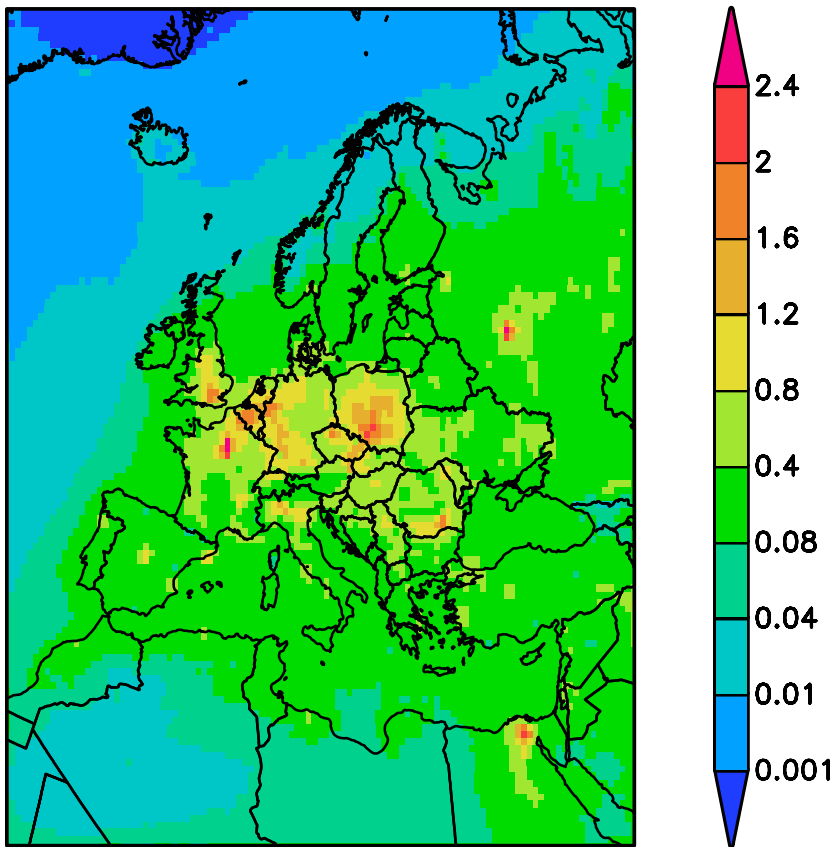
Fig. 1. Model domain and BC mean concentration ( \mu\text{g}/\text{m}^3 )
