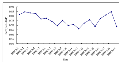
Fig. 1 Time series plot of BeP/(BaP+BeP)
