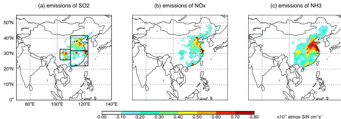
Fig. 1. Figure 1 with the correct unit: Spatial distributions of (a) SO 2 , (b) NO x and (c) NH 3 emissions from China used in 2006C simulation
