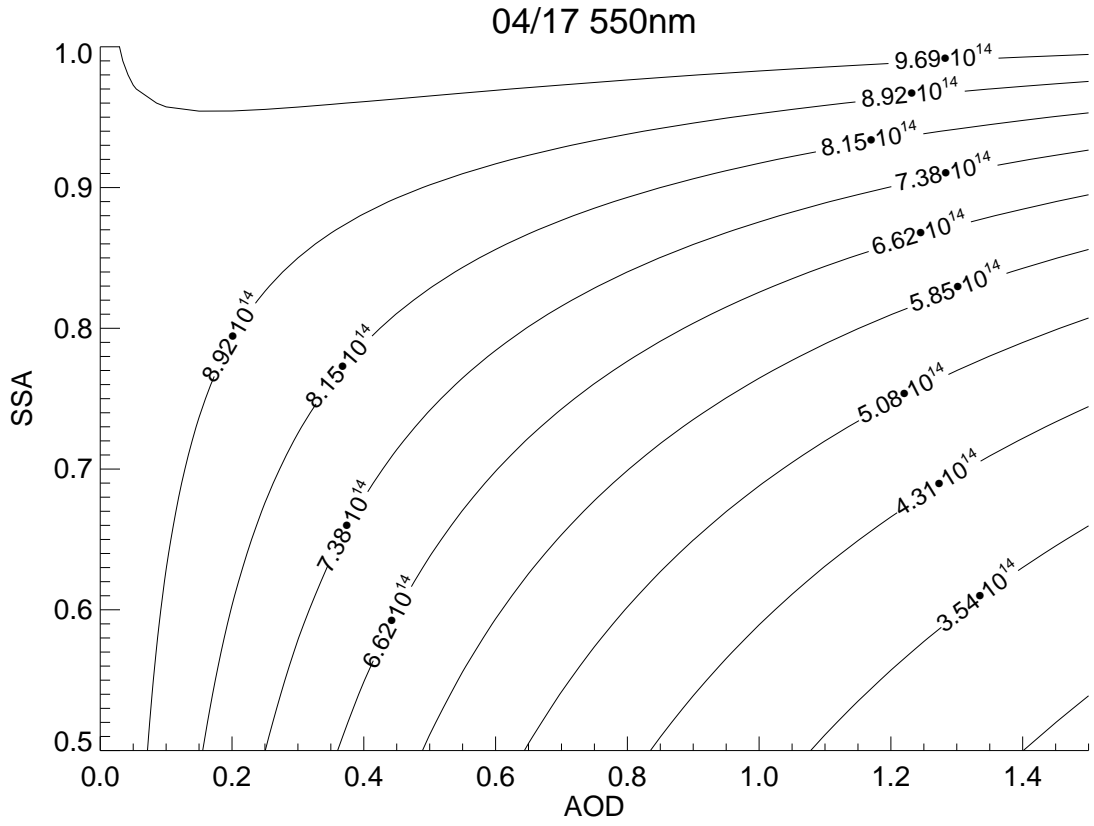
Figure 1. Actinic flux as a function of SSA and AOD.
