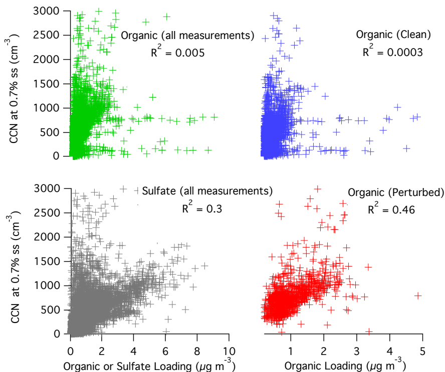
Fig. 1. Correlation plots showing the relationship between organic mass (top left), sulfate mass (bottom left), organic mass during clean measurements (top right) and organic mass during perturbed measurements
