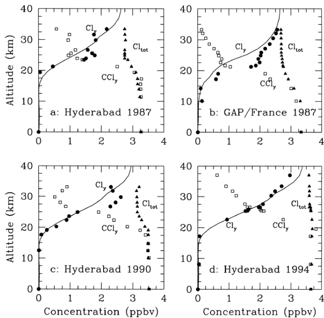
Fig. 6. Vertical distributions of Cl_{total} (filled triangle), CCl_y (open square), Cl_y (filled circle) as calculated using eq. (7). Those calculated using the observations over Hyderabad are for (a) 27 March 1987; (c) 9 April 1990 and (d) 16 April 1994. The distributions estimated using the profiles obtained from GAP, France are shown in (b). Estimated Cl_y from MPIC 2D model derived profiles of HCl, ClONO_2 and ClO_y is shown as continuous line.
