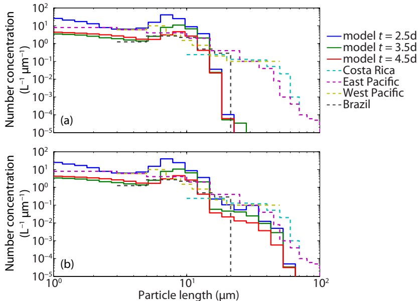
Fig. 9. Ice number size distributions from model at 2.5 d, 3.5 d and 4.5 d, and observations in TTL cirrus over Costa Rica (Davis et al., 2010), East Pacific (Lawson et al., 2008), West Pacific (McFarquhar et al., 2000) and Brazil (Voigt et al., 2007). In the study of Voigt et al. (2007), the instrument was able to detect ice crystals up to about 30 \mu m , but no crystal larger than 22 \mu m was observed. In (a), all ice crystals in the simulated cloud are spheres, as assumed in the bin microphysics and radiation schemes in the model. In (b), 2 % and 1 % of spherical crystals in the model output are replaced respectively by plate-like and columnar crystals.
