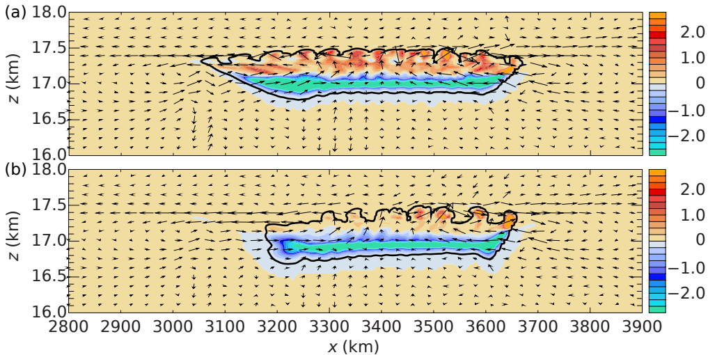
Fig. 15. Instantaneous latent heat release ( 10^{-8} \text{ K s}^{-1} ) at 3.5 d in the all-physics case (a) and in the no-RAV case (b). The thick, black contour marks the cloud boundary, which is defined by the 11^{-1} contour of ice number concentration. Vectors show the radiatively induced velocities.
