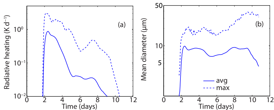
Fig. 7. Same as Fig. 5 but for radiative heating rate (a) and mean diameter of ice crystals (b). Radiative heating rate and mean diameter are shown in logarithmic scale.
