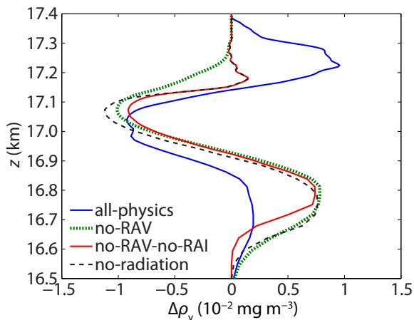
Fig. 14. Differences in the water vapor densities between the final and initial time averaged over the horizontal domain. Results are shown for four simulations: all-physics, no-RAV, no-RAV-no-RAI, and no-radiation.
