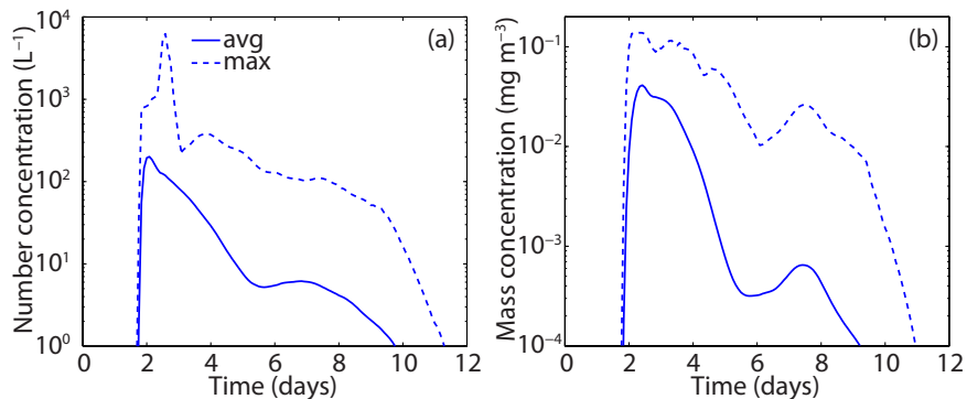
Fig. 6. Same as Fig. 5 but for ice number concentration (a) and IWC (b) . Ice number concentration and IWC are shown in logarithmic scale.
