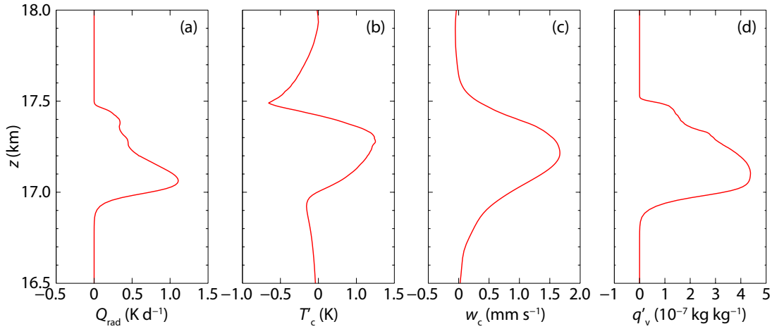
Fig. 12. Horizontal averages between x = 3200 km and 3600 km of the radiative heating rate (a) , its induced temperature perturbations (b) , its induced vertical velocity (c) , and perturbation water vapor mixing ratio (d) at 3.5 d.
