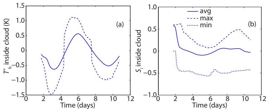
Fig. 5. Time evolution of the maximum and average over the cloudy region of the large-scale temperature perturbations (a) and supersaturation ratio (b) . In (b) the minimum over the cloudy region of the supersaturation ratio is also shown.
