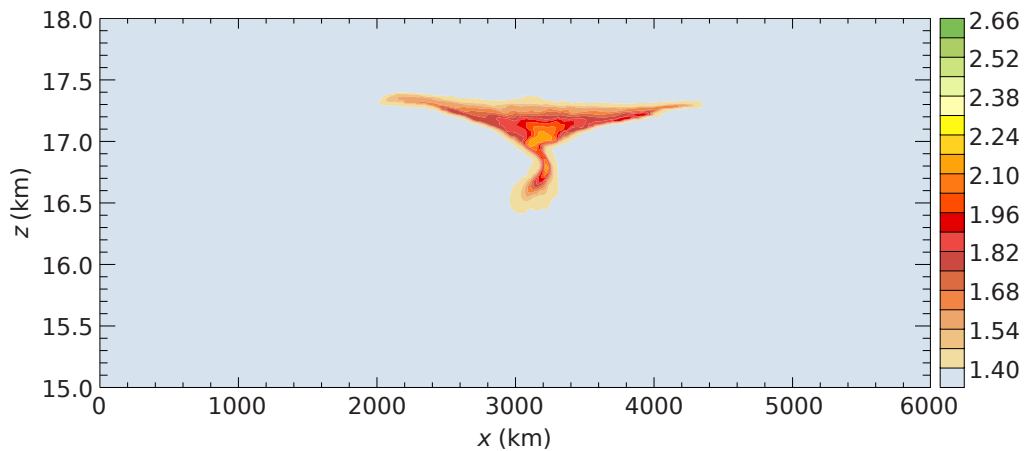
Fig. 13. Water vapor mixing ratio ( 10^{-6} \text{ kg kg}^{-1} ) at the final time in the control simulation.
