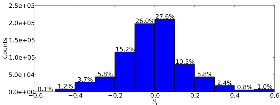
Fig. 8. Frequency distribution of the supersaturation ratio ( S_i ) over the cloudy grid points and all model's output times.
