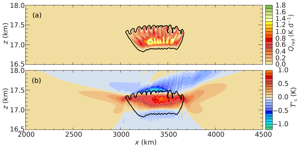
Fig. 10. The radiative heating (a) and induced temperature perturbations (b) at 3.5 d. The black outline in each figure marks the radiative heating rate contour of 0.01 \text{ K d}^{-1} . Note the ratio of horizontal to vertical scales is 10^4 to 6.
