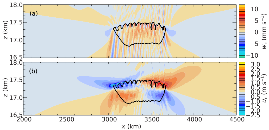
Fig. 11. Same as Fig. 10 but for the radiatively induced vertical velocity (a) and horizontal velocity (b).
