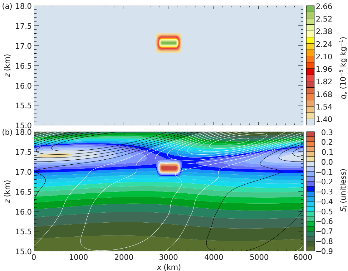
Fig. 4. Water vapor mixing ratio (a) and supersaturation ratio (b) at the initial time. In (b) , the black and white contours respectively show negative and positive large-scale wave temperature perturbations.
