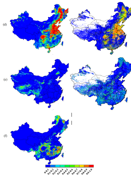
Fig. 1 The coverage fraction of each vegetation type for MODIS (left) based on 12 km x 12 km grid and MEGAN (right) based on 1 km x 1 km grid. (a) Broadleaf forest; (b) Coniferous forest; (c) Crop; (d) Grass; (e) Shrub; (f) Mixed forest.
