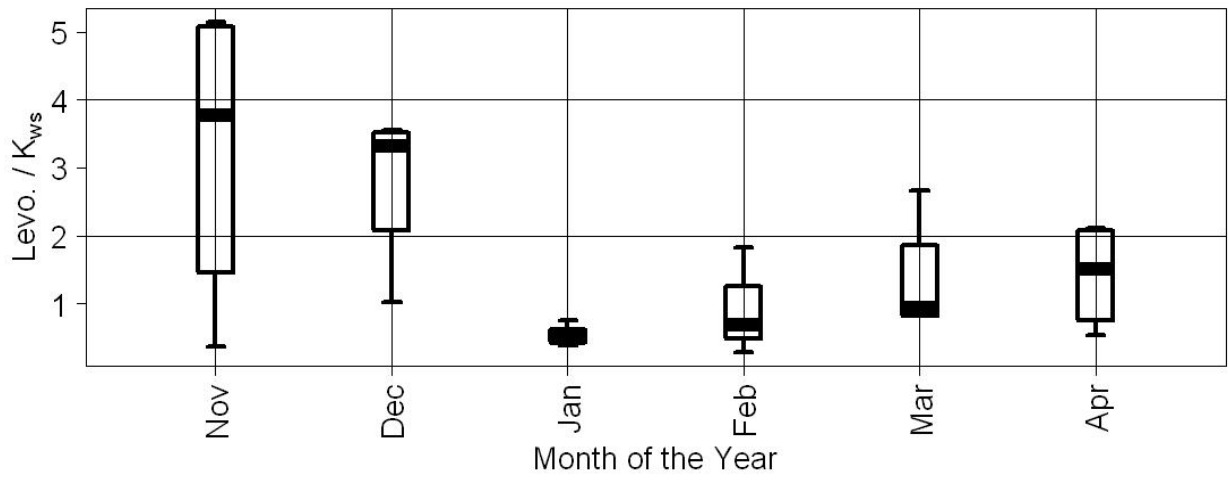
Figure 4: Ratio of levoglucosan: K_{ws} at Budbrooke according to month of observation
