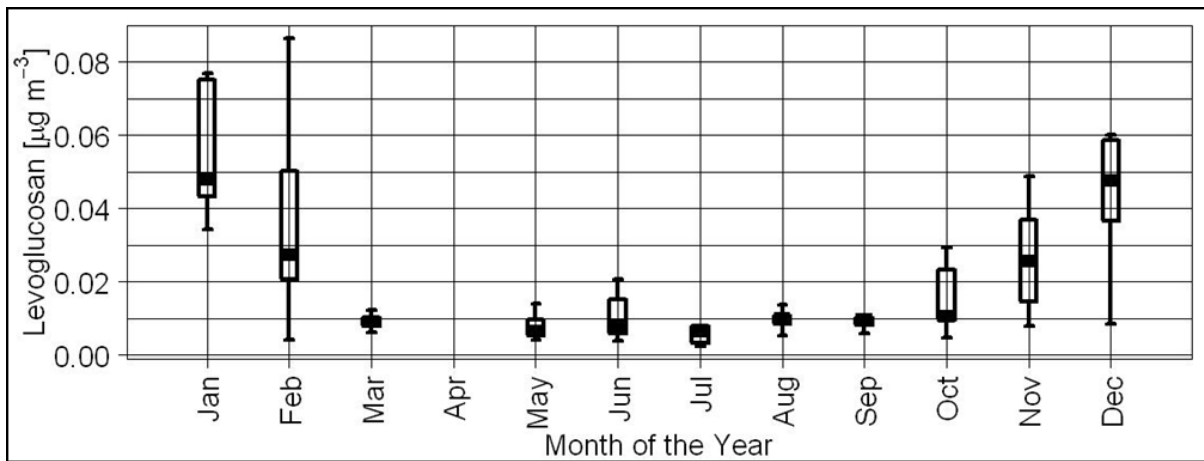
Figure 1: Monthly variation of levoglucosan concentrations measured at EROS between 23/06/2008 and 31/03/2010
