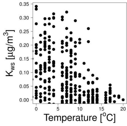
Figure 5: Variation of K_{ws} with temperature at EROS site
