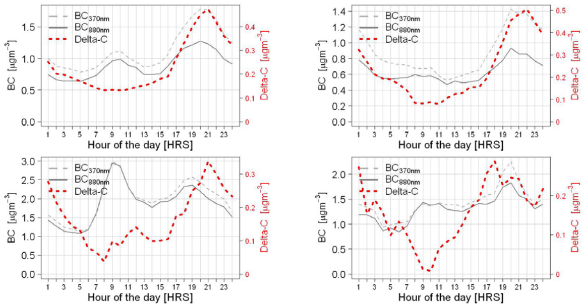
Figure 6: Average diurnal variation in black carbon estimated at 370 and 880 nm with the aethalometer and Delta-C at Budbrooke (top panel) and North Kensington, winter (bottom panel). Left plot: weekday; right plot: weekend.
