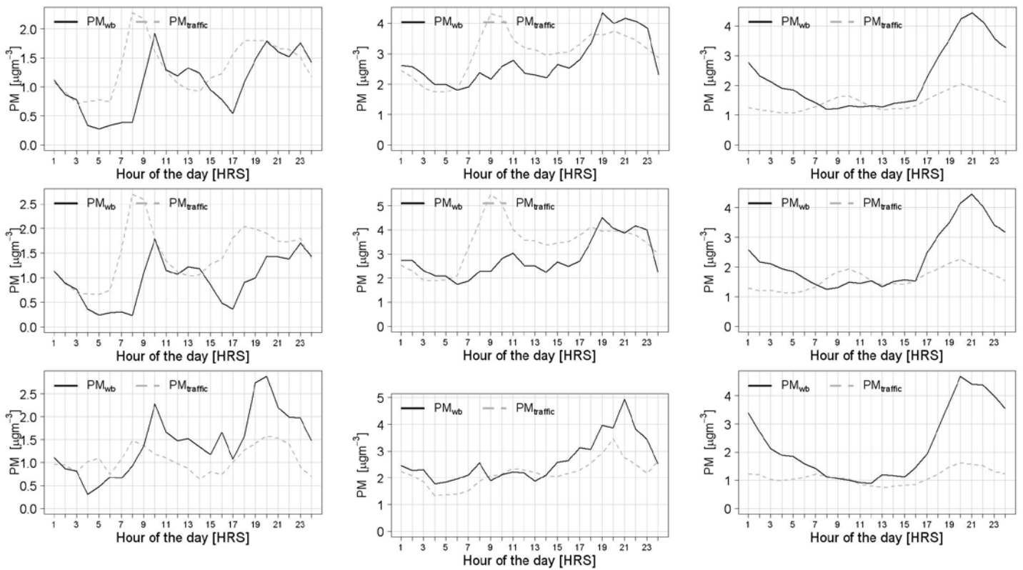
Figure 3: Diurnal variation of PM_{wb} and PM_{traf} measured at EROS (04/05/2009-31/03/2010) (left panel), North Kensington (16/02/2011)-15/03/2011) (middle panel) and Budbrooke (20/11/2009-08/04/2010) (right panel). (Top panel plot: average of all days; middle plot: average weekday; bottom panel plots: average week end day)
