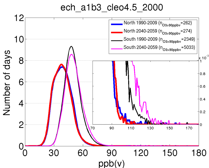
Fig. 1. Frequency distributions of daily max O 3 concentrations in North and South Europe in the climate sensitivity simulation with meteorological data downscaled from the ECHAM5 global model.
