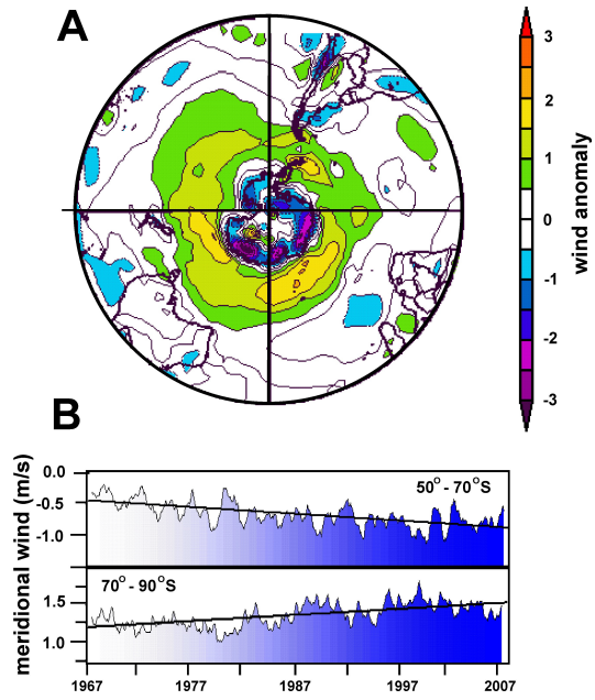
Fig. 2 - (A) wind anomaly (after 1979 minus before 1979); (B) meridional wind from NCEP-NCAR Reanalysis in 2 latitudinal C4522
