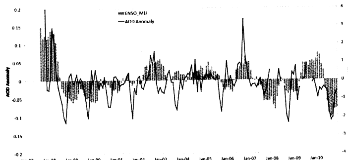
Fig. 4. Time series of AOD anomaly and ENSO Index over Indonesia region ( 8^{\circ}\text{S} – 8^{\circ}\text{N} , 90^{\circ}\text{E} – 130^{\circ}\text{E} ).
