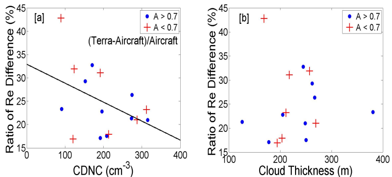
Figure R2 the percentage differences between Terra-MODIS retrievals and aircraft measurements of cloud effective radius as a function of cloud drop number concentration and cloud geometric thickness
